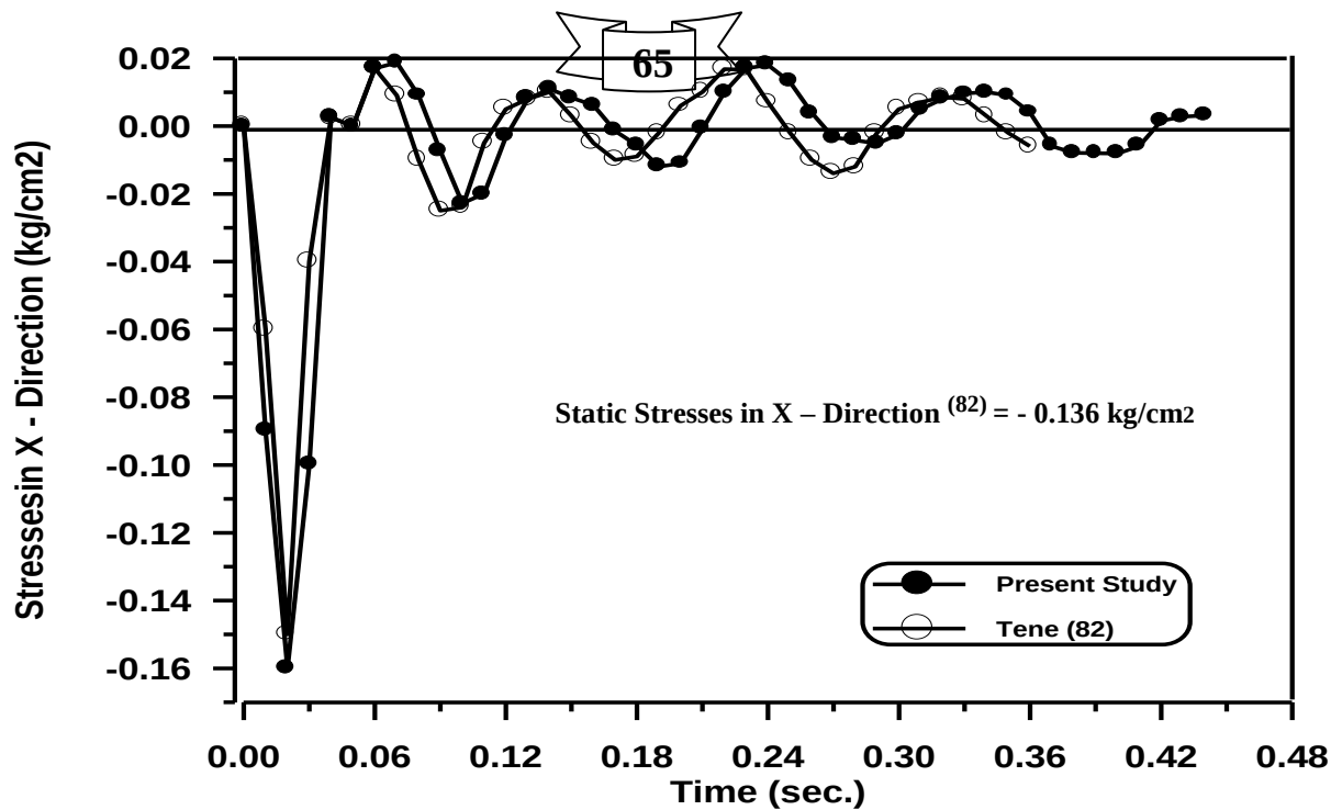
Figure (5-10) Time – Stresses in X – Direction Response of the Circular Arch Without Damping at Gauss Point (3).
