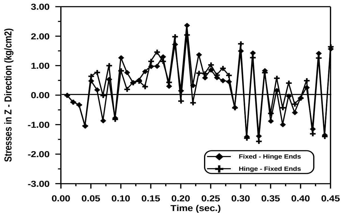
Figure (5-80) Time – Stresses in Z - Direction Response at Gauss Point (25 or 26) With Various Boundary Condition.
