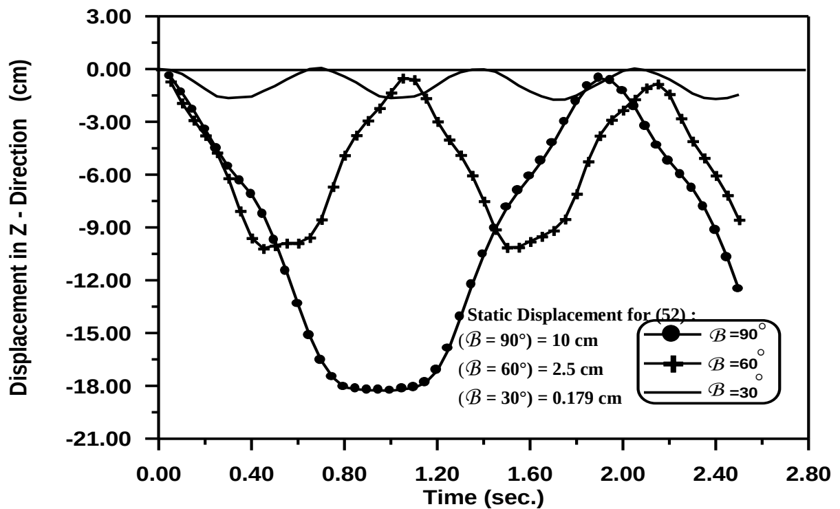
Figure (5-19) Time – Displacement in Z - Direction Response at Free End for Curved Cantilever with Three Subtended Angles.
