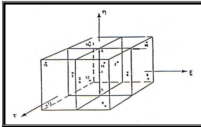
Figure (4.4) Three - Dimensional Concrete Element with 20 nodes (44) .
