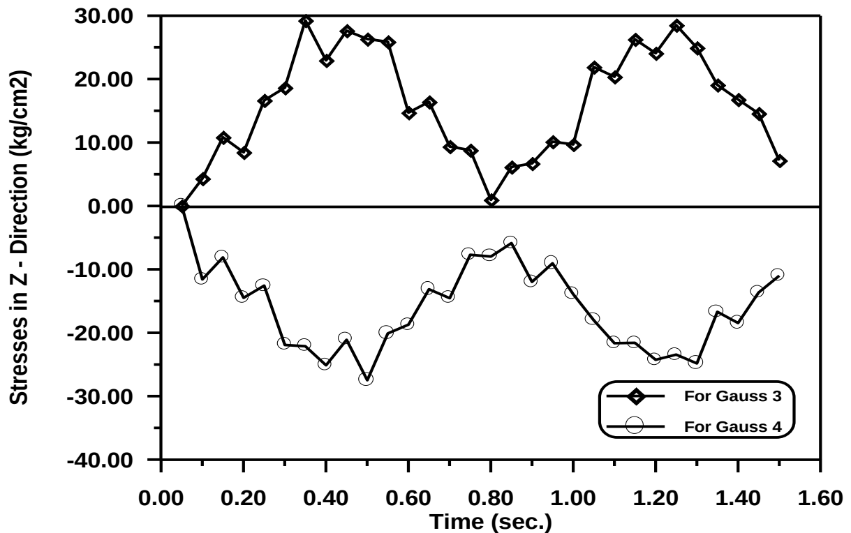
Figure (5-59) Time – Stresses in Z - Direction Response of Arch at Gauss Point (3) and (4) for Number of Elements = 9.
