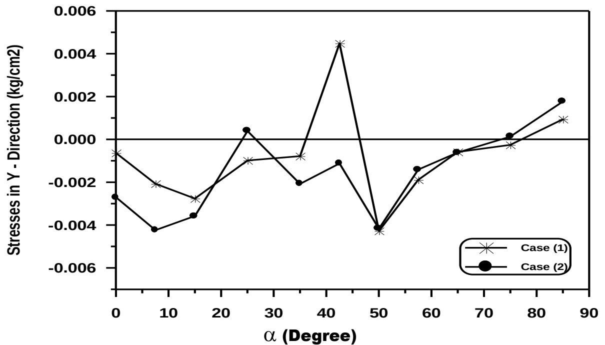
Figure (5-44) The Stresses in Y - Direction Along the Arch at (t=0.0025 sec.).
