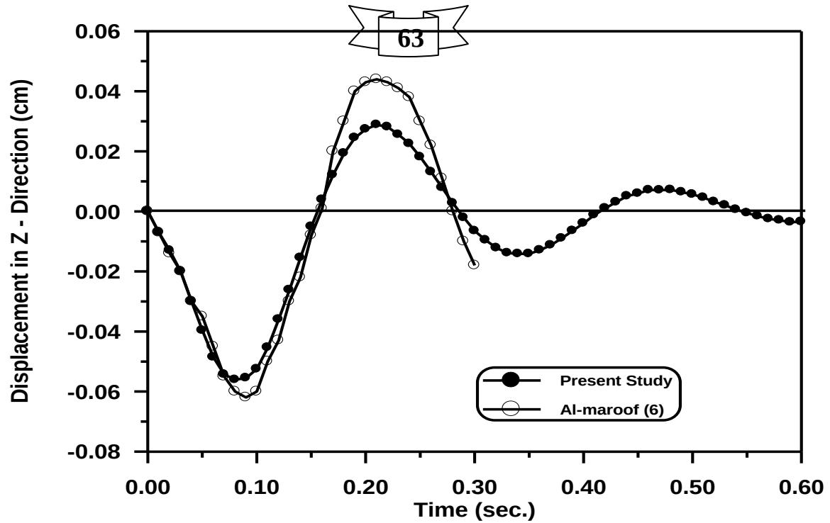
Figure (5-6) Time – Displacement in Z - Direction Response for Dynamic Response of the Circular Arch With Damping at ( \alpha = 90^\circ ).
