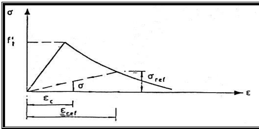
Figure (3.9) Strain – Softening Curve with Secant Unloading and Re – Loading (44) .
