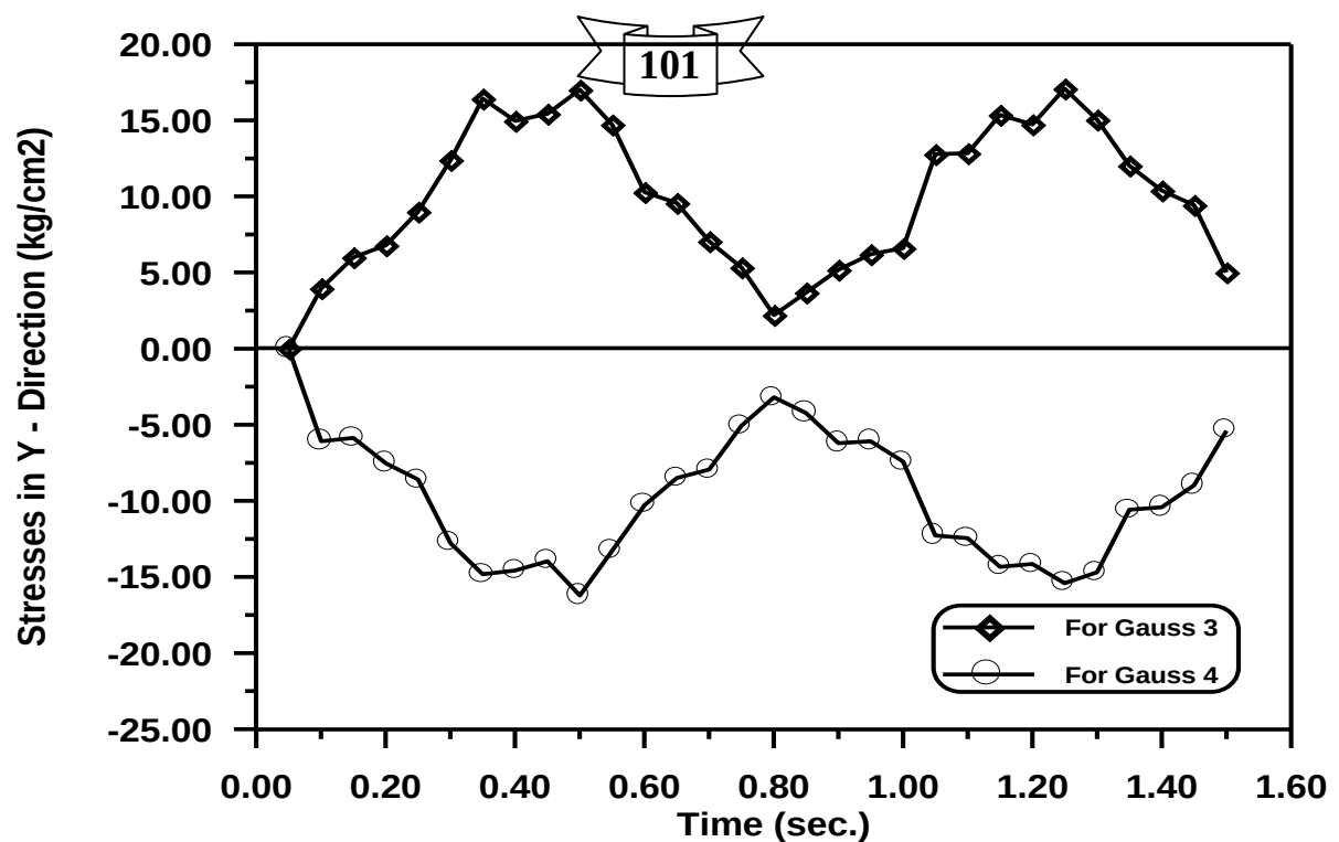
Figure (5-60) Time – Stresses in Y - Direction Response of Arch
