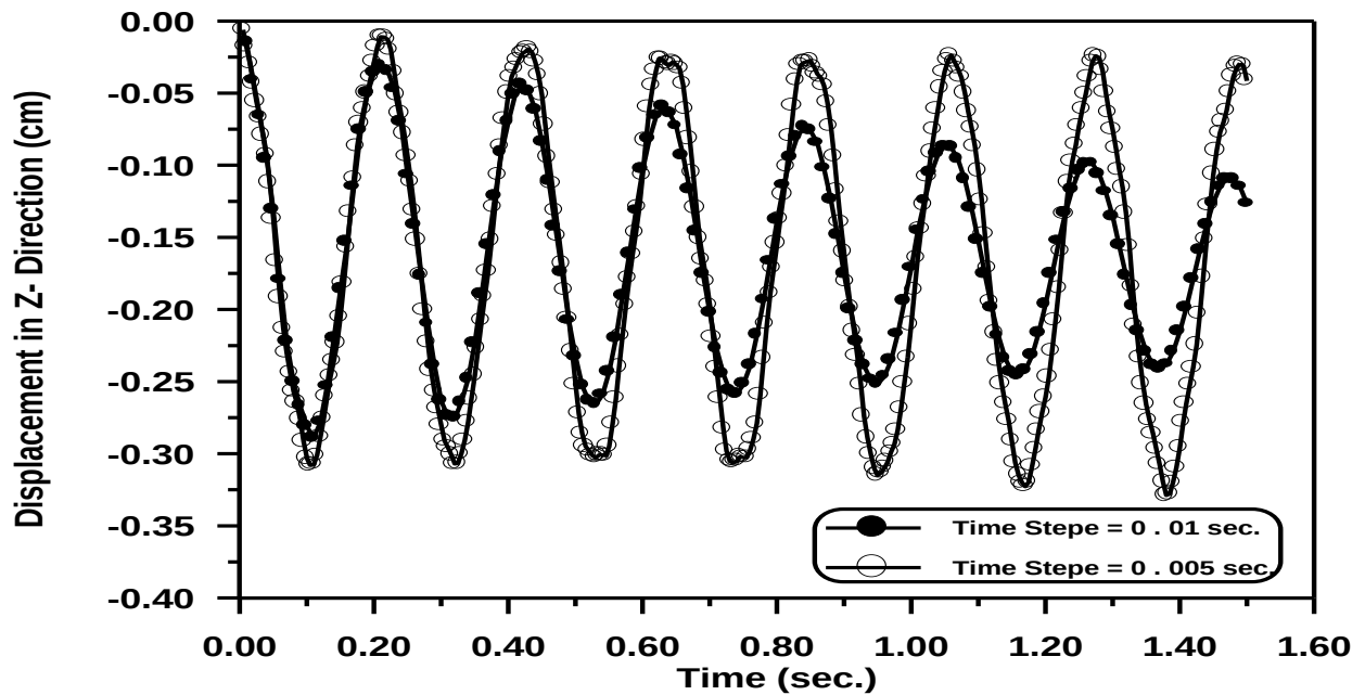
Figure (5-91) Effect the Time Step on Time – Displacement in Z - Direction Response at Center of Arch .
