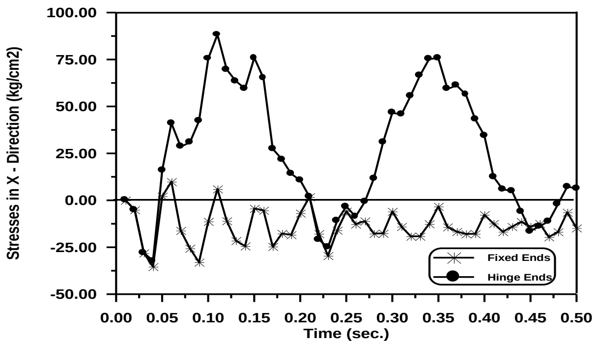
Figure (5 -82) Time – Stresses in X - Direction Response at Gauss Point (27) With Various Boundary Conditions.
