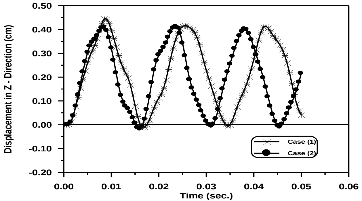
Figure (5-31) Time – Displacement in Z - Direction Response Of the Center of Circular Arch.
