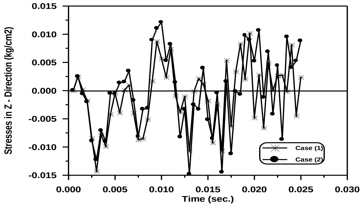
Figure (5-40) Time – Stresses in Z - Direction Response of The Circular Arch at Gauss Point (2).
