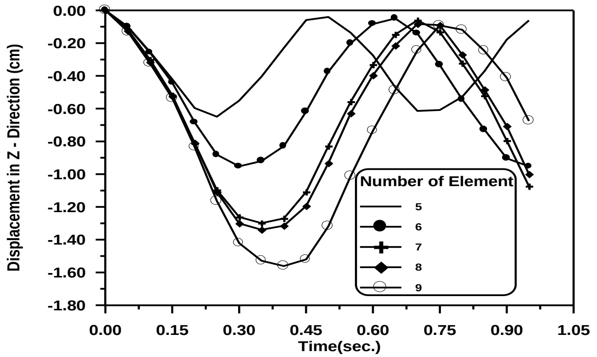
Figure (5-48) Effect the Number of Elements on Time – Displacement in Z - Direction Response at Center of Arch.
