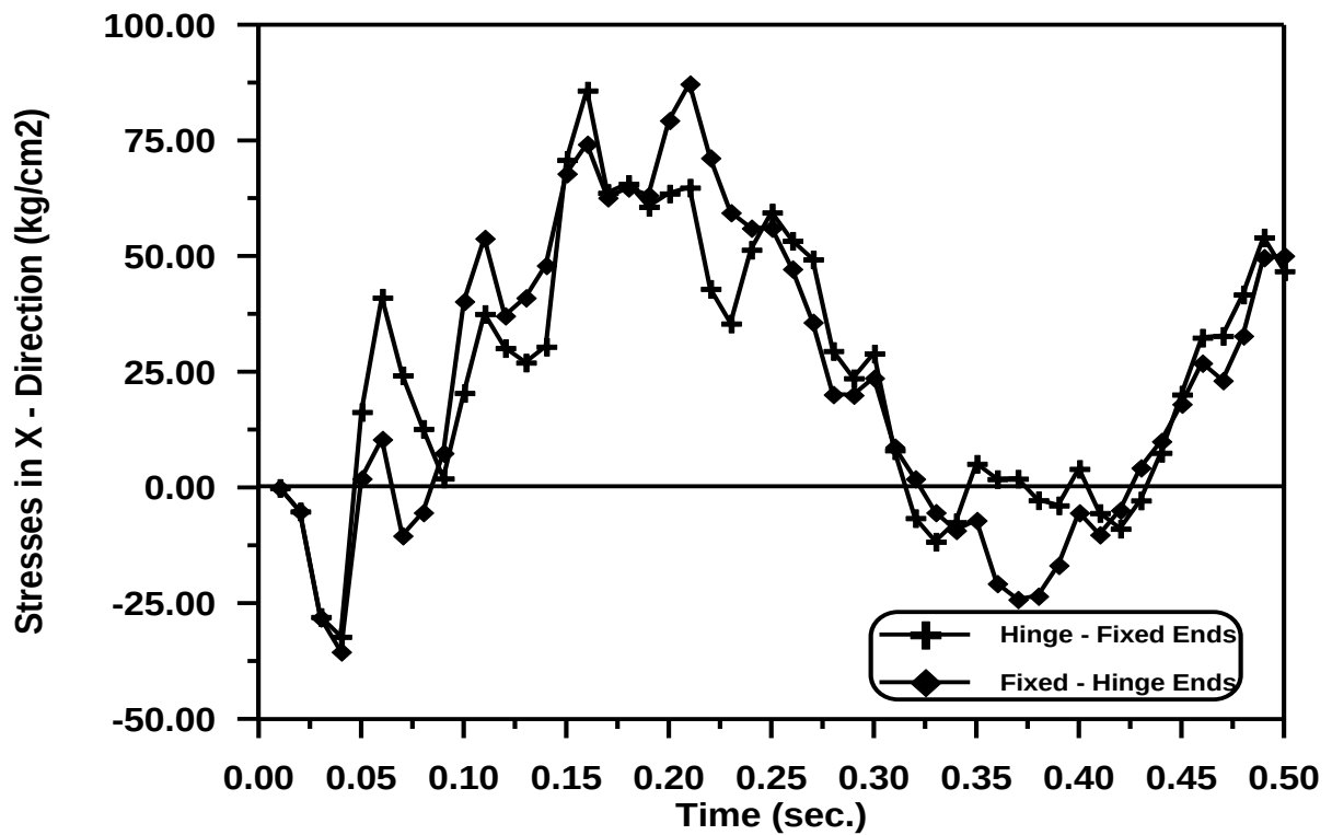
Figure (5-81) Time – Stresses in X - Direction Response at Gauss Point (27) With Various Boundary Conditions .
