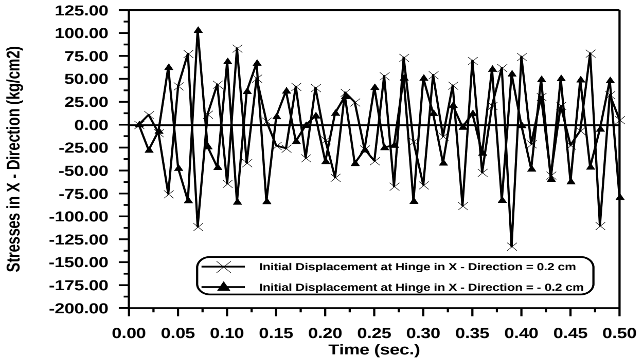
Figure (5-96) Effect the Initial Displacement on Time – Stresses Response at Gauss Point (6) .
