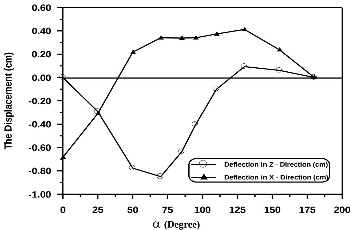
Figure (5-73) The Displacement Along the Arch Under Dynamic Load with Fixed – Hinge Ends at ( t=0.35\text{sec.} ).
