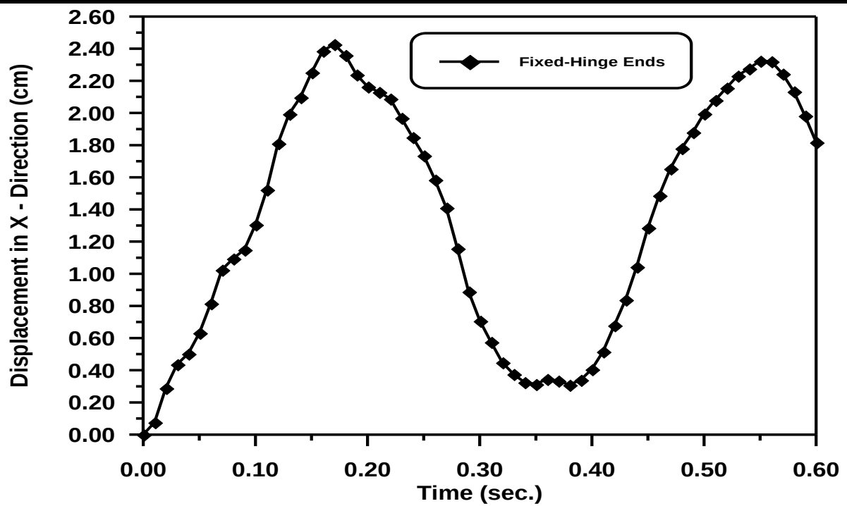
Figure (5-69) Time – Displacement in X - Direction Response at ( \alpha=50^\circ ) with Various Boundary Condition.
