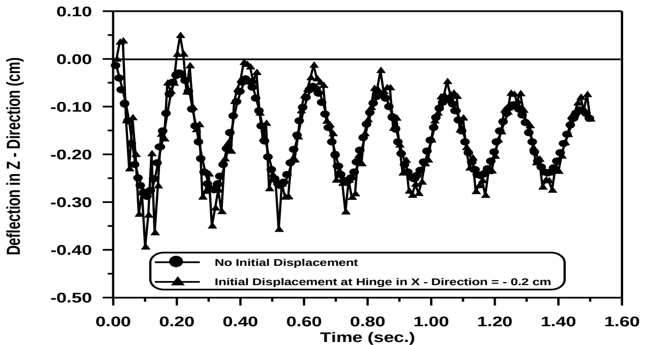
Figure (5-93) Effect the Initial Displacement opposite X – Direction on Time – Displacement in Z - Direction Response at Center of Arch .
