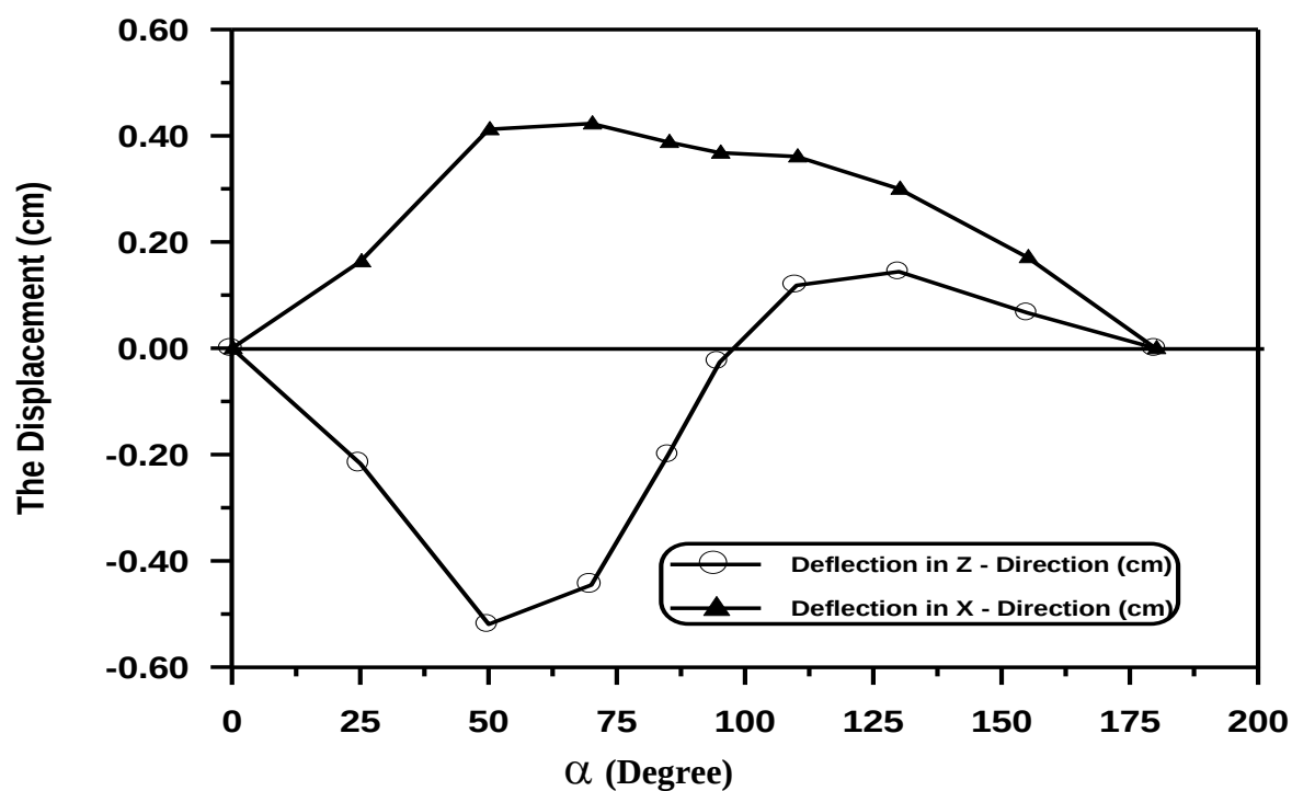
Figure (5-72) The Displacement Along the Arch Under Dynamic Load with Fixed – Fixed Ends at (t=0.35 sec.).
