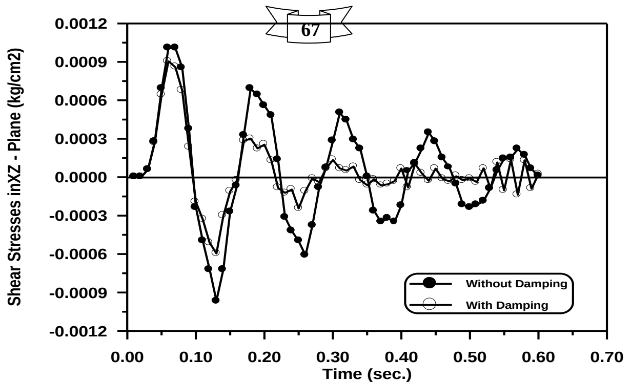
Figure (5-14) Time –Shear Stresses in XZ - Plane Response of the Circular Arch at Gauss Point (63).
