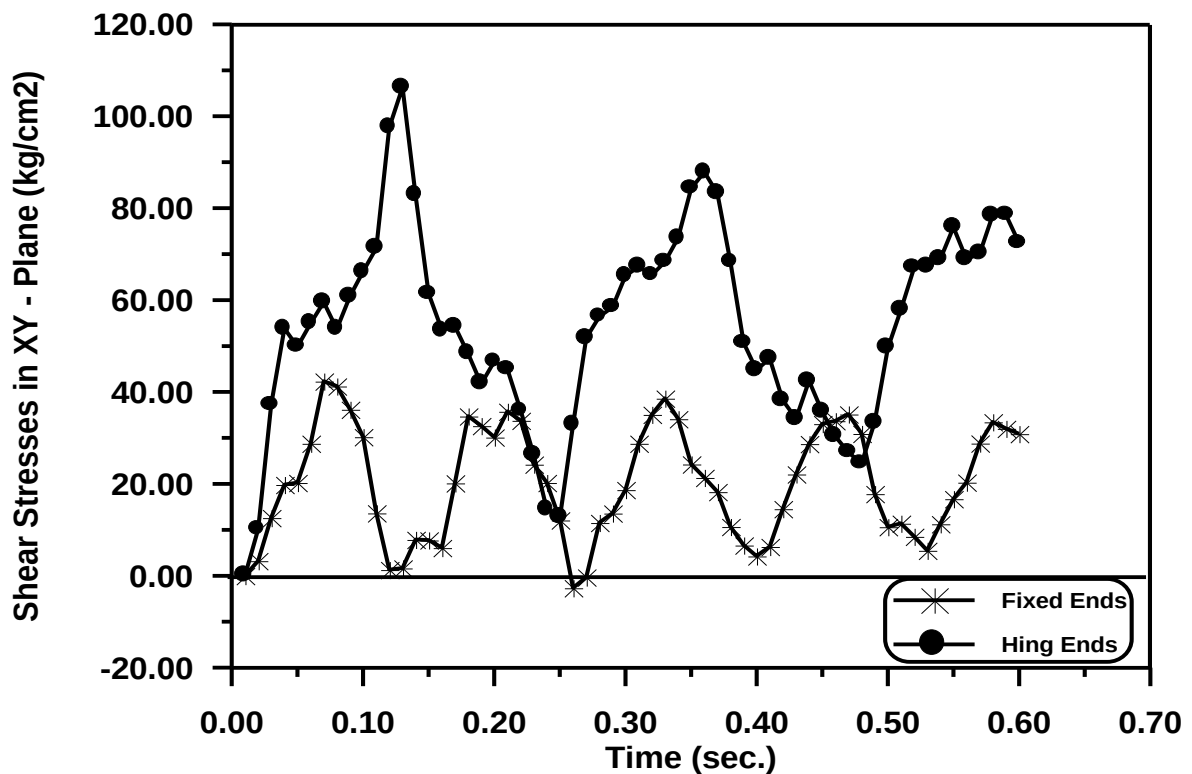
Figure (5-86) Time – Shear Stresses in XY - Plane Response at Gauss Point (6) with Various Boundary Conditions.
