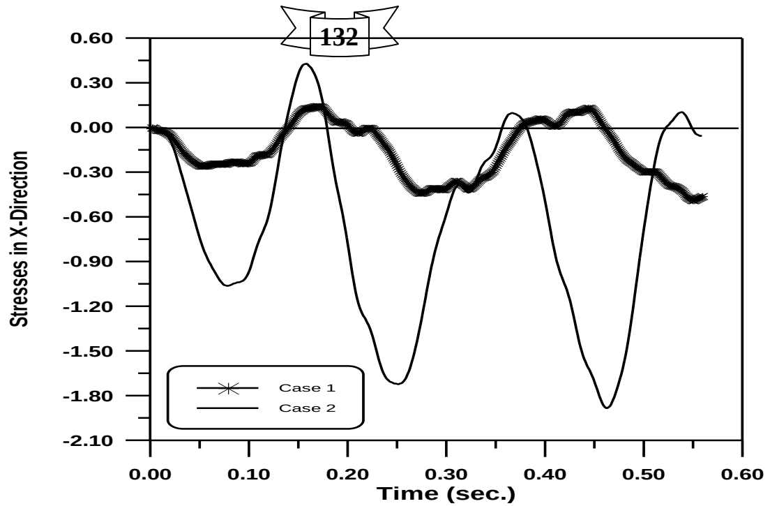
Figure(5-103) Time – Stresses in X – Direction Response at Gauss Point (6) of Center Circular Arch
