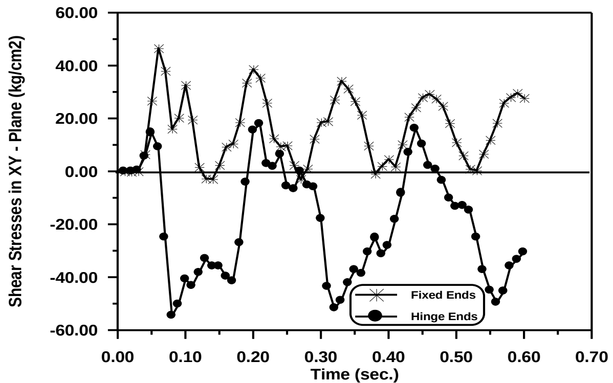
Figure (5-88) Time – Shear Stresses in XY - Plane Response at Gauss Point (53) with Various Boundary Conditions.
