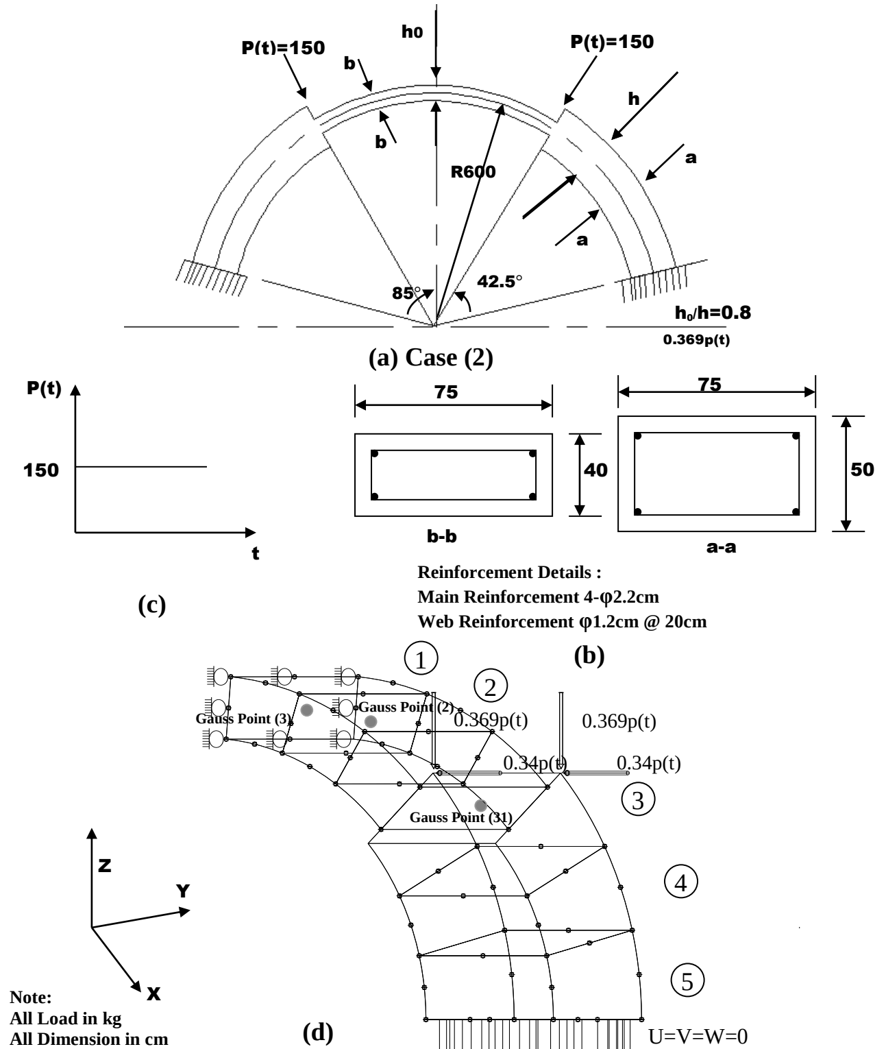
(a) geometry and loading of arch (b) cross section (c) load – time relation (d) finite element idealization and numbering of half of the arch
