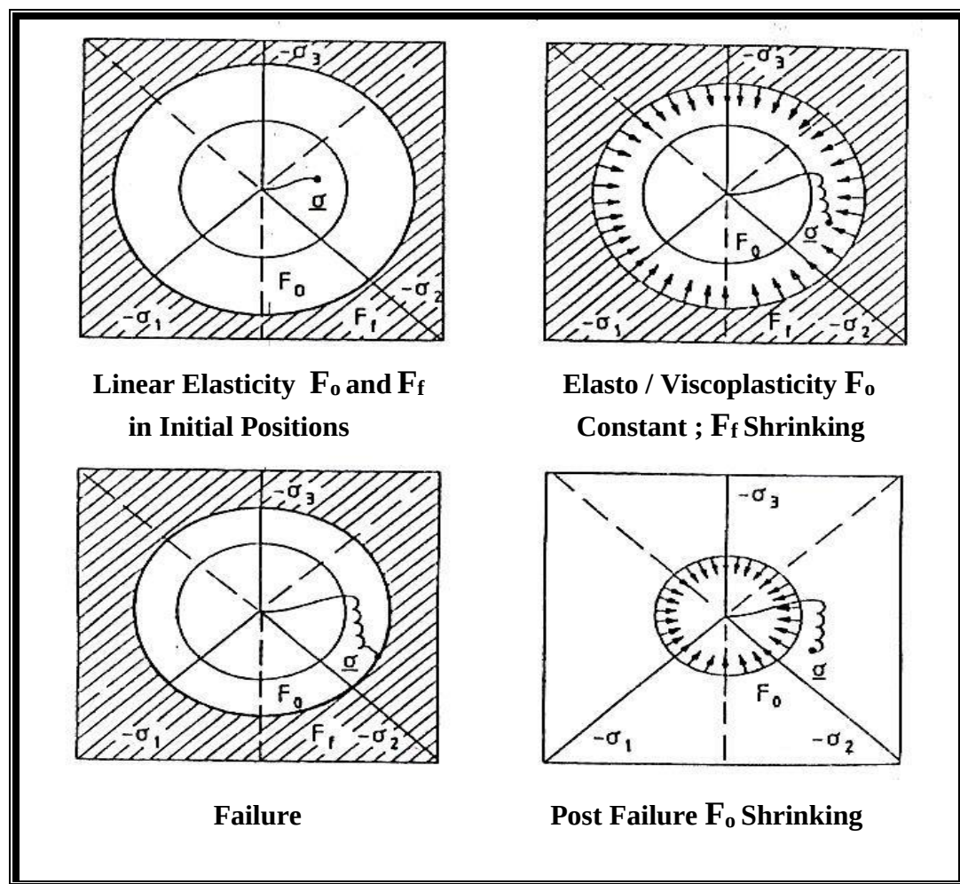
Figure (3.3) Evaluation of the Yield and Failure Surfaces (44) .
