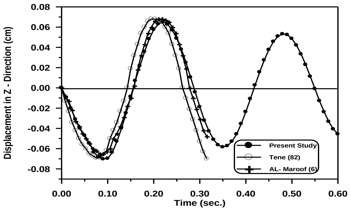
Figure (5-4) Time – Displacement in Z - Direction Response for Dynamic Response of the Circular Arch at ( \alpha = 90^\circ ).
