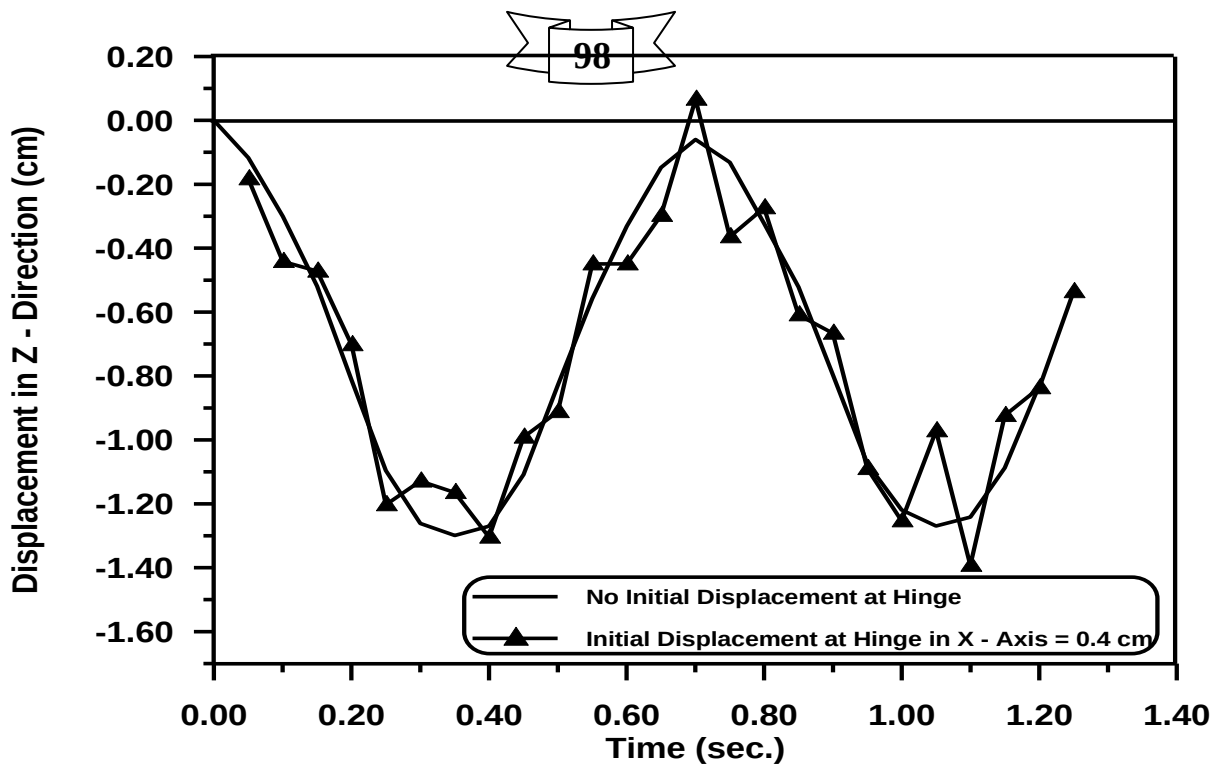
Figure (5-54) Effect Initial Displacement at Hinge on Time –Displacement in Z - Direction Response at Center of Arch for Number of Element = 7.
