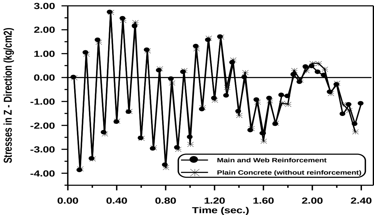
Figure (5-63) Time – Stresses in Z - Direction Response of Arch at Gauss Point (1) or (2) for Number of Elements = 9.
