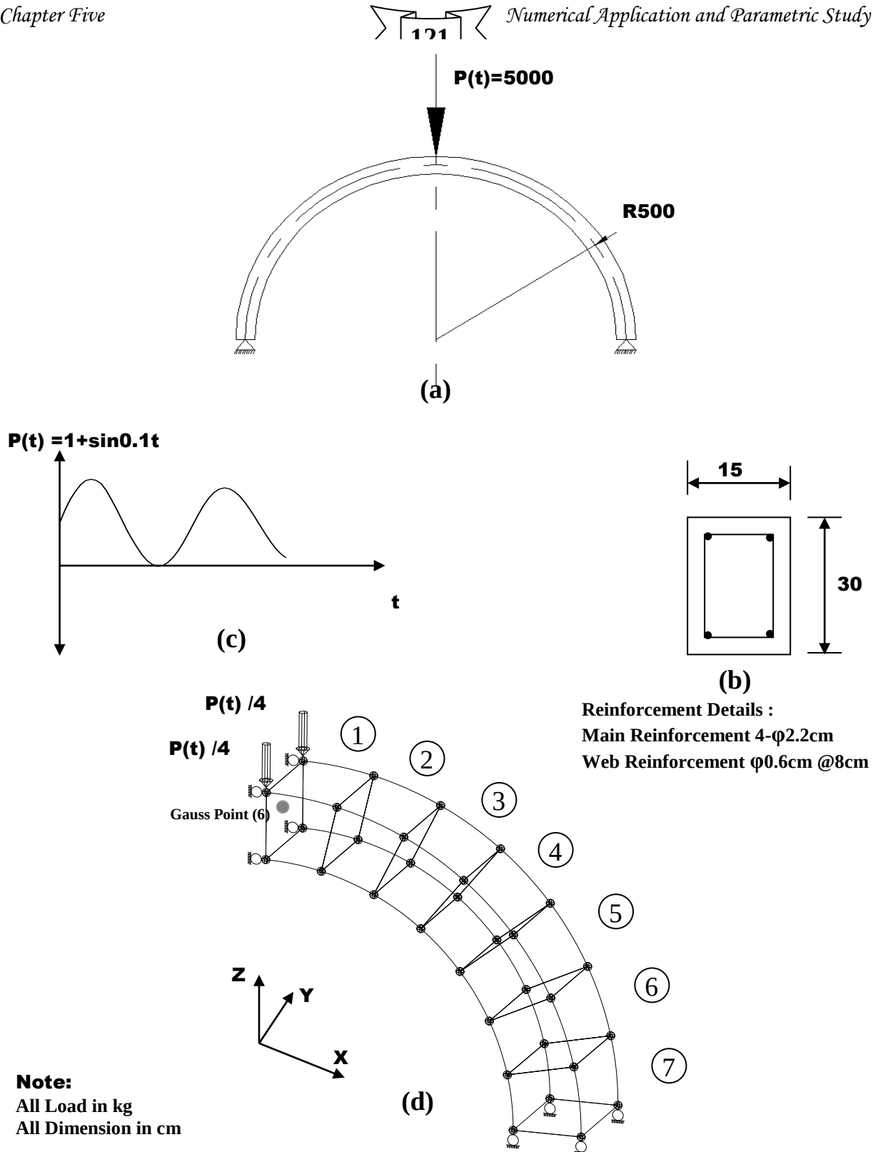
(a) geometry and loading of arch (b) cross section (c) load – time relation (d) finite element idealization and numbering of half of the arch
