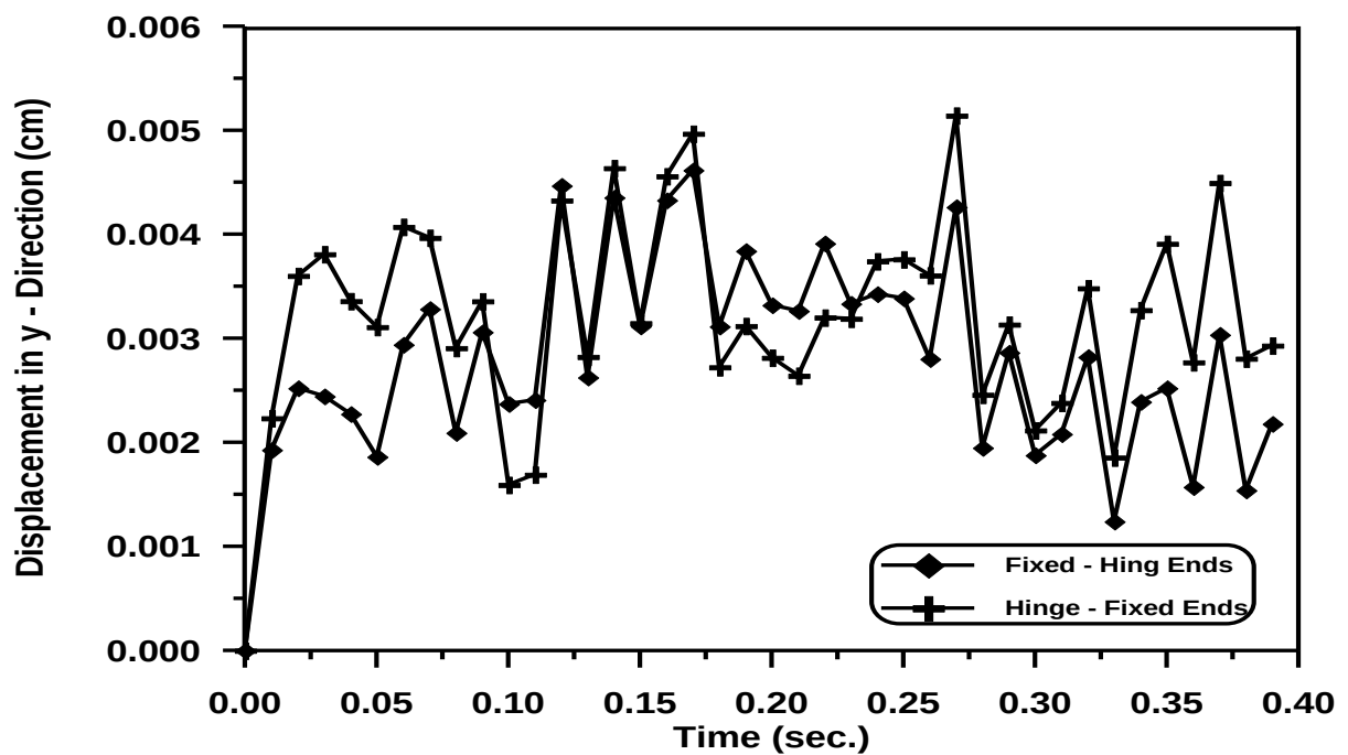
Figure (5-68) Time – Displacement in Y - Direction Response at ( \alpha=50^\circ ) with Various Boundary Condition.
