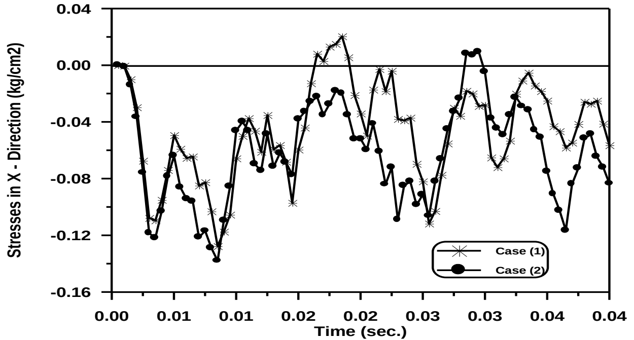
Figure (5-39) Time – Stresses in X - Direction Response of The Circular Arch at Gauss Point (2).
