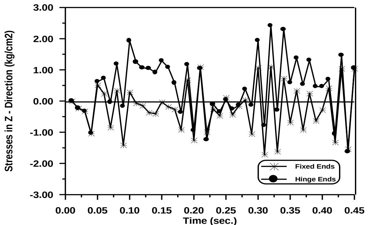
Figure (5-76) Time – Stresses in Z - Direction Response at Gauss Point (25 or 26) With Various Boundary Condition.
