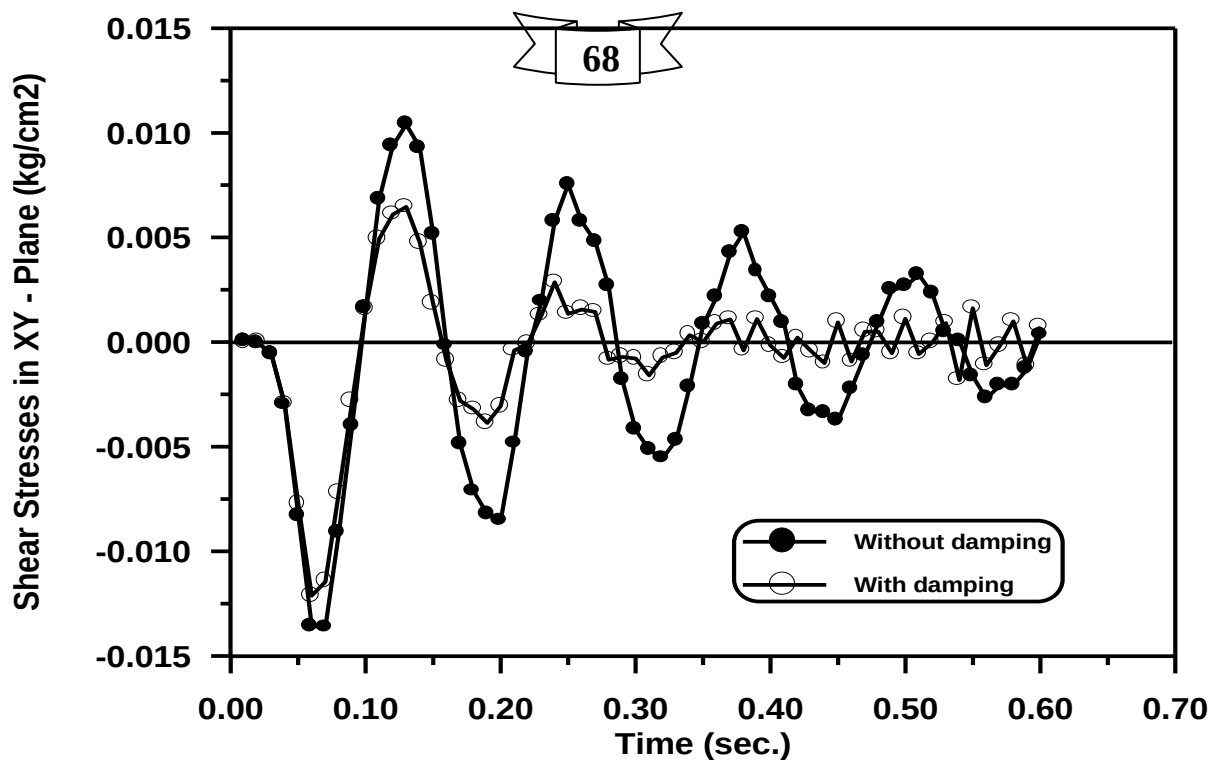
Figure (5-16) Time –Shear Stresses in XY – Plane Response of the Circular Arch at Gauss Point (63).
