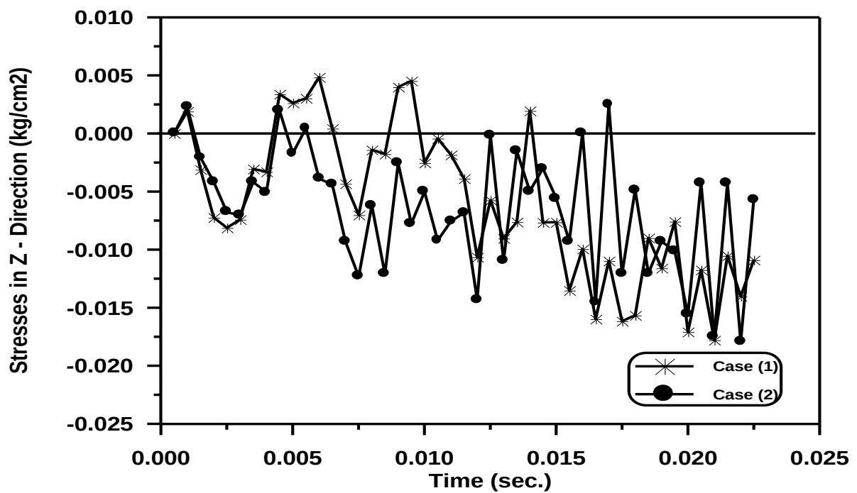
Figure (5-36) Time – Stresses in Z - Direction Response
