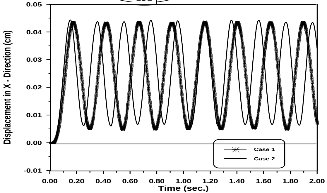
Figure(5-101) Time – Displacement in X – Direction Response of the Circular Arch at ( \alpha=45^\circ )
