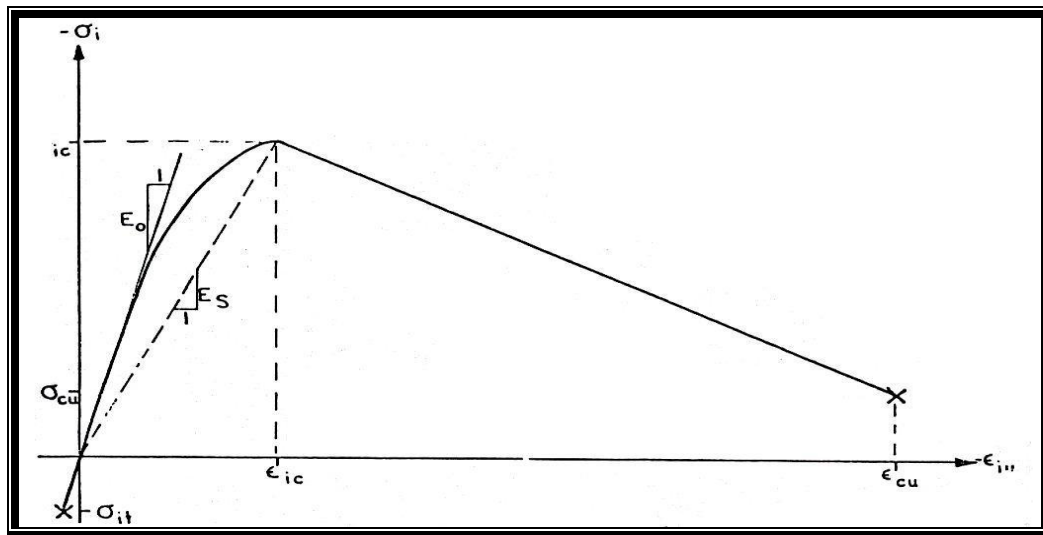
Figure (3.2) Equivalent Uniaxial Stresses – Strain Curve of Concrete (3) .
