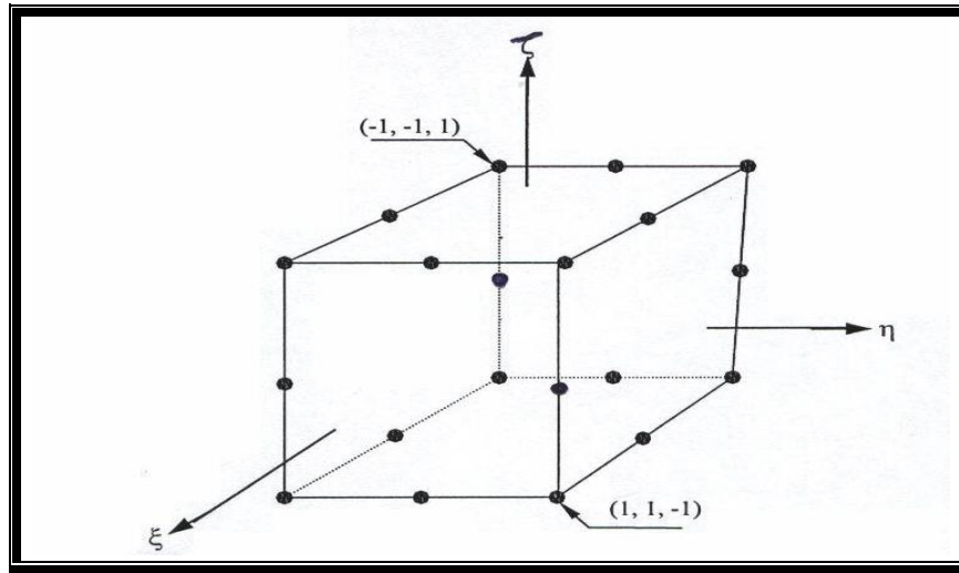
Figure (4.2) Non – Dimensional Co – ordinate Element ( \xi, \eta, \tau ) (15) .
