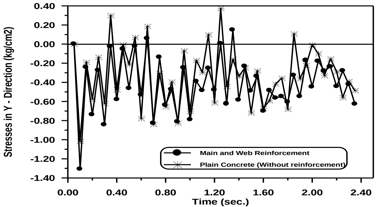
Figure (5-61) Time – Stresses in Y - Direction Response of Arch at Gauss Point (1) or (2) for Number of Elements = 9.
