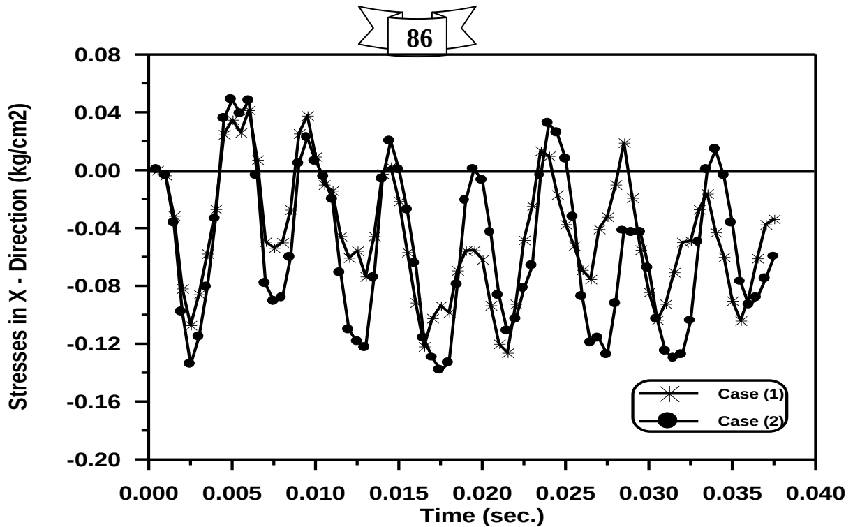
Figure (5-35) Time – Stresses in x - Direction Response of The Circular Arch at Gauss point (3).
