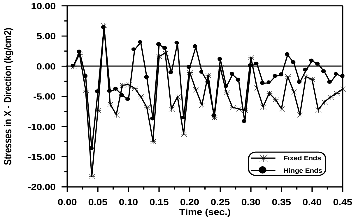
Figure (5-75) Time – Stresses in X - Direction Response at Gauss Point (25 or 26) With Various Boundary Condition.
