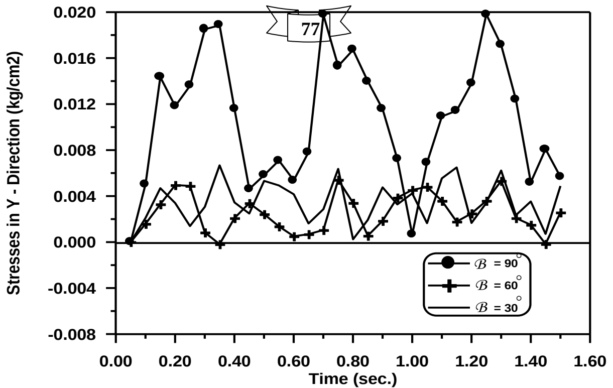
Figure (5-26) Time – Stresses in Y - Direction Response at Gauss
