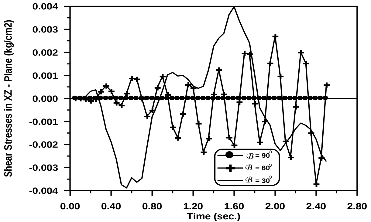
Figure (5-27) Time – Shear Stresses in XZ – Plane Response at Gauss Chapter Five Point (30) For Curved Cantilever with Three Subtended Angles. Numerical Application and Parametric Study
