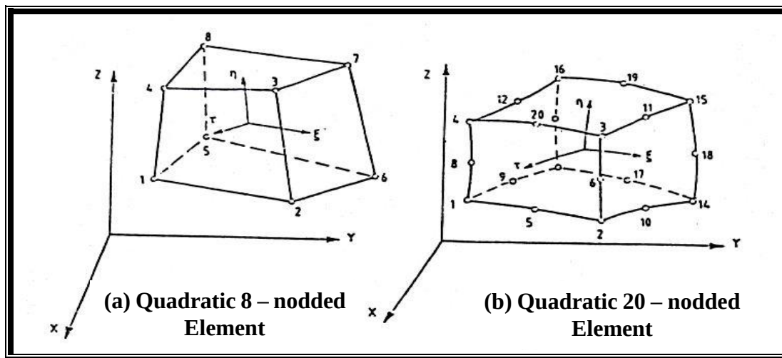
Figure (4.1) Linear and Quadratic Isoparametric Solid Element (3) .
