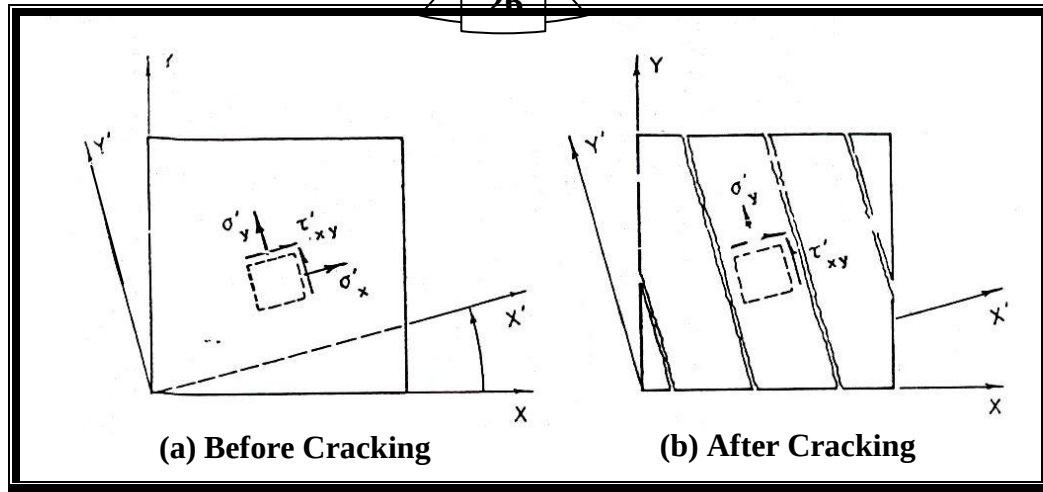
Figure (3.5) Smeared Crack Stresses Distribution (3) .
