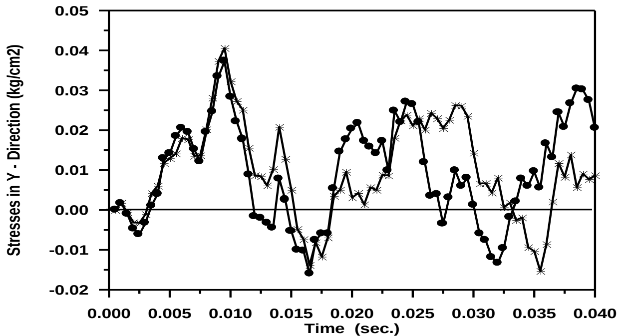
Figure (5-38) Time – Stresses in Y - Direction Response of The Circular Arch at Gauss Point (2).
