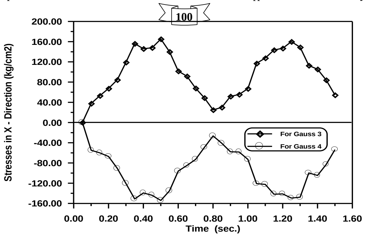
Figure (5-58) Time – Stresses in X – Direction Response of Arch at Gauss Point (3) and (4) for Number of Elements = 9.
