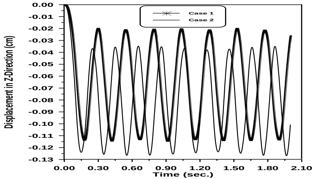
Figure(5-99) Time – Displacement in Z – Direction Response of The Center Circular Arch
