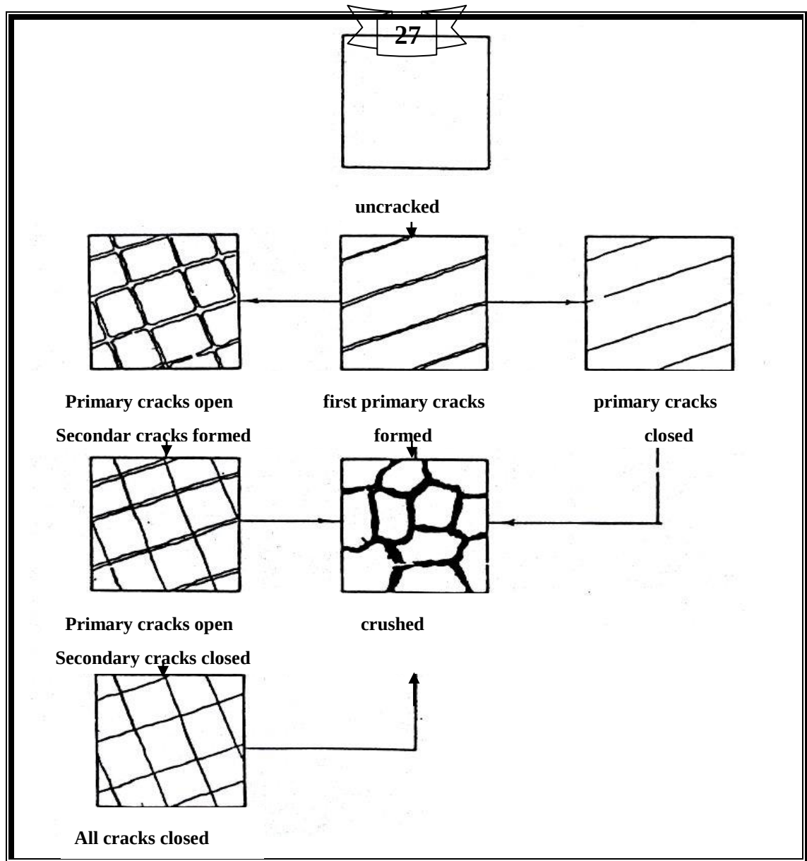
Figure (3.6) Possible Crack Formations in Post – Cracking Level (23) .
