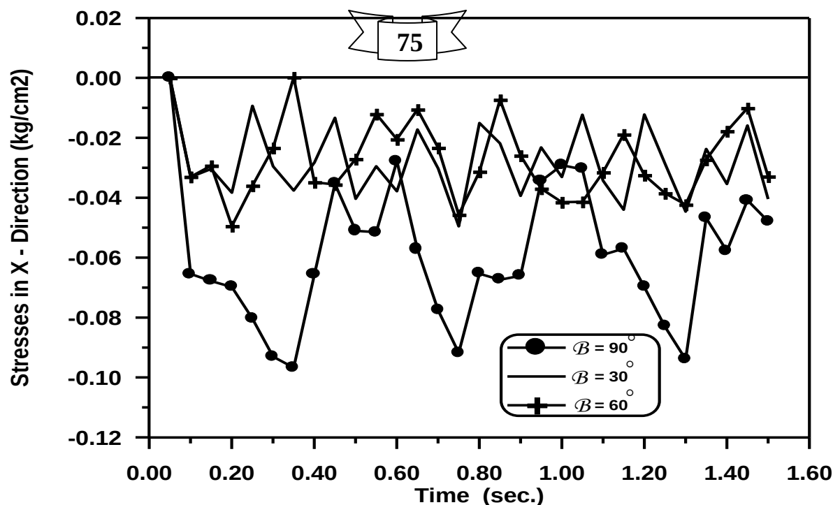
Figure (5-22) Time – Stresses in X - Direction Response at Gauss Point (6) for Curved Cantilever with Three Subtended Angles.
