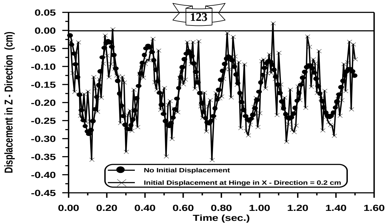
Figure (5-92) Effect the Initial Displacement in X - Direction on Time – Displacement in Z - Direction Response at Center of Arch .
