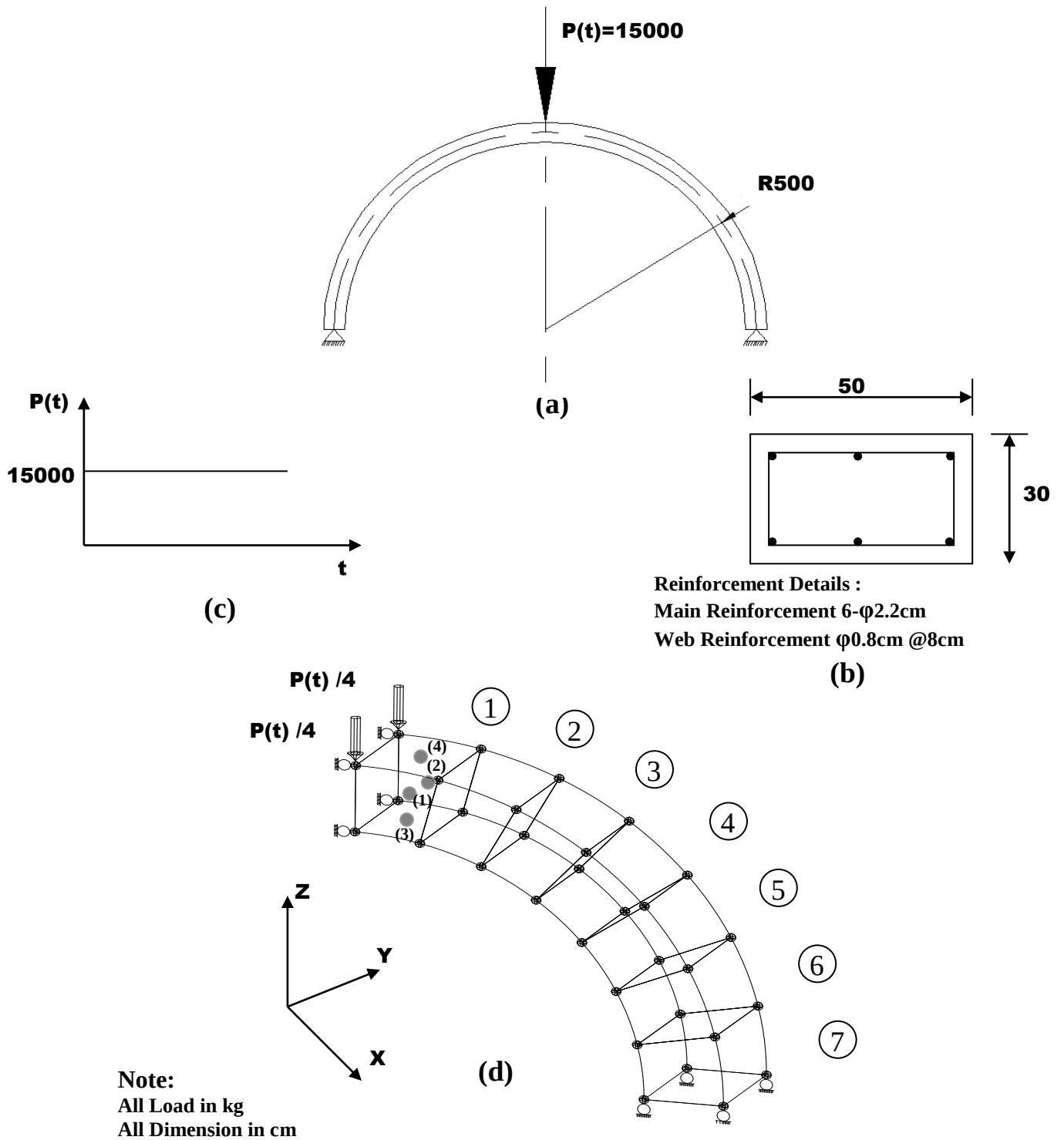
(a) geometry and loading of arch (b) cross section (c) load – time relation (d) finite element idealization and numbering of half of the arch
