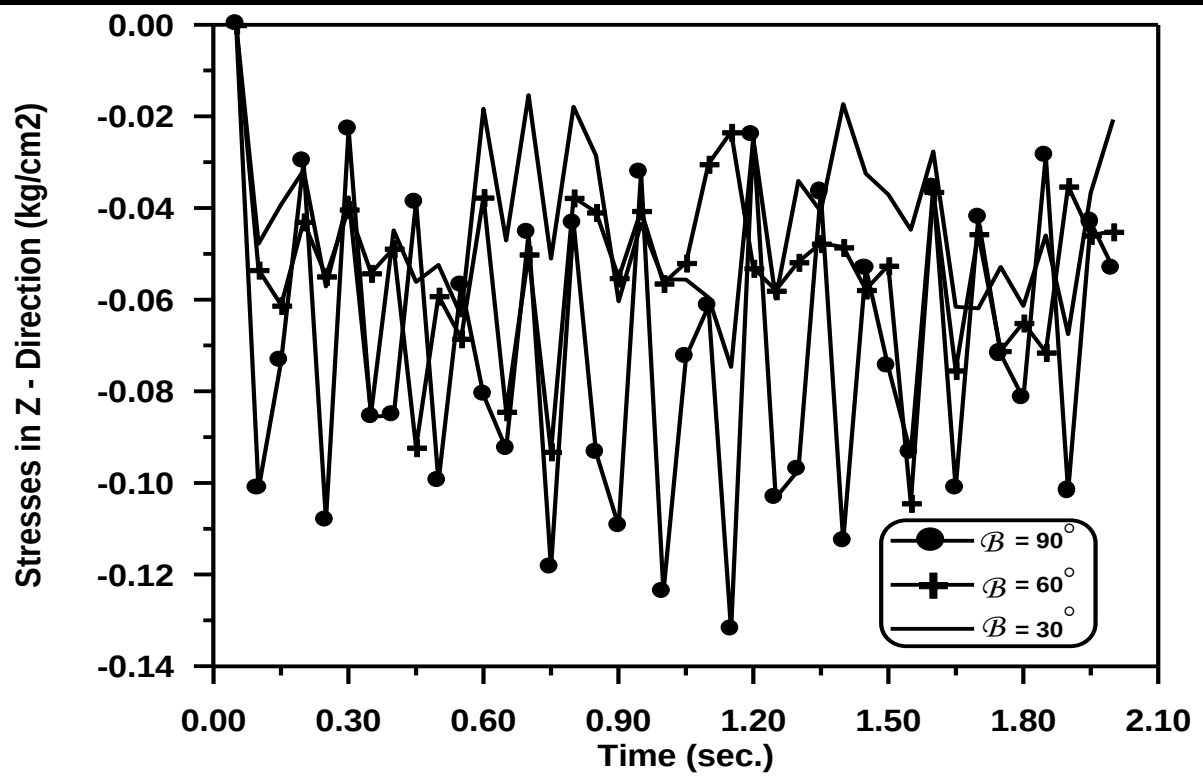
Figure (5-25) Time – Stresses in Z - Direction Response at Gauss Point (5) For Curved Cantilever with Three Subtended Angles. Chapter Five Numerical Application and Parametric Study
