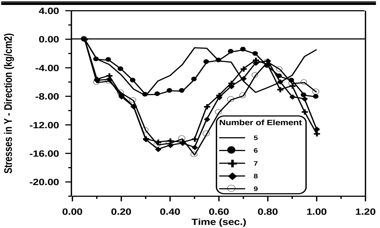
Figure (5-57) Effect the Number of Elements on Time – Stresses In Y – Direction Response of Arch at Gauss Point (4).
