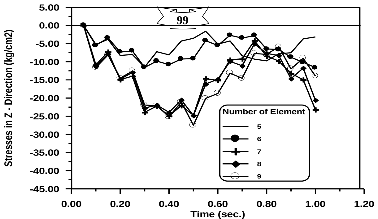
Figure (5-56) Effect the Number of Elements on Time – Stresses In Z - Direction Response of Arch at Gauss Point (4).
