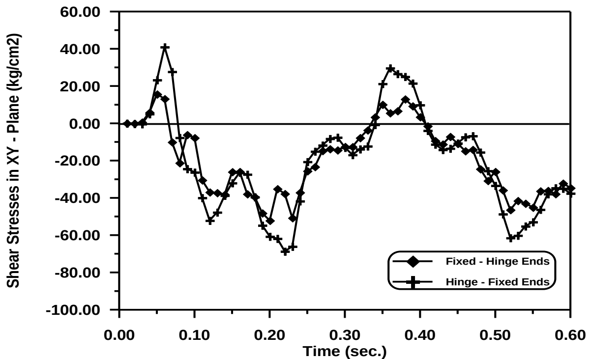
Figure (5-87) Time – Shear Stresses in XY - Plane Response at Gauss Point (53) with Various Boundary Conditions.
