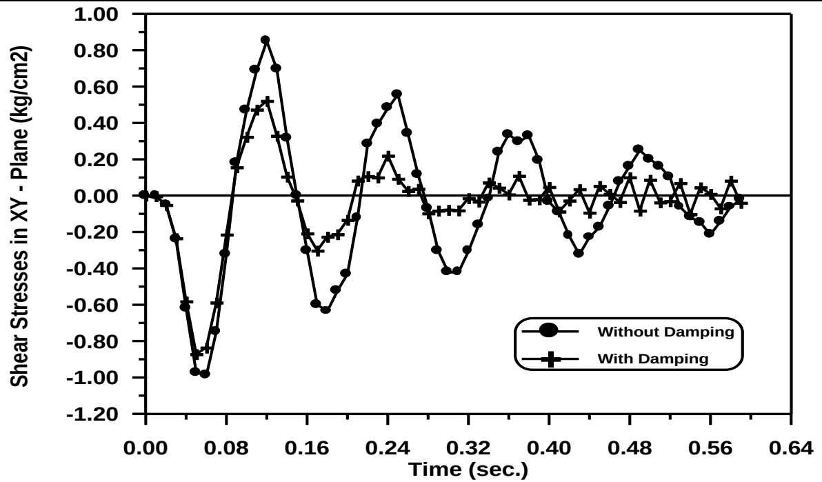
Figure (5-13) Time –Shear Stresses in XY - Plane Response of the Circular Arch at Gauss Point (62).
