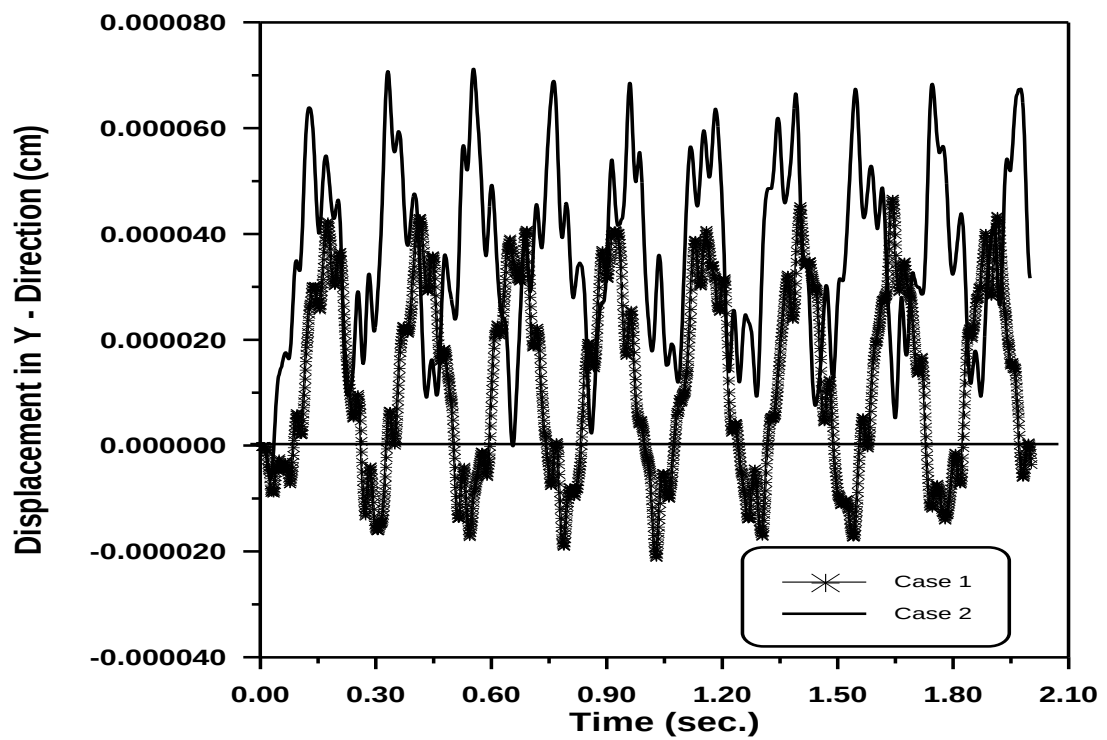
Figure(5-100) Time – Displacement in Y – Direction Response of the Circular Arch at ( \alpha=45^\circ )
