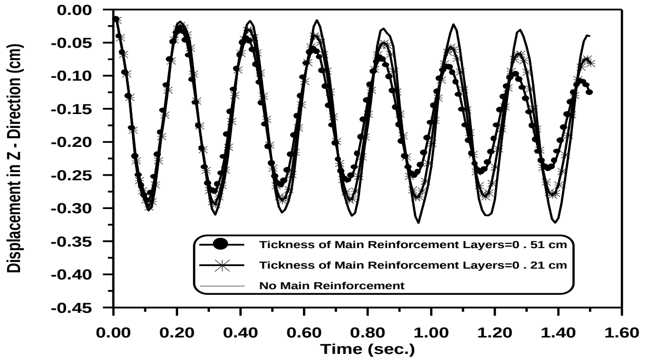
Figure (5-90) Effect the Thickness of Main Reinforcement Layers on Time – Displacement in Z - Direction Response at Center of Arch .
