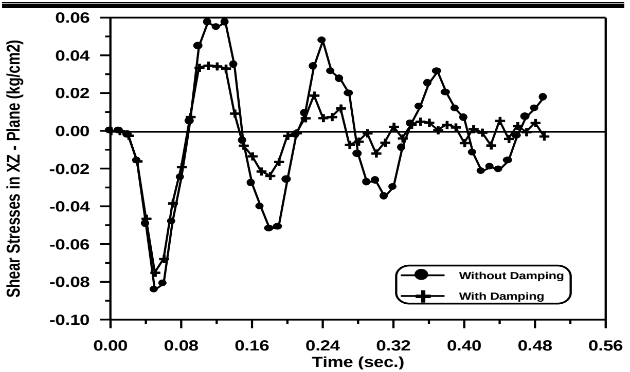
Figure (5-11) Time –Shear in XZ - Plane Stresses Response of the Circular Arch at Gauss Point (62)
