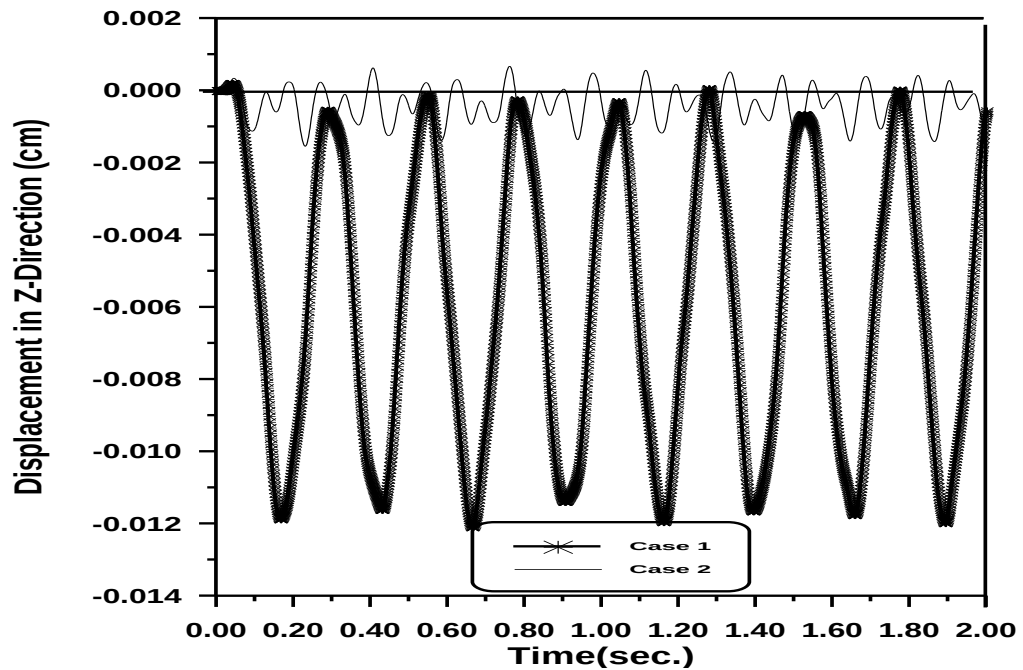
Figure(5-102) Time – Displacement in Z – Direction Response of the Circular Arch at ( \alpha=45^\circ )
