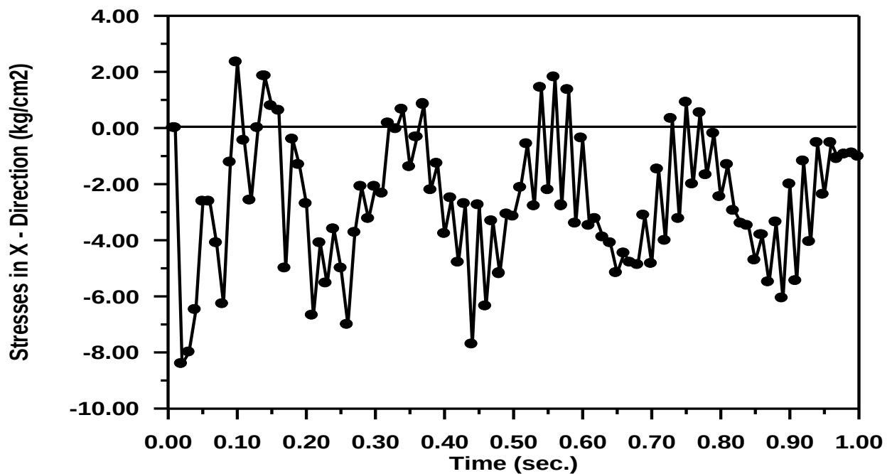
Figure (5-95) Time – Stresses in X - Direction Response at Gauss Point (6) .
