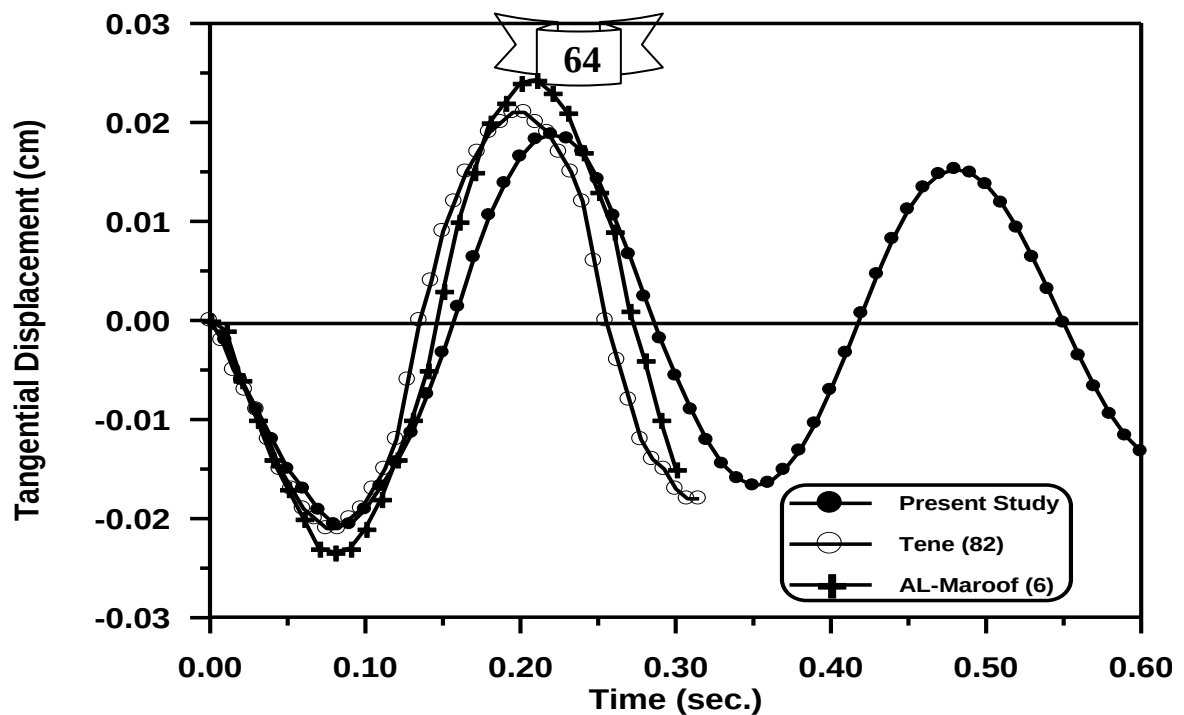
Figure (5-8) Time – Tangential Displacement Response for Dynamic Response of the Circular Arch Without Damping at ( \alpha = 67.5^\circ ).
