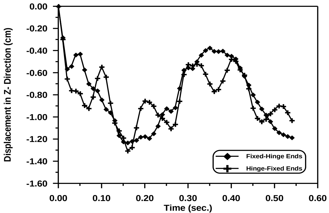
Figure (5-70) Time – Displacement in Z - Direction Response at ( \alpha=50^\circ ) with Various Boundary Condition.
