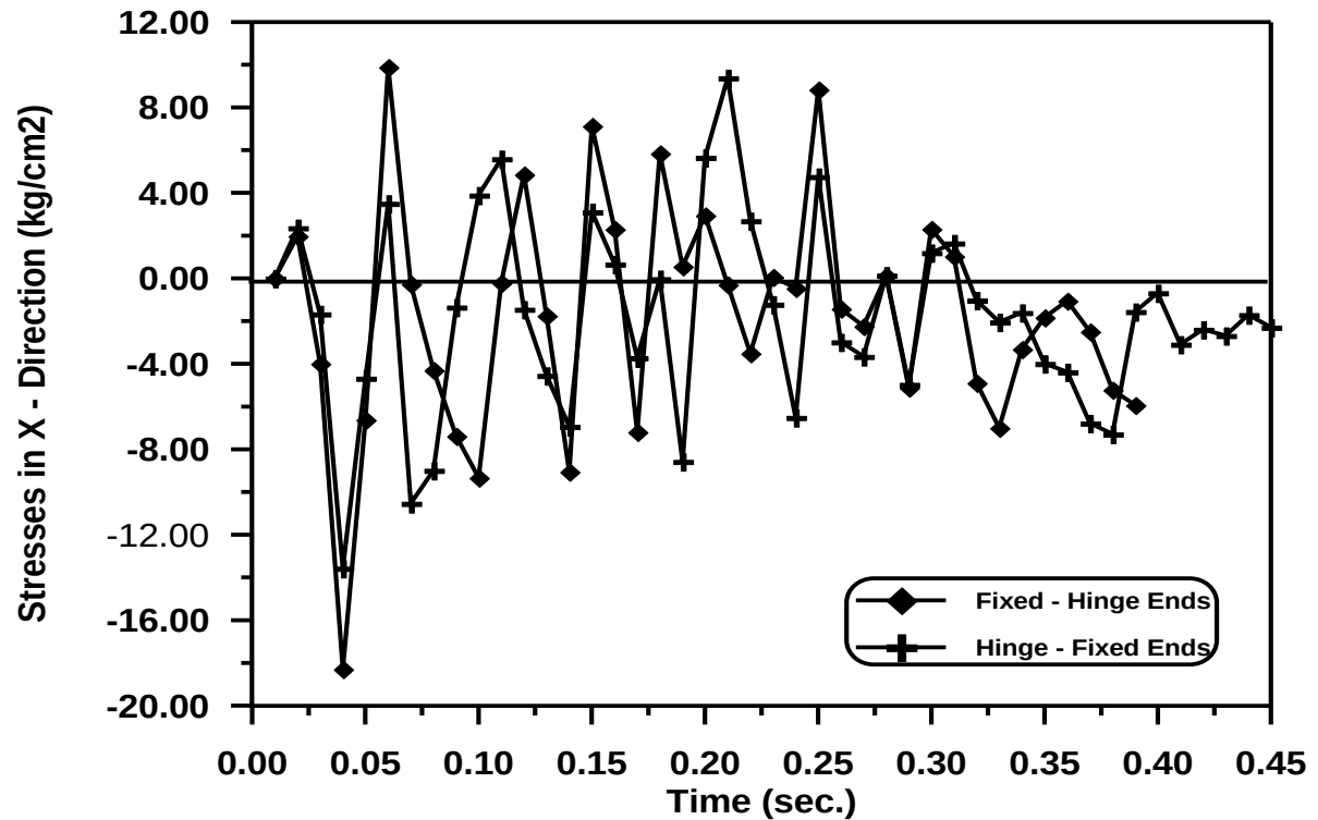
Figure (5-79) Time – Stresses in X - Direction Response at Gauss Point (25 or 26) With Various Boundary Condition.
