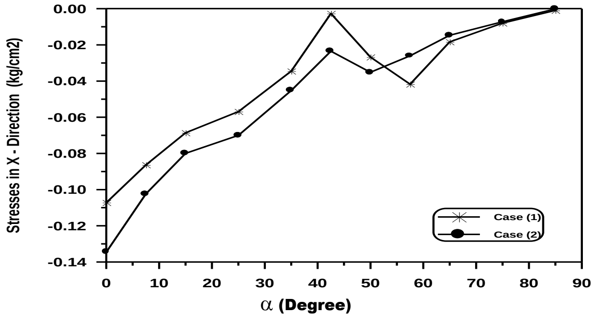
Figure (5-45) The Stresses in X - Direction Along the Arch at (t=0.0025 sec.).
