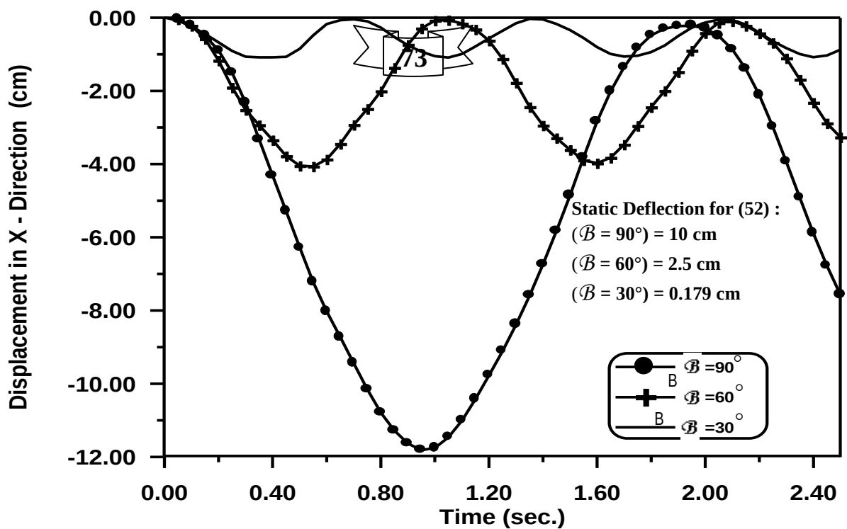
Figure (5-18) Time – Displacement in X - Direction Response at Free End for Curved Cantilever with Three Subtended Angles.
