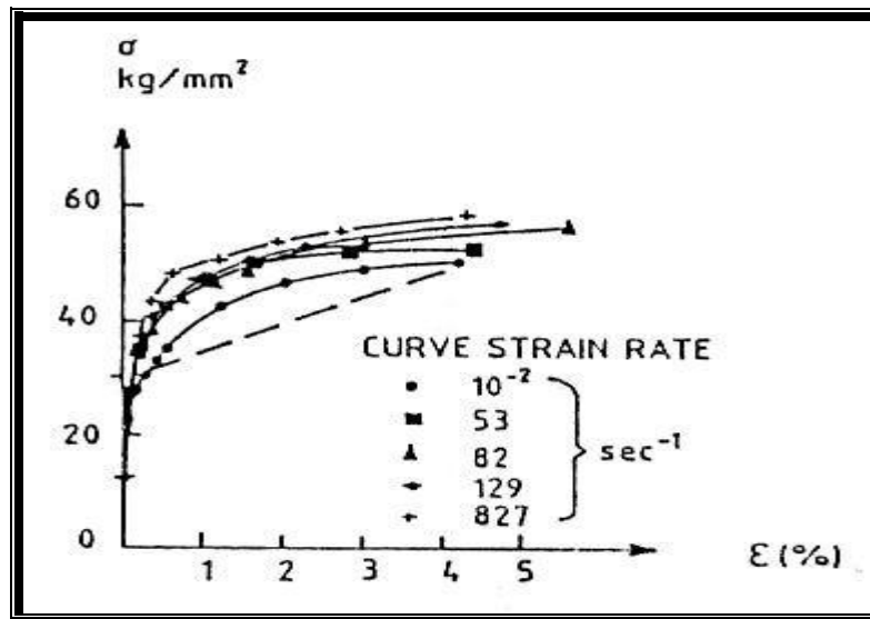
Figure (3.11) Dynamic Stresses – Strain Diagram for Steel (44) .
