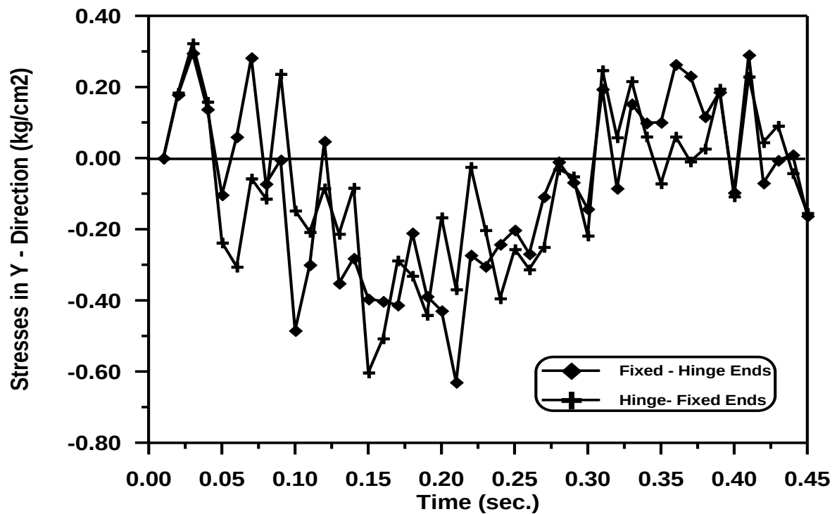
Figure (5-78) Time – Stresses in Y - Direction Response at Gauss Point (25 or 26) With Various Boundary Condition.
