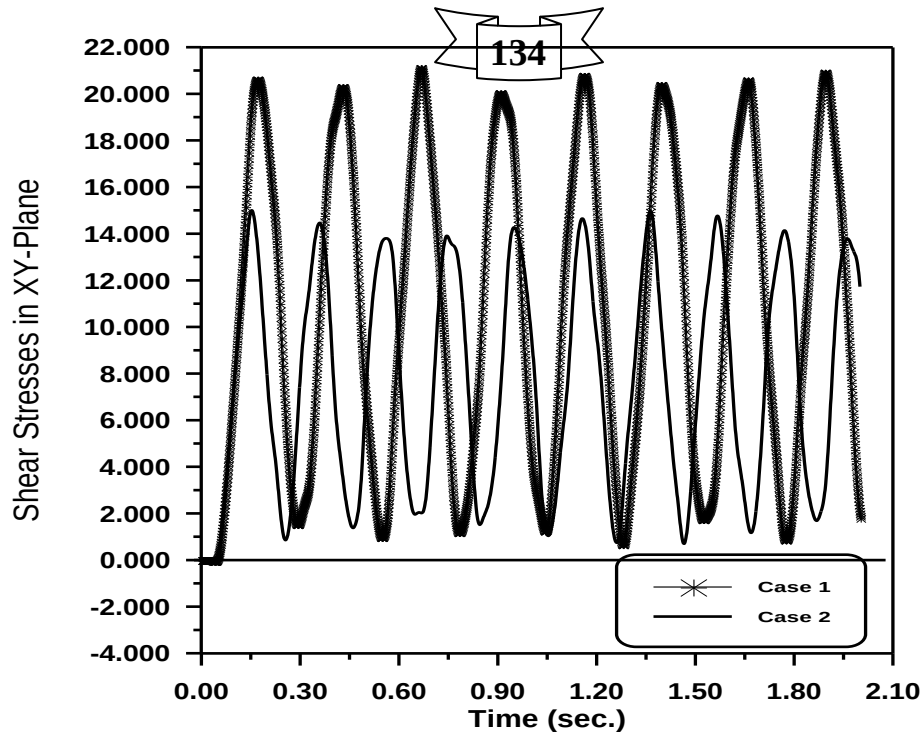
Figure(5-107) Time – Shear Stresses in XY - Plane Response at Gauss Point (35) with Various Boundary Conditions.
