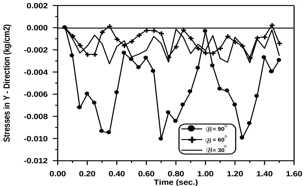
Figure (5-21) Time – Stresses in Y - Direction Response at Gauss Point (6) for Curved Cantilever with Three Subtended Angles.
