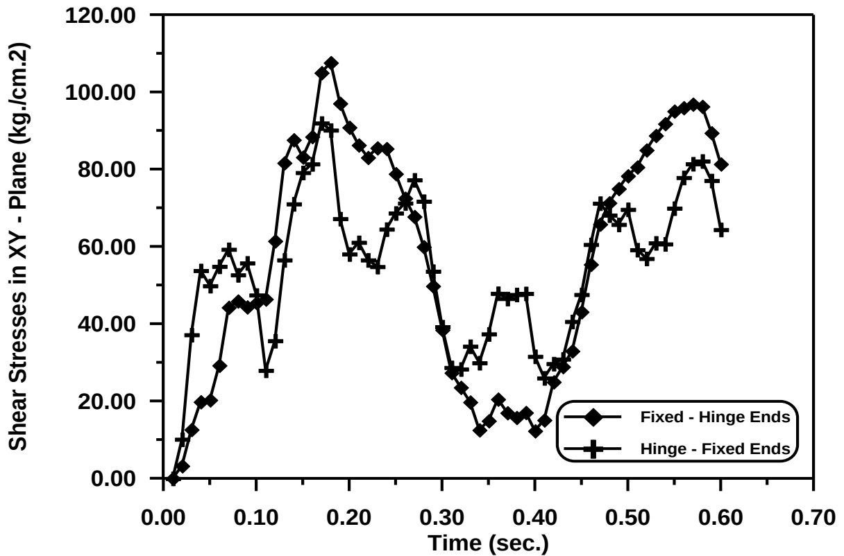
Figure (5-85) Time – Shear Stresses in XY - Plane Response at Gauss Point (6) with Various Boundary Conditions.
