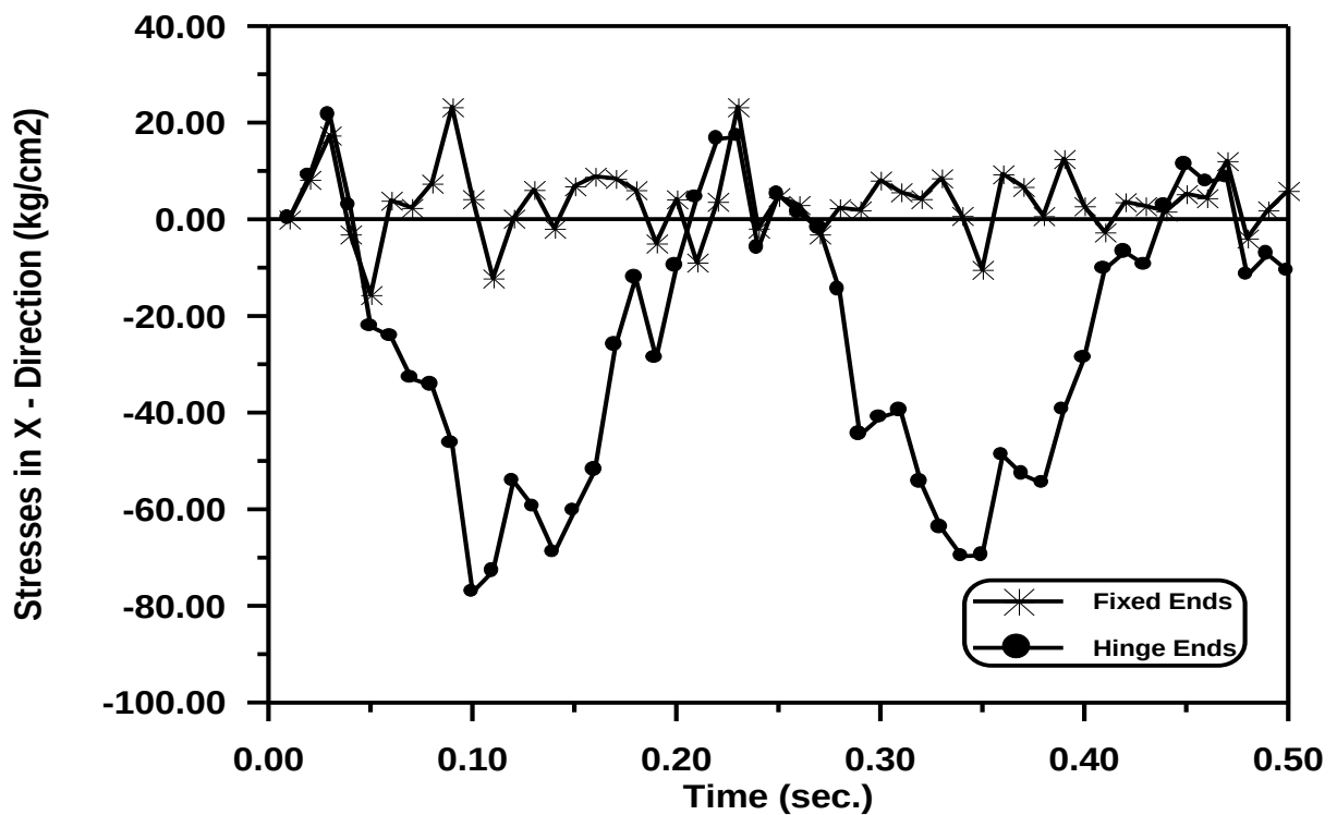
Figure (5-84) Time – Stresses in X - Direction Response at Gauss Point (28) With Various Boundary Conditions.
