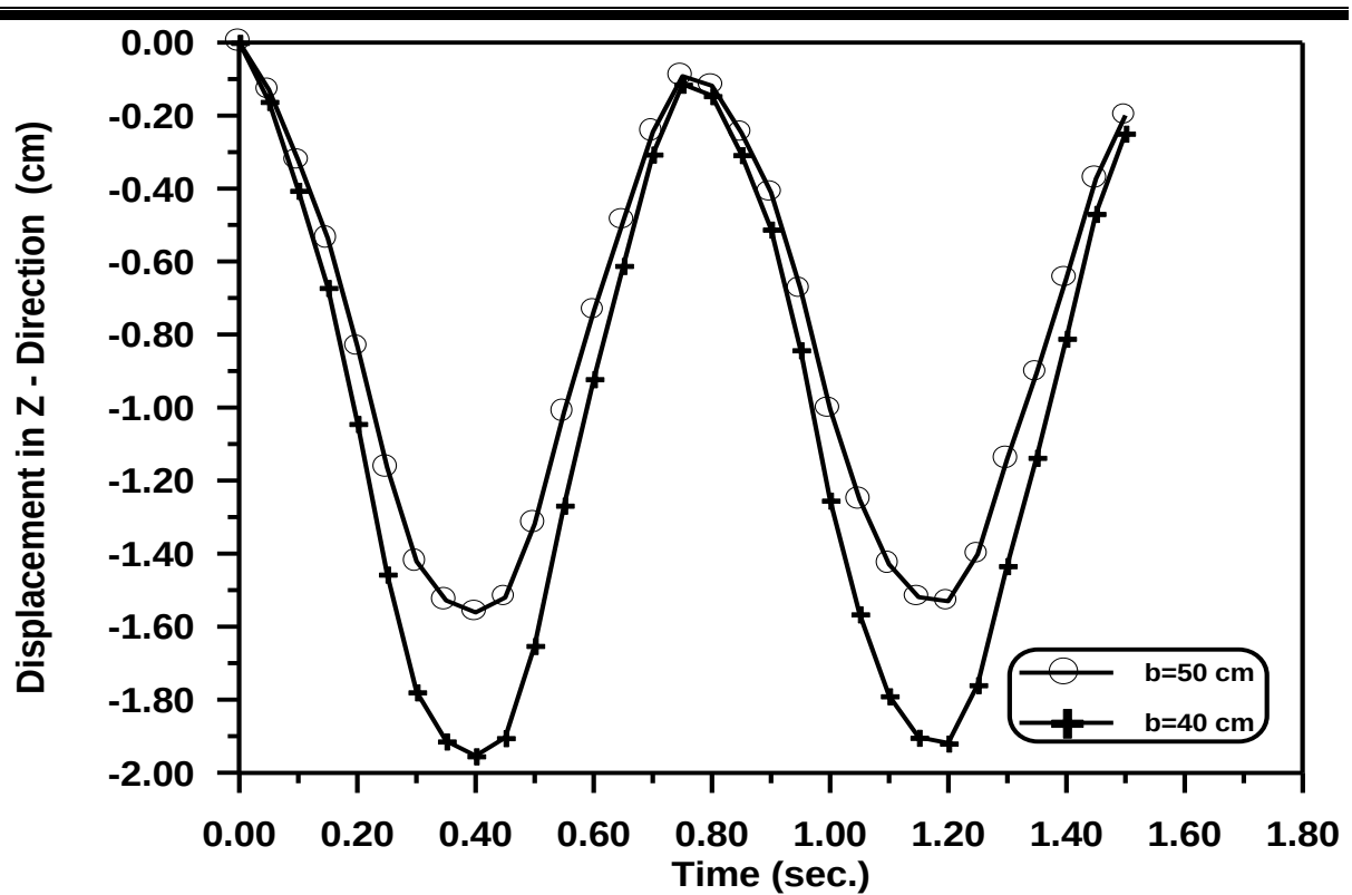
Figure (5-49) Effect the Change of Width on Time – Displacement in Z – Direction Response at A center of Arch with Number of Element = 9.
