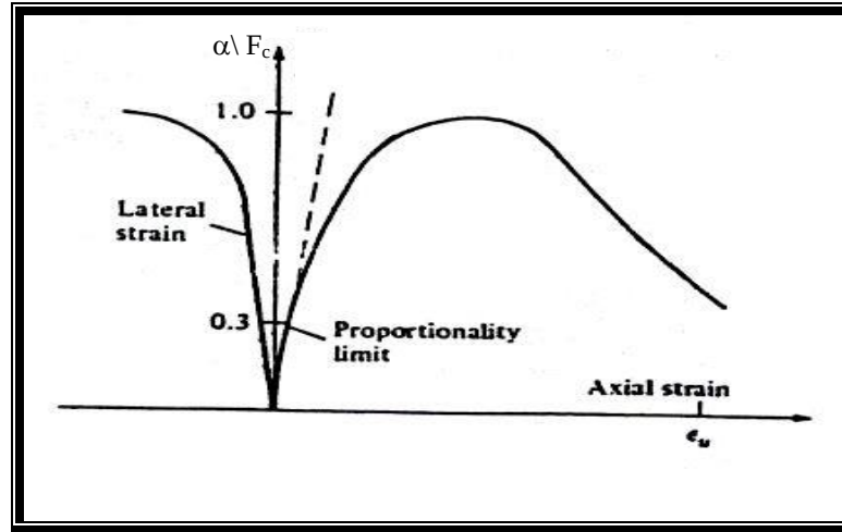
Figure (3.1) Typical Plot of Compressive and Lateral Strain of Concrete (23) .
