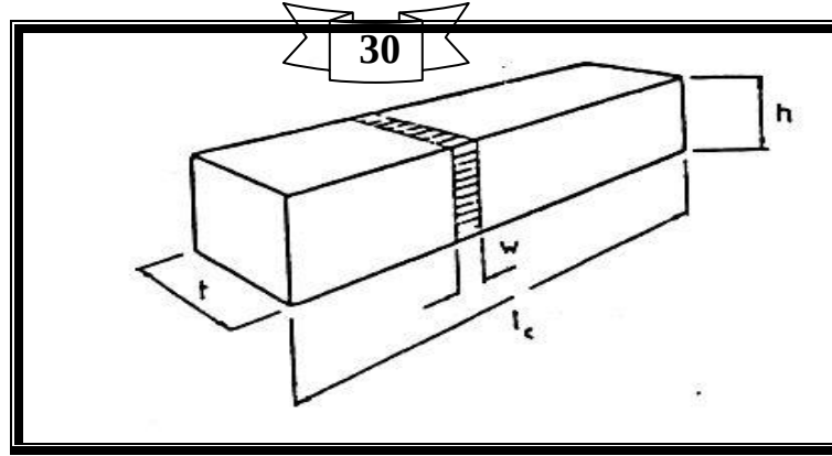
Figure (3.8) Illustration of Characteristic Length for A prismatic Control Volume (44) .
