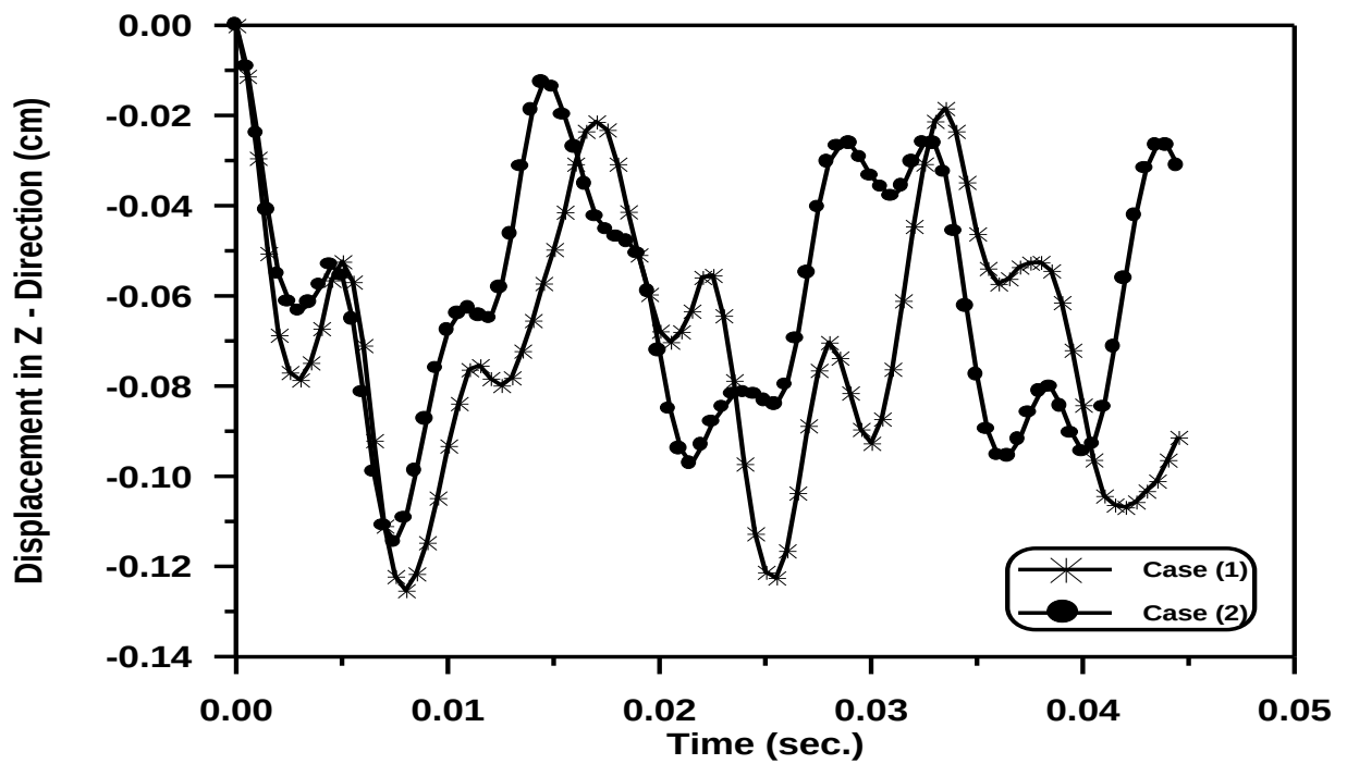
Figure (5-32) Time – Displacement in Z - Direction Response
