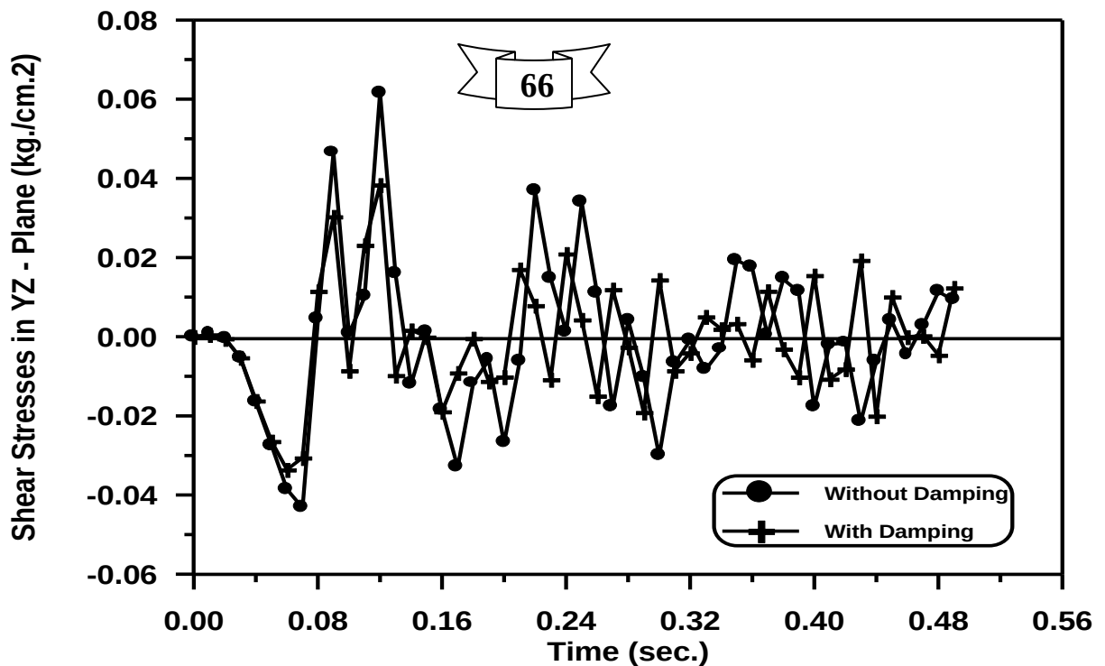
Figure (5-12) Time –Shear Stresses in YZ – Plane Response of the Circular Arch at Gauss Point (62).
