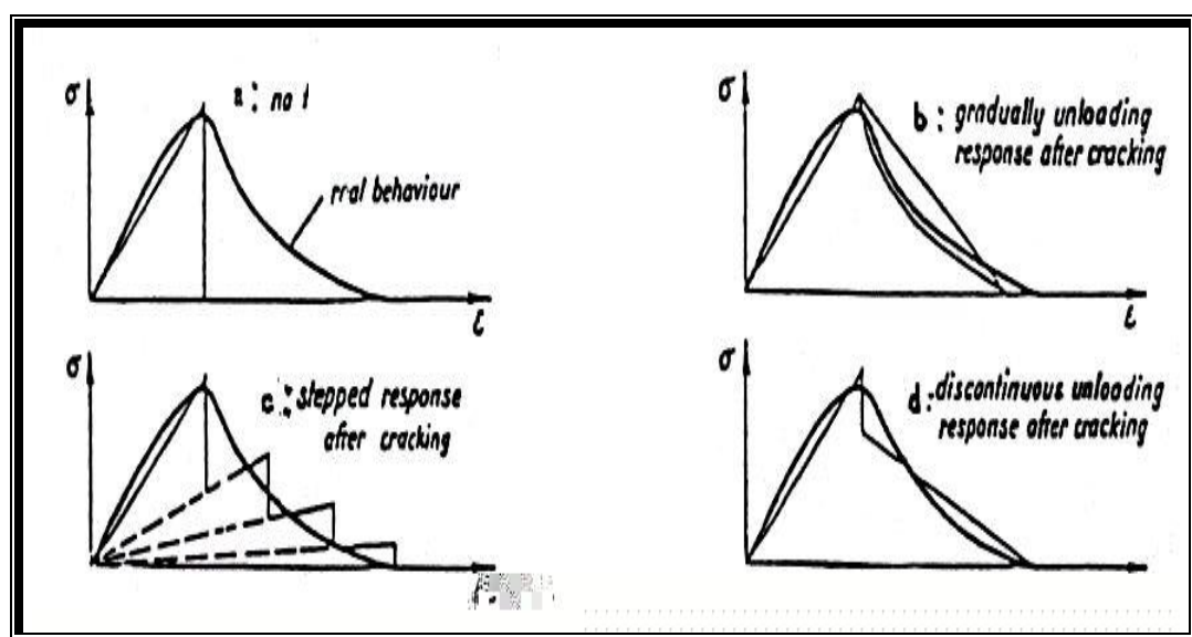
Figure (3.7) Some Possible Assumptions for Strain – Softening of Concrete After Cracking (61) .
