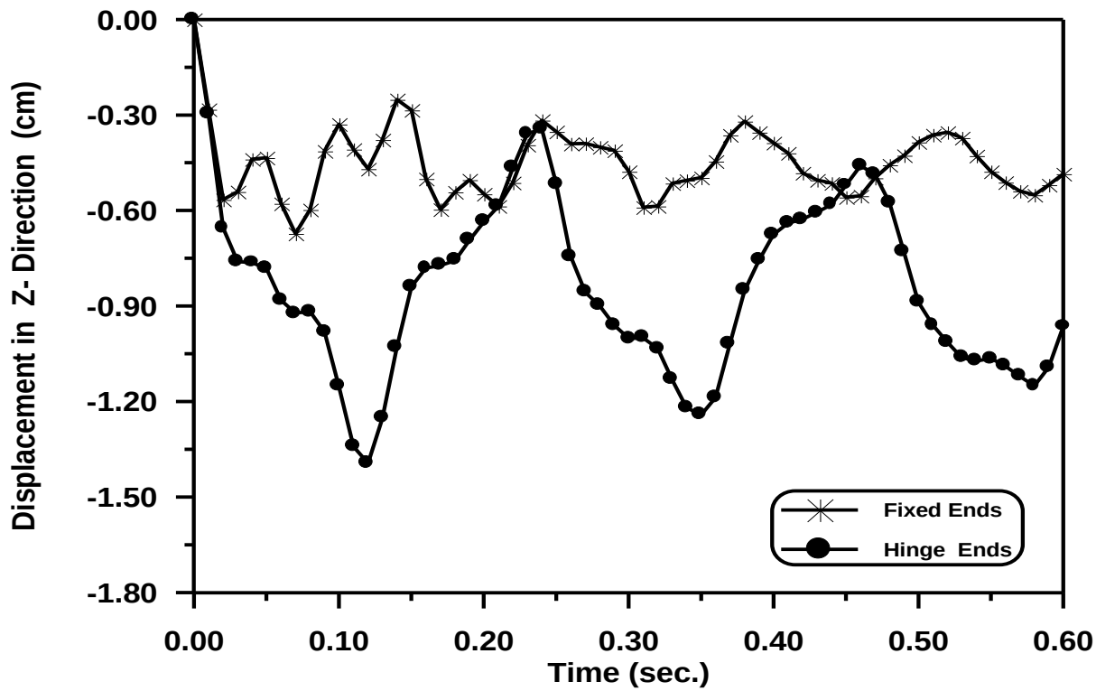
Figure (5-66) Time – Displacement in Z - Direction Response at ( \alpha=50^\circ ) with Various Boundary Condition.
