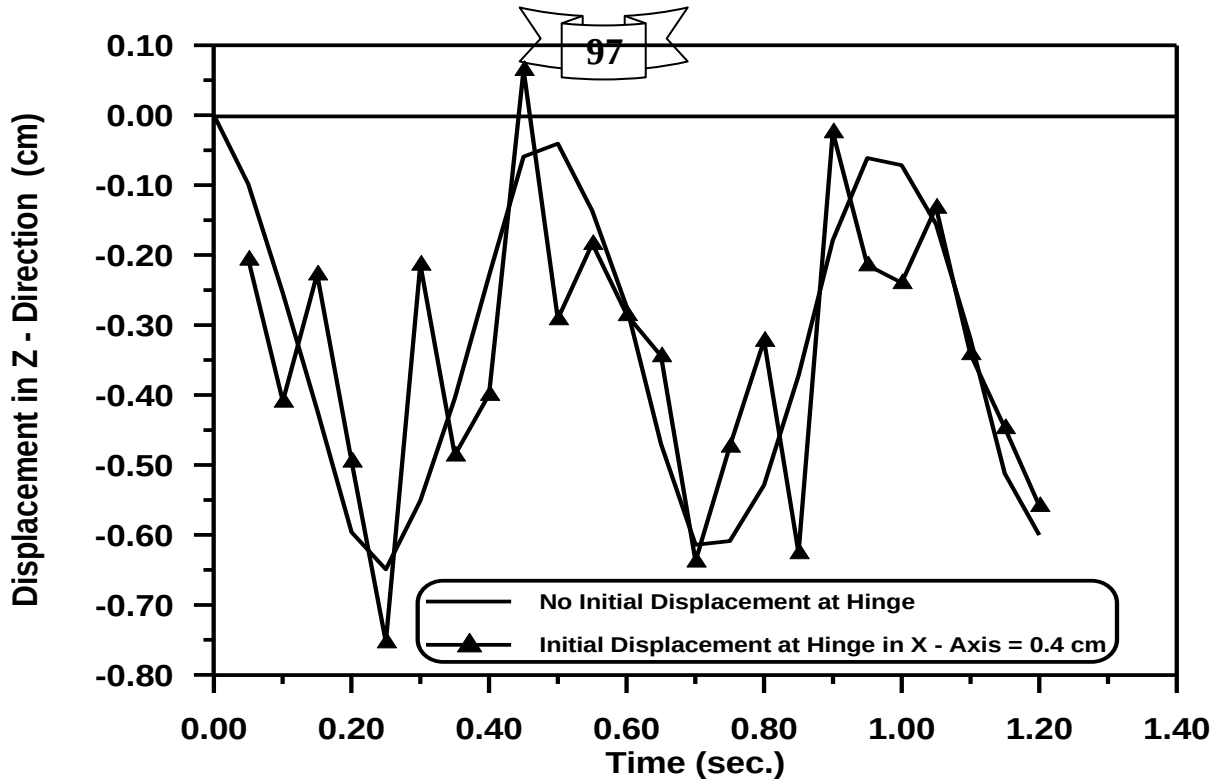
Figure (5-52) Effect Initial Displacement at Hinge on Time -Displacement in Z - Direction Response at Center of Arch for Number of Element = 5.
