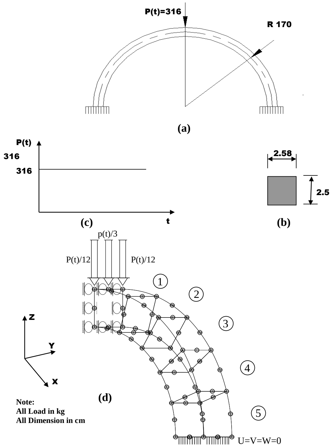
(a) geometry and loading of arch (b) cross section (c) load – time relation (d) finite element idealization and numbering of half of the arch
