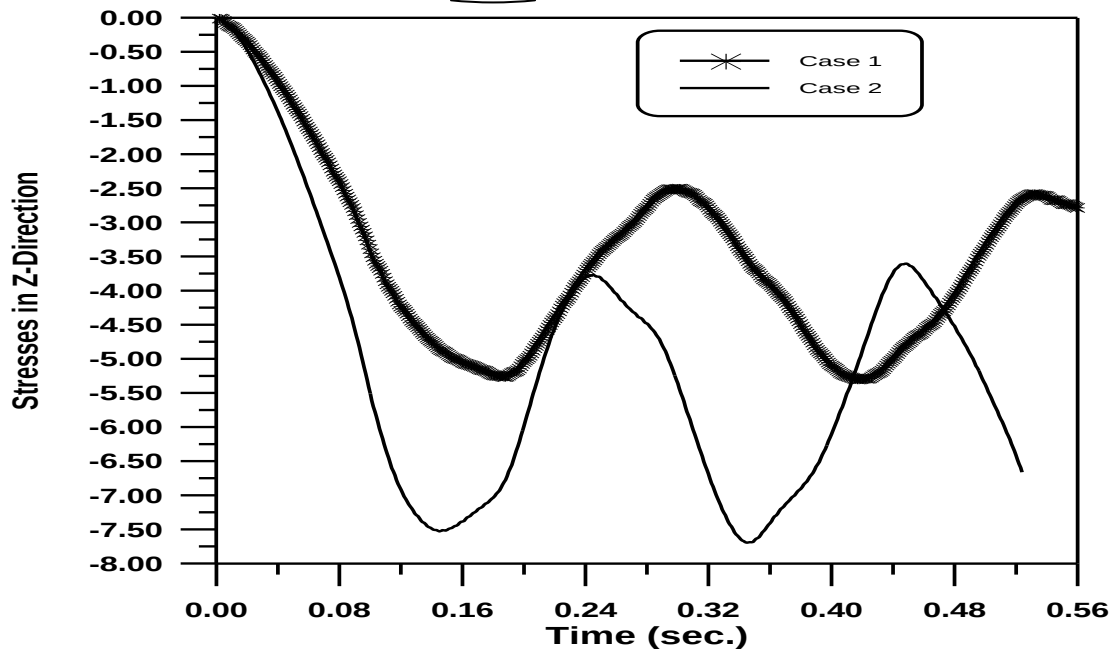
Figure(5-105) Time – Stresses in Z – Direction Response at Gauss Point (6) of Center Circular Arch
