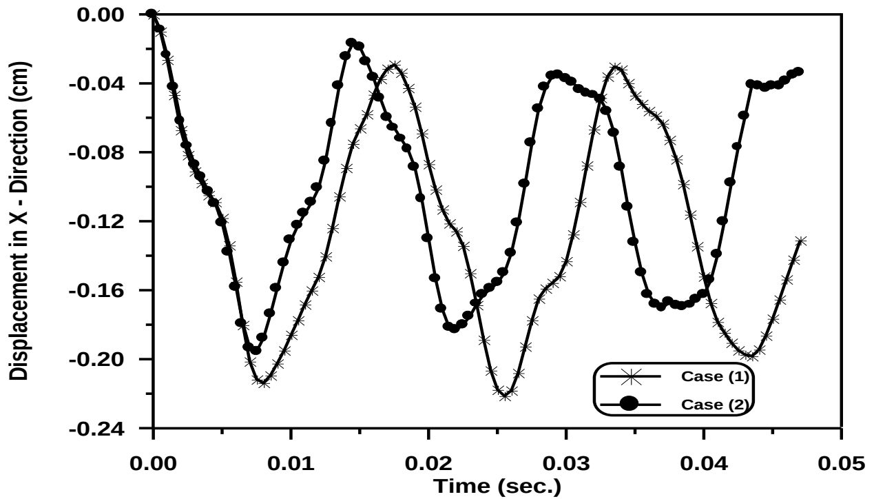
Figure (5-33) Time – Displacement in X - Direction Response of The Circular Arch at ( \alpha=42.5^\circ ).
