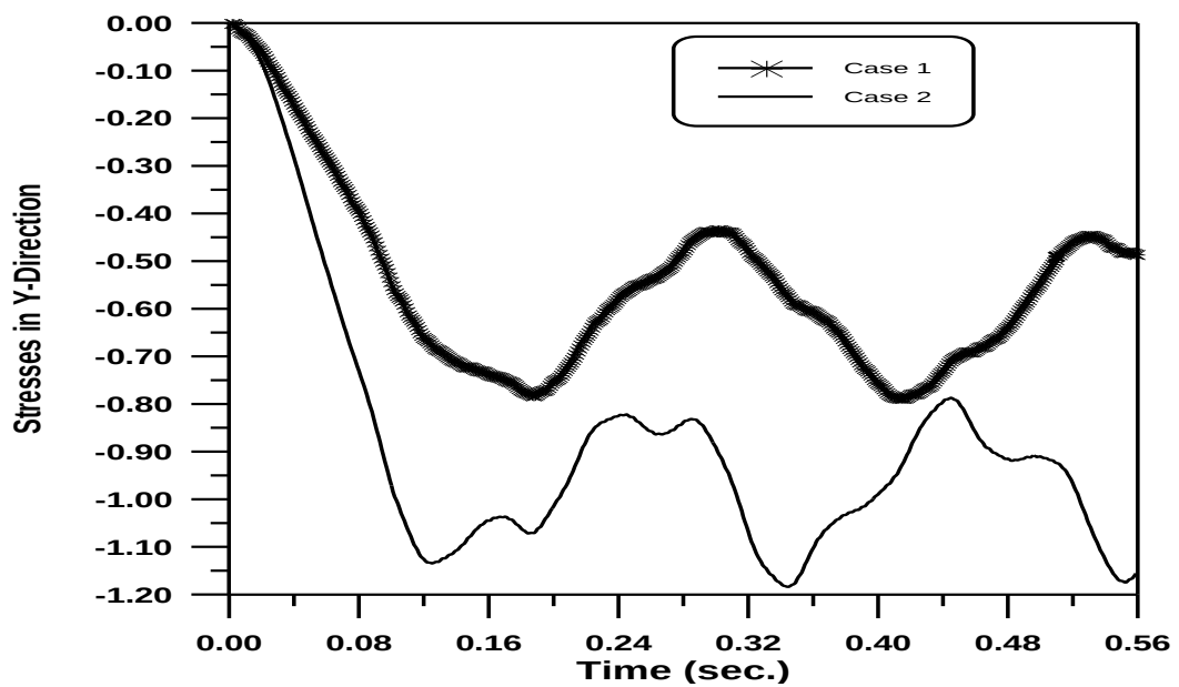
Figure(5-104) Time – Stresses in Y – Direction Response at Gauss Point (6) of Center Circular Arch
