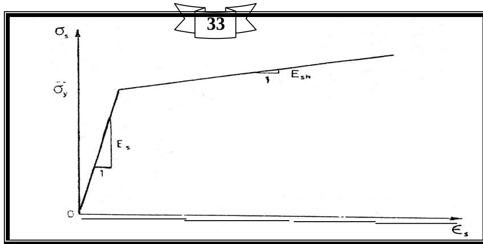
Figure (3.10) Typical Stresses – Strain Curve for Steel (3) .
