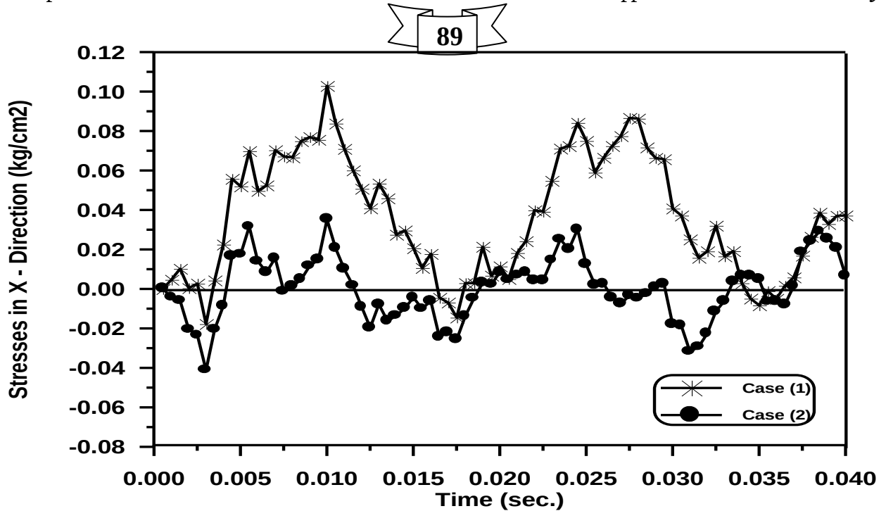
Figure (5-41) Time – Stresses in X - Direction Response of The Circular Arch at Gauss point (31) .
