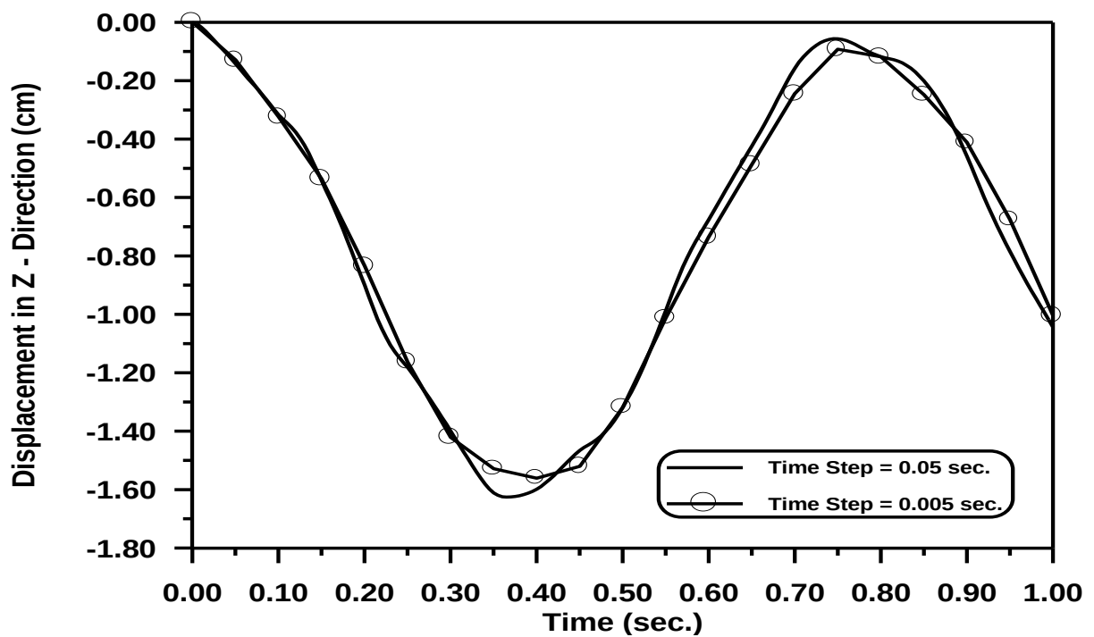
Chapter Five Figure (5-51) Effect of Time – step on Time – Displacement in Z - Direction Response at Center of Arch. Number of Elements = 5 and Parametric Study
