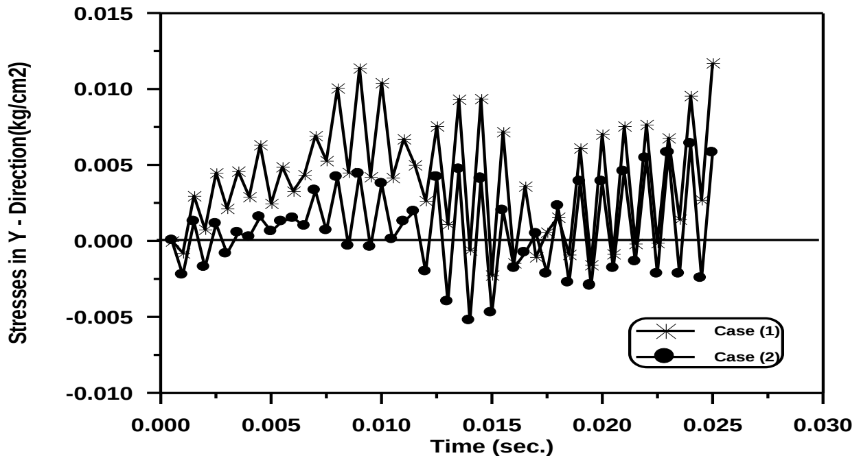
Figure (5-43) Time – Stresses in Y - Direction Response of The Circular Arch at Gauss point (31) .
