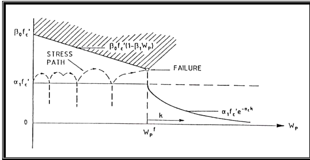
Figure (3.4) Variation of the Yield and Failure with the Dissipated Energy Density (44) .
