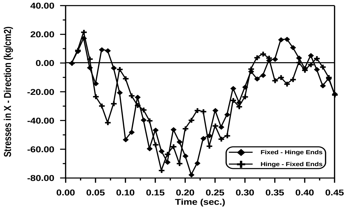
Figure (5-83) Time – Stresses in X - Direction Response at Gauss Point (28) With Various Boundary Conditions.
