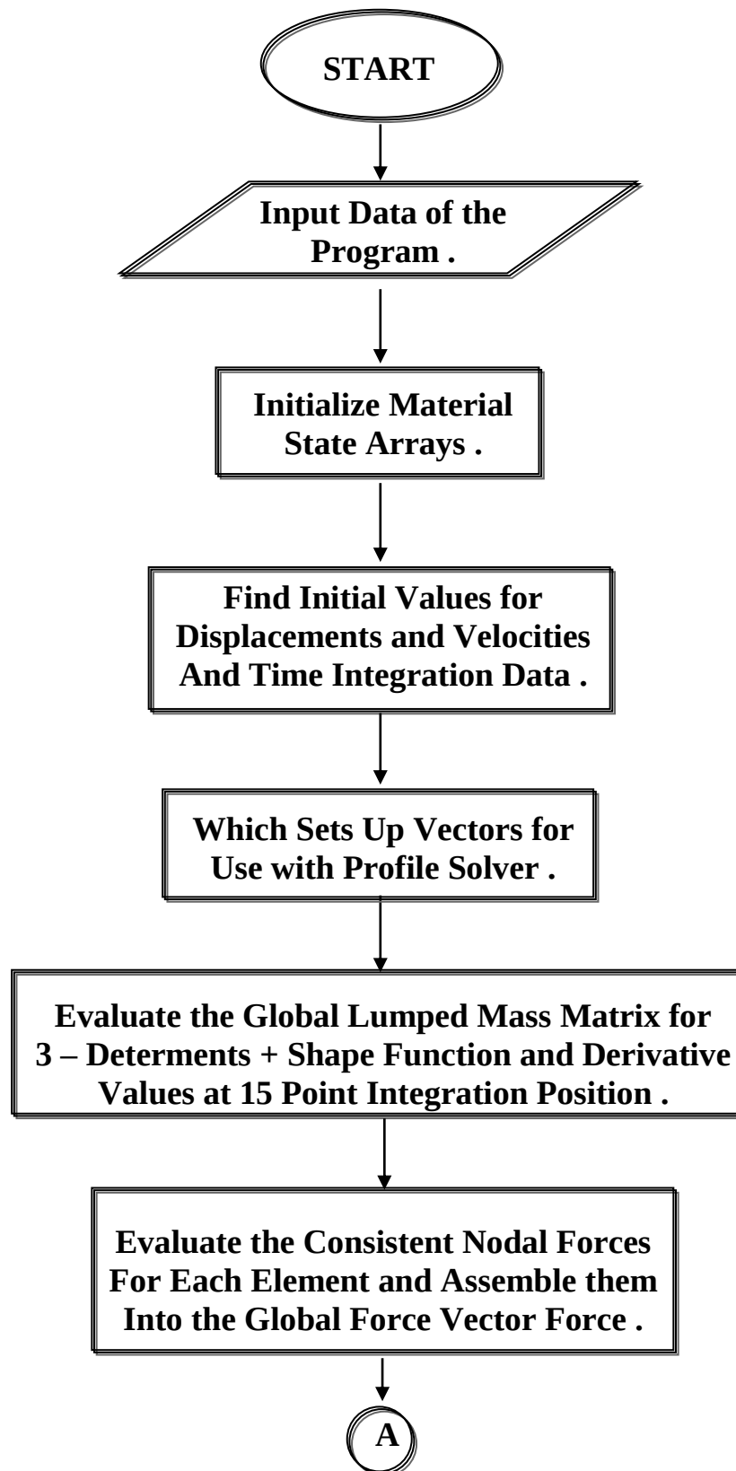
Figure (4.5) Flowchart of the Program DARC3
