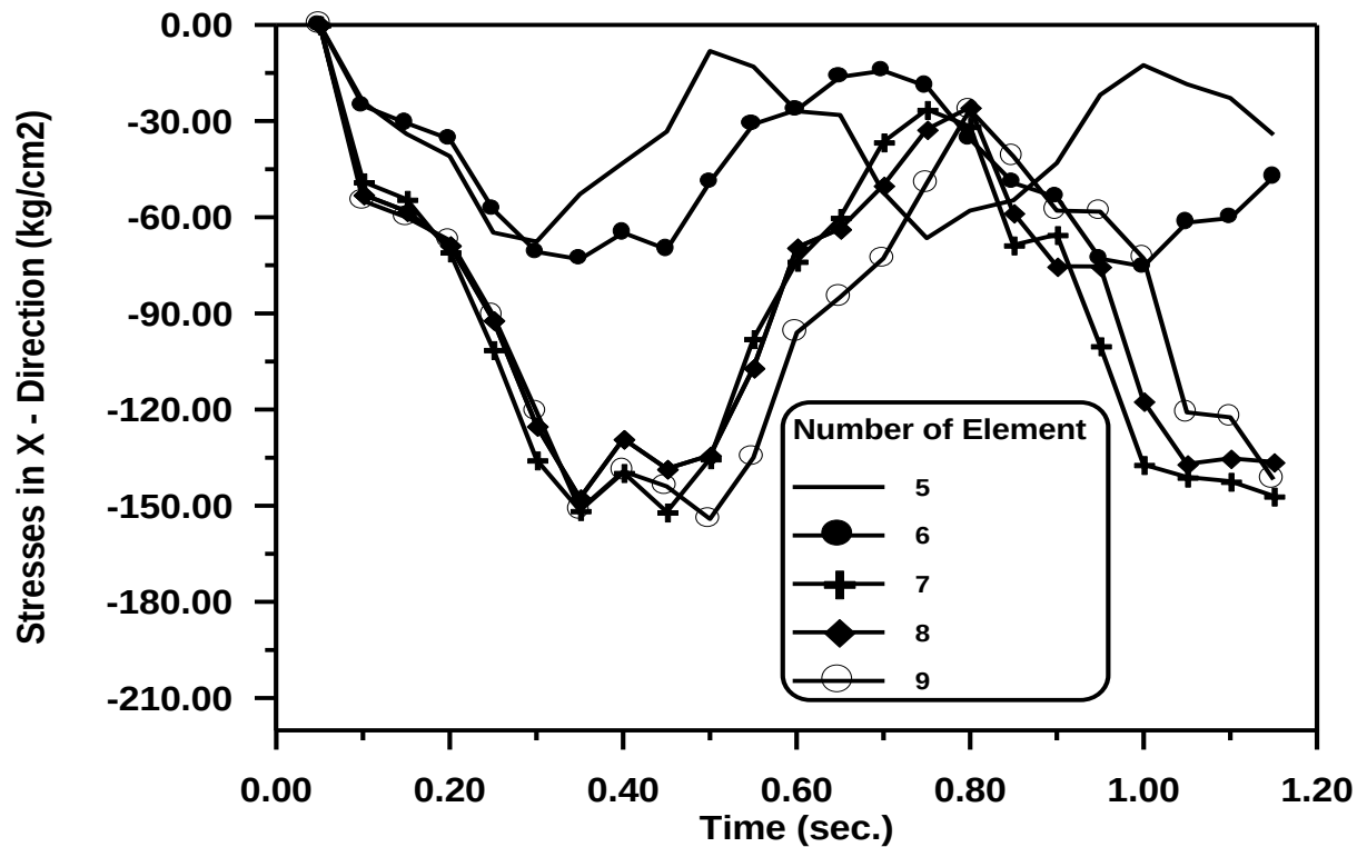
Figure (5-55) Effect the Number of Elements on Time – Stresses Chapter Five In X – Direction Response of Arch at Gauss Point (4). Numerical Application and Parametric Study
