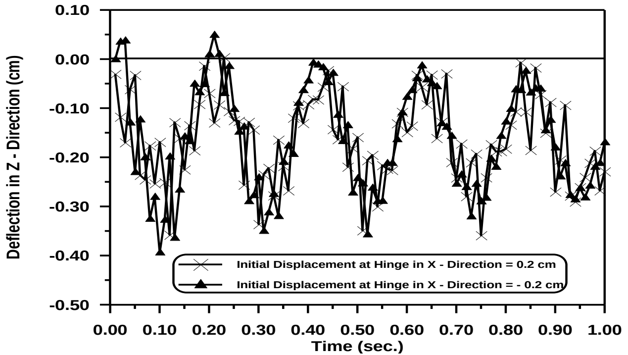
Figure (5-94) Effect the Initial Displacement on Time – Displacement in Z - Direction Response at Center of Arch
