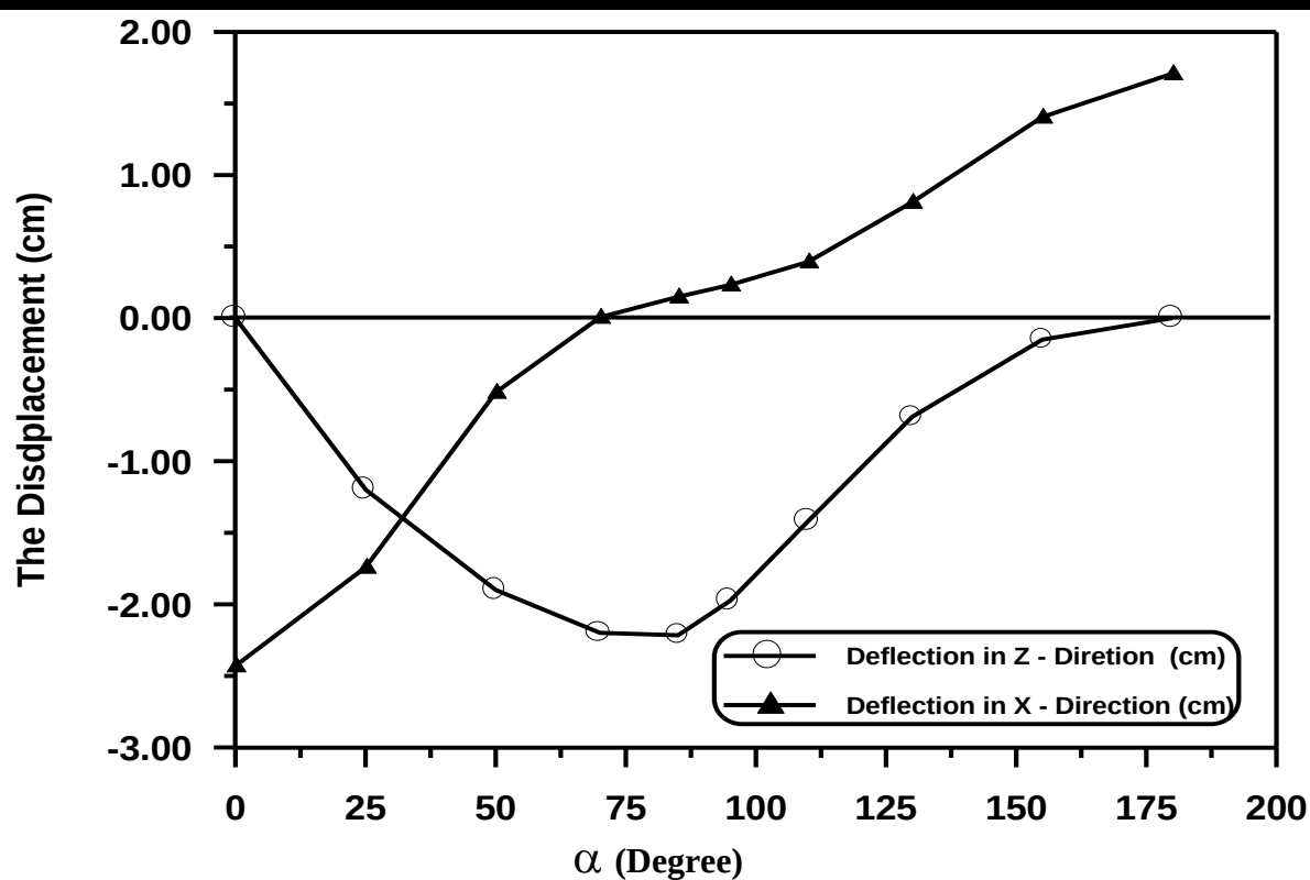
Figure (5-71) The Displacement Along the Arch Under Dynamic Load with Hinge – Hinge Ends at (t=0.35 sec.).
