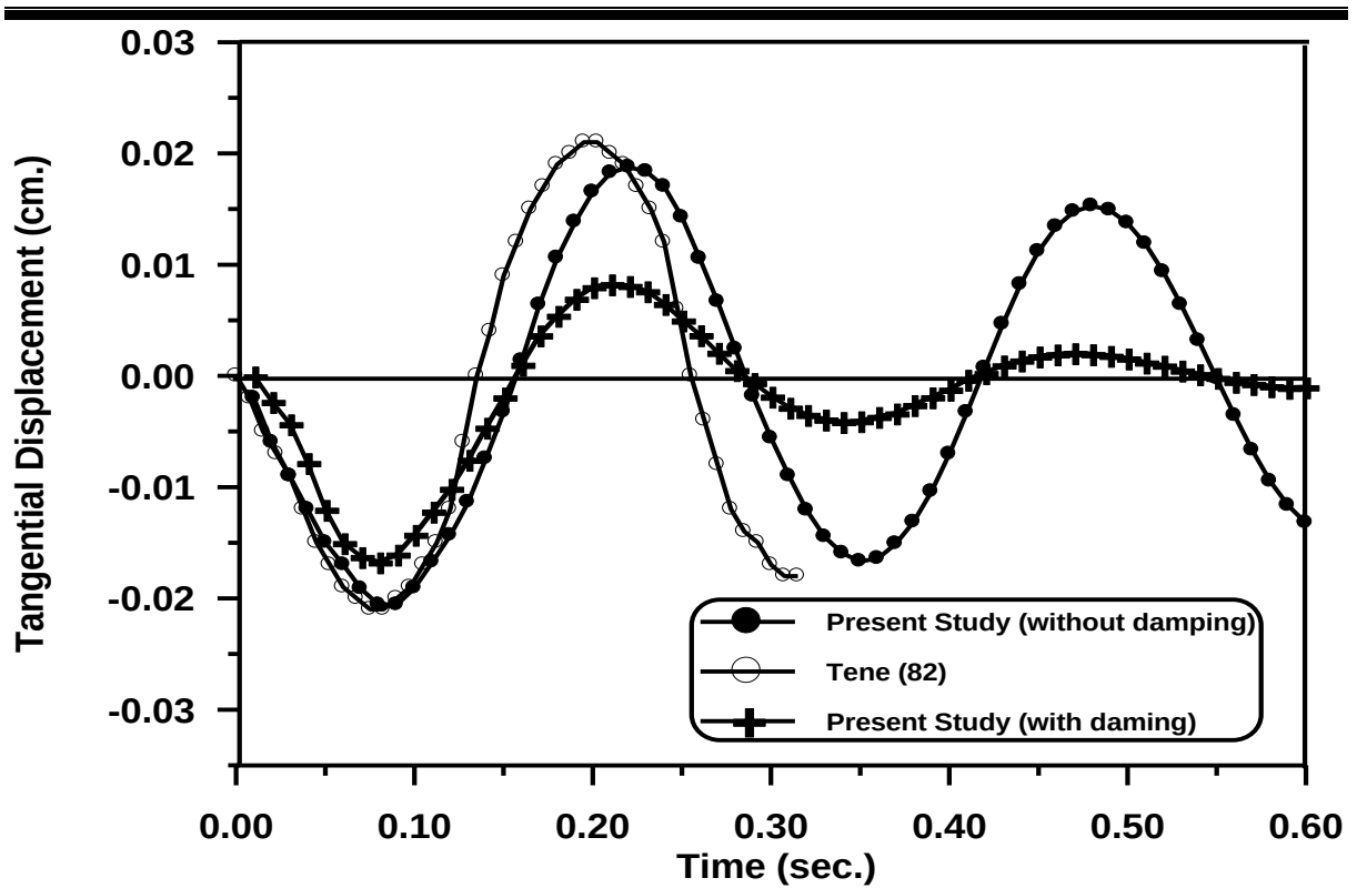
Figure (5-7) Time – Tangential Displacement Response for Dynamic Response of the Circular Arch at ( \alpha = 67.5^\circ ).
