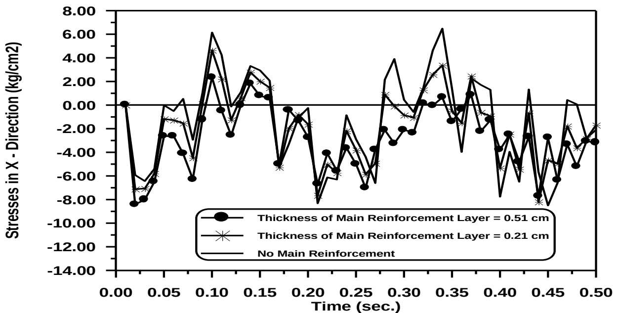
Figure (5-97) Effect the Thickness of Main Reinforcement Layers on Time – Stresses Response at Gauss Point (6) .
