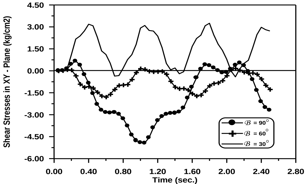
Figure (5-29) Time – Shear Stresses in XY - Plane Response at Gauss Point(30) For Curved Cantilever with Three Subtended Angles.
