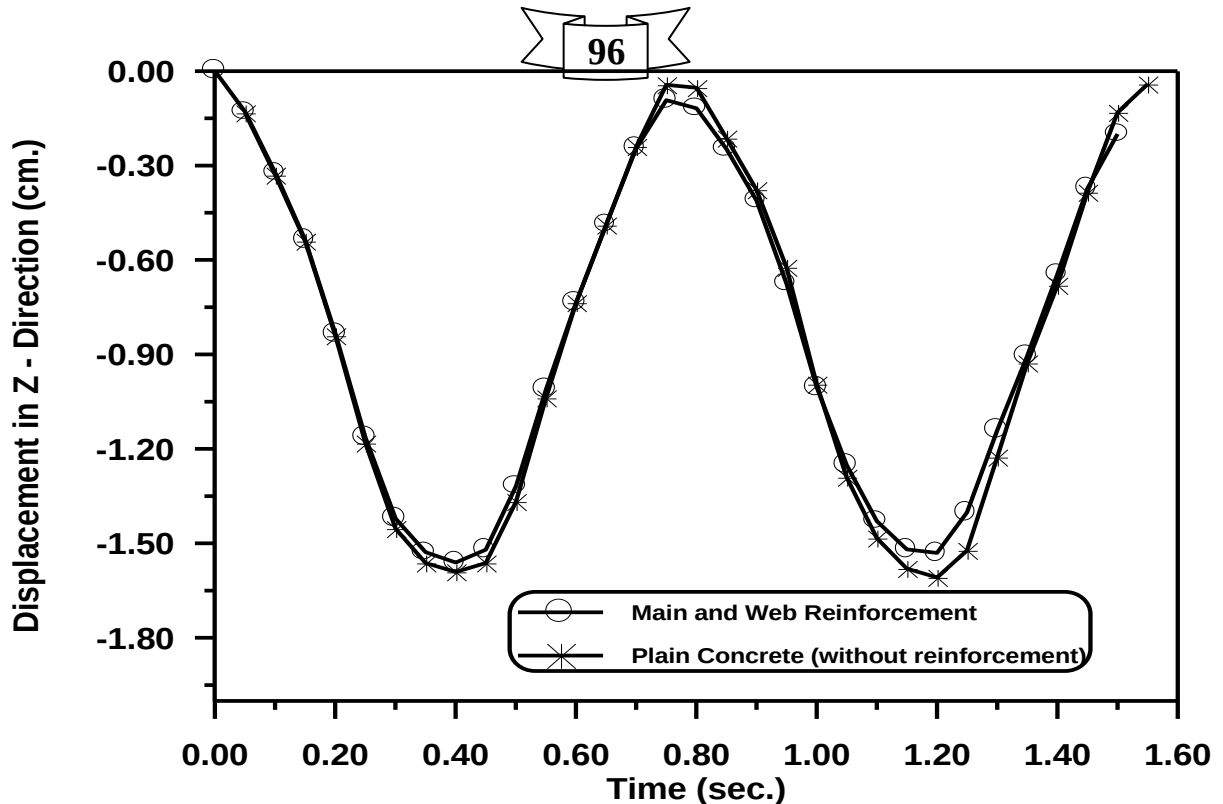
Figure (5-50) Effect of Reinforcement on Time – Displacement in Z - Direction Response at Center of Arch.
