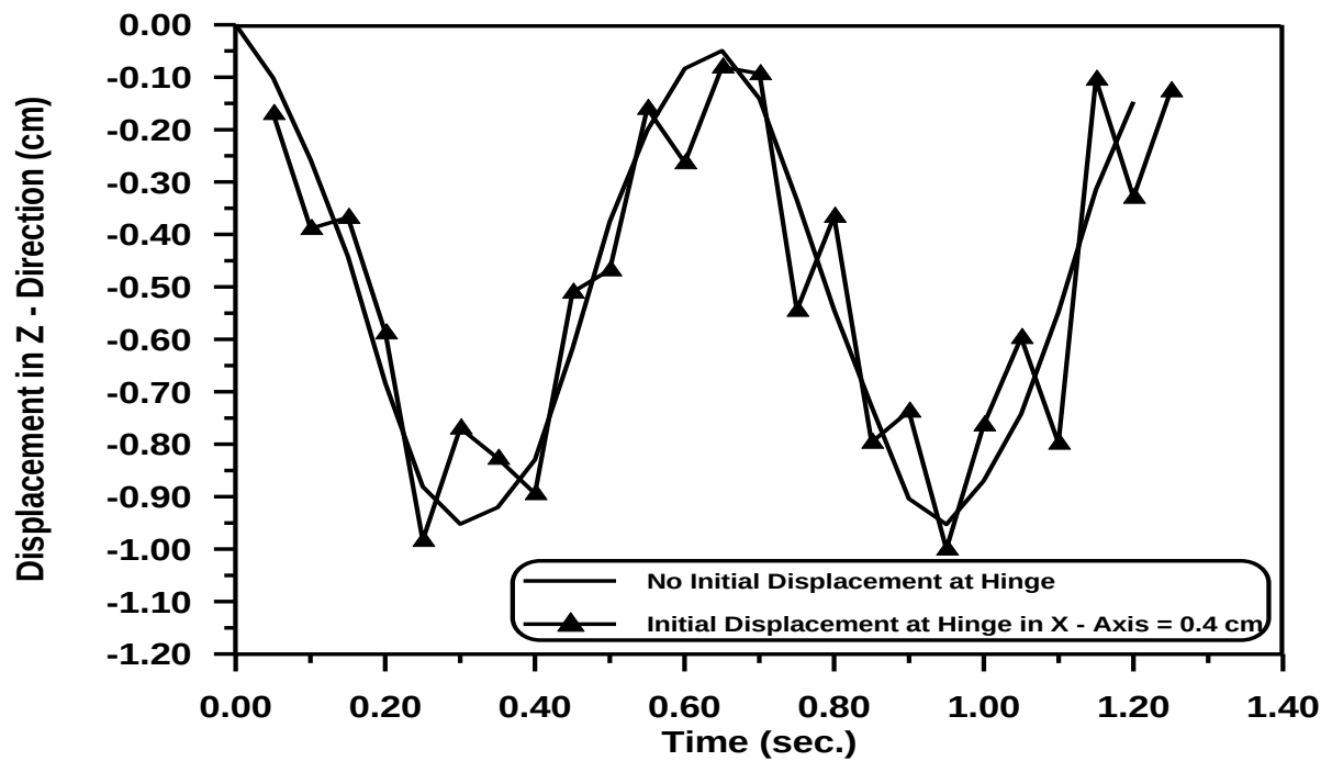
Figure (5-53) Effect Initial Displacement at Hinge on Time –Displacement in Z - Direction Response at Center of Arch for Number of Element = 6. Chapter Five Numerical Application and Parametric Study
