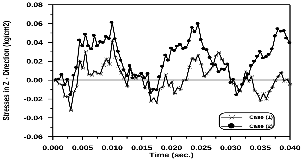
Figure (5-42) Time – Stresses in Z – Direction Response of The Circular Arch at Gauss point (31) .
