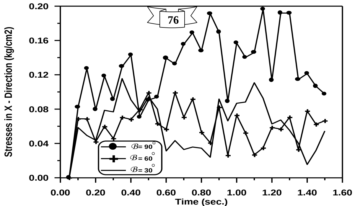
Figure (5-24) Time – Stresses in X - Direction Response at Gauss Point (5) For Curved Cantilever with Three Subtended Angles.
