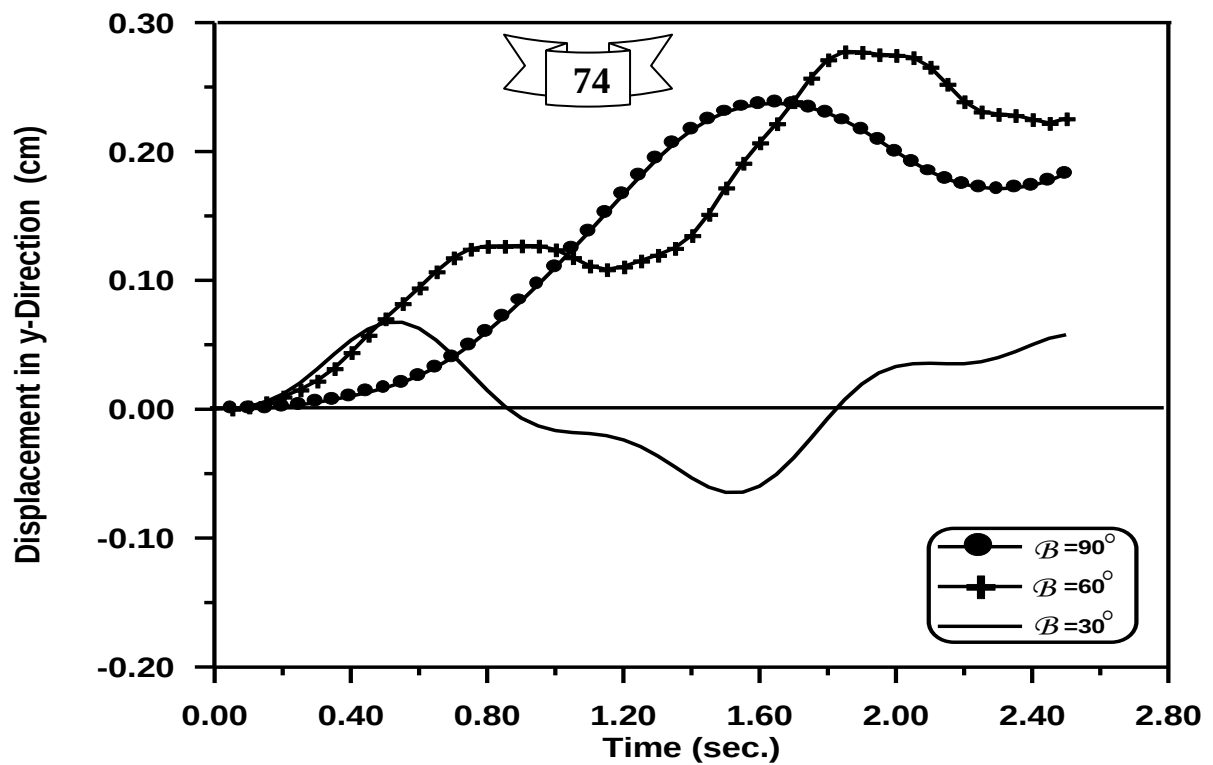
Figure (5-20) Time – Displacement in Y - Direction Response at Free End for Curved Cantilever with Three Subtended Angles.
