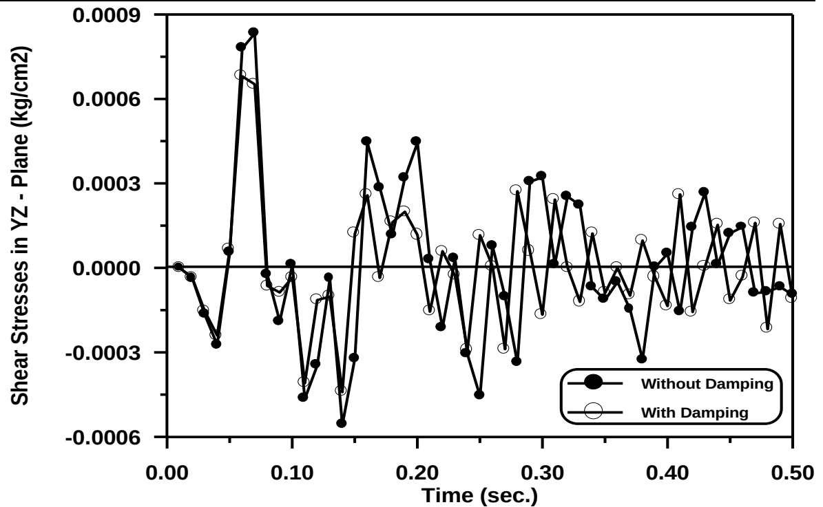
Figure (5-15) Time –Shear Stresses in YZ - Plane Response of the Circular Arch at Gauss Point (63).
