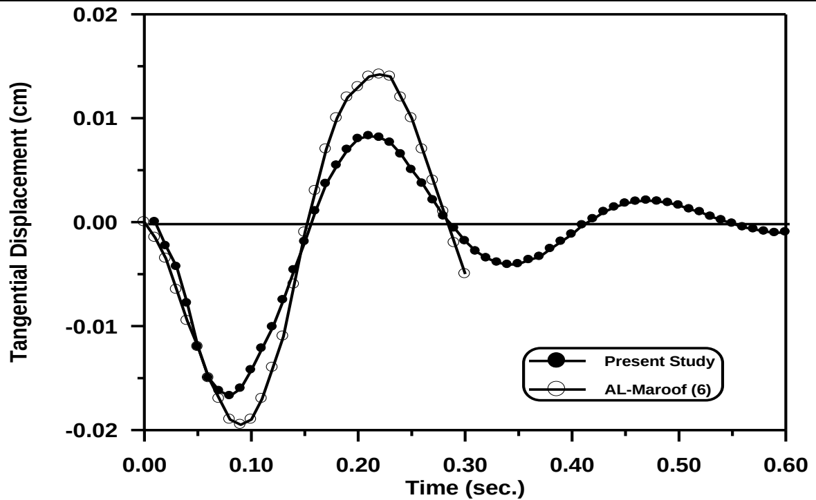
Figure (5-9) Time – Tangential Displacement Response for Dynamic Response of the Circular Arch With Damping at ( \alpha = 67.5^\circ ). Chapter Five Numerical Application and Parametric Study
