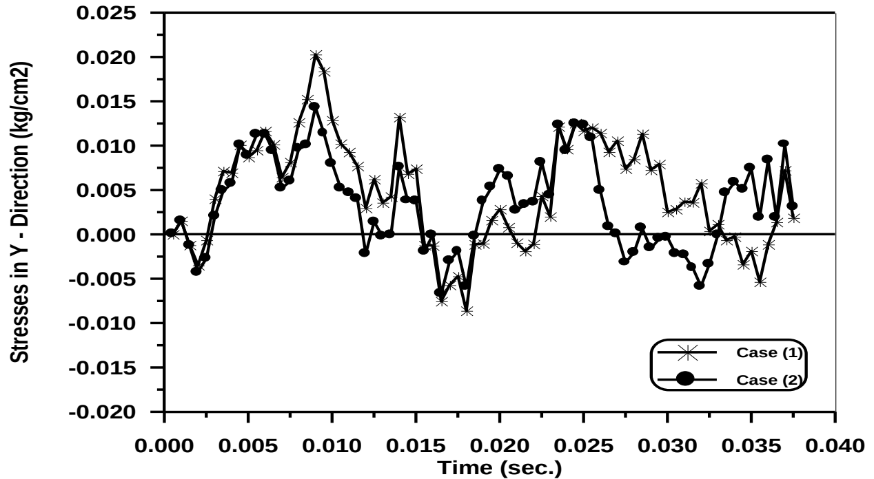
Figure (5-37) Time – Stresses in Y - Direction Response of The Circular Arch at Gauss point (3).
