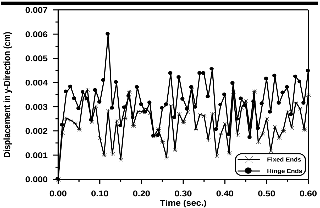
Figure (5-67) Time – Displacement in Y - Direction Response at ( \alpha=50^\circ ) with Various Boundary Condition.
