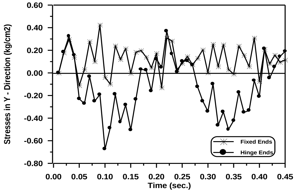
Figure (5-77) Time – Stresses in Y - Direction Response at Gauss Point (25 or 26) With Various Boundary Condition.
