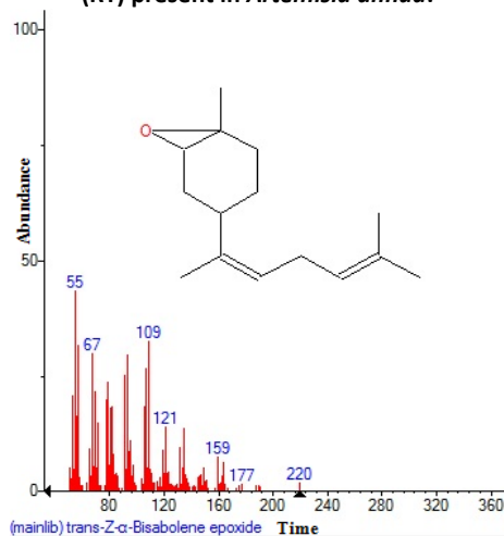
Figure 24. Structure of Trans-Z- \alpha -Bisabolene epoxide with 9.026 (RT) present in Artemisia annua .
