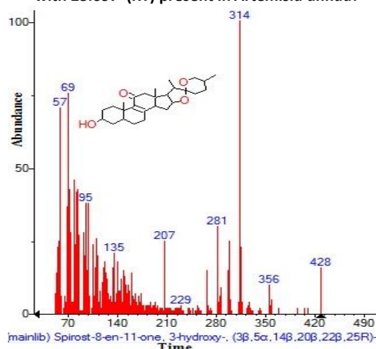
Figure 48. Structure of Spirost-8-en-11-one, 3-hydroxy-, (3β,5α,14β,20β,22β,25R) with 26.289 (RT) present in Artemisia annua .
