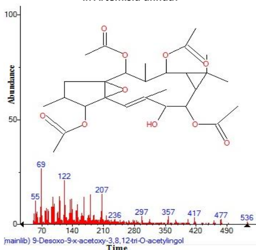
Figure 45. Structure of 9-Desoxo-9-x-acetoxy-3,8,12-tri-O-acetylingol with 21.649 (RT) present in Artemisia annua .
