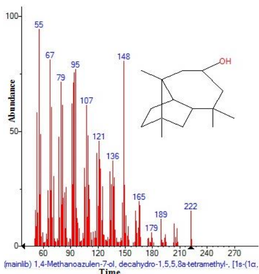
Figure 20. Structure of 1,4-Methanoazulen-7-ol, decahydro-1,5,5,8a-tetramethyl-, [1s-(1 \alpha ,3a)] with 7.527 (RT) present in Artemisia annua .
