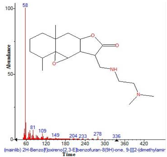
Figure 11. Structure of 2H-Benzo[f]oxireno[2,3-E]benzofuran-8(9H)-one, 9-[[[2-(dimethylamir with 4.672 (RT) present in Artemisia annua .
