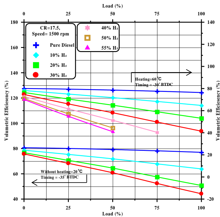
Fig 7 Variation of Volumetric Efficiency with Load for Different Hydrogen Blending Ratios With and Without Heating
