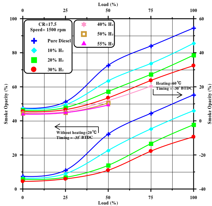
Fig 16 Variation of smoke opacity with Load for Different Hydrogen Blending Ratios With and Without Heating
