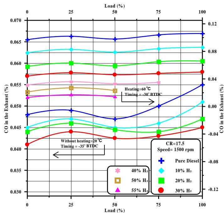
Fig 12 Variation of Carbon Monoxide with Load for Different Hydrogen Blending Ratios With and Without Heating
