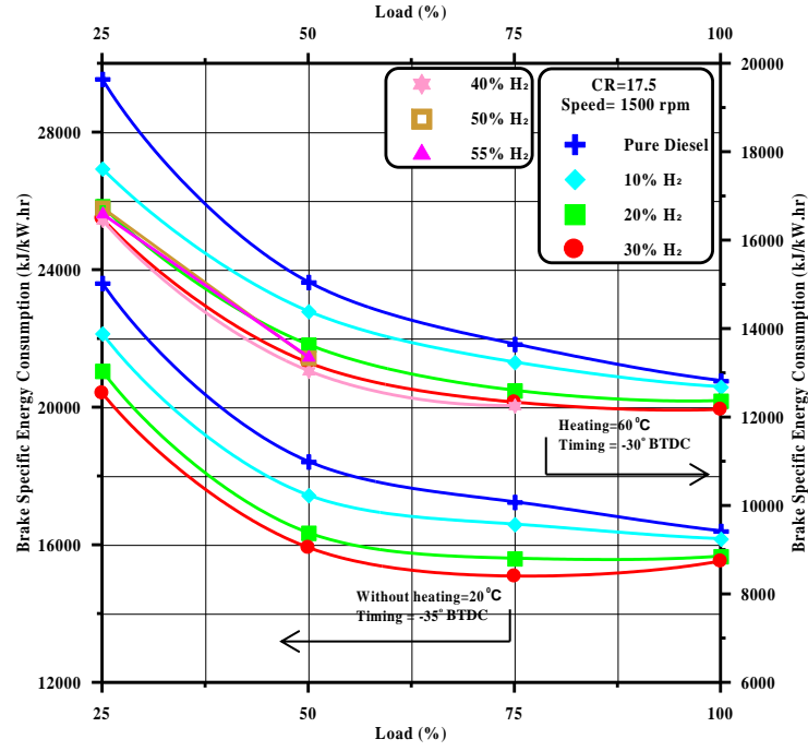
Fig 6 Variation of brake specific Energy consumption with Load for Different Hydrogen Blending Ratios With and Without Heating
