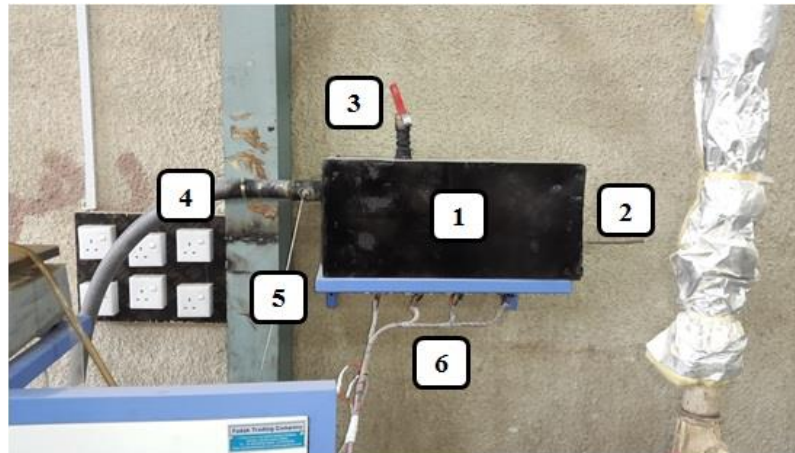
Plate 2 Air Heating System
