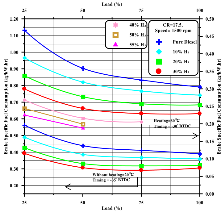
Fig 5 Variation of brake specific fuel consumption with Load for Different Hydrogen Blending Ratios With and Without Heating
