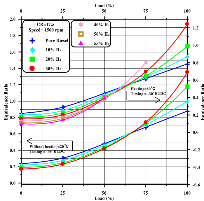
Fig. 8 Variation of Equivalence Ratio with Load for Different Hydrogen Blending Ratios With and Without Heating
