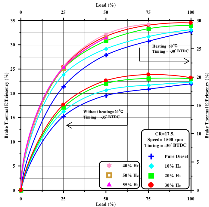
Fig 4 Variation of Brake Thermal Efficiency with Load for Different Hydrogen Blending Ratios With and Without Heating
