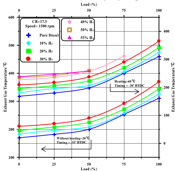
Fig 11 Variation of Exhaust Gas Temperature with Load for Different Hydrogen Blending Ratios With and Without Heating
