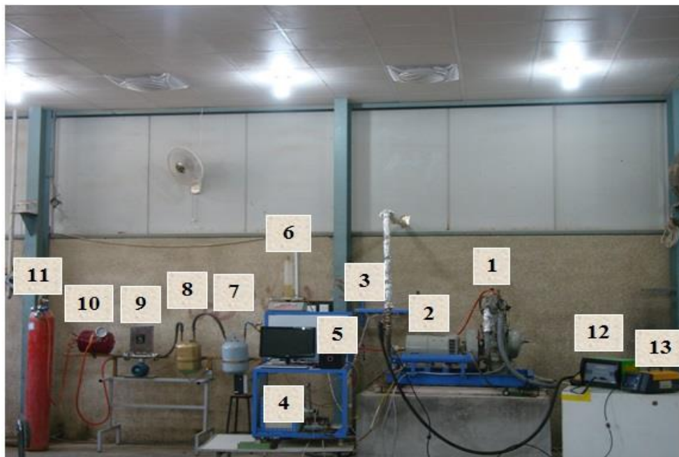
Plate 1 Front View of the Experimental Set Up
