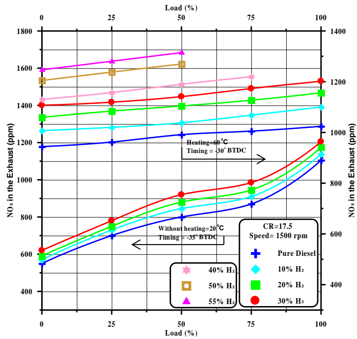
Fig 15 Variation of NO x with Load for Different Hydrogen Blending Ratios With and Without Heating
