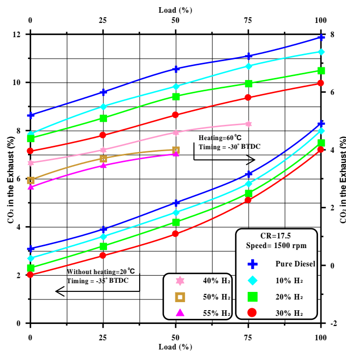
Fig 13 Variation of Carbon Dioxide with Load for Different Hydrogen Blending Ratios With and Without Heating
