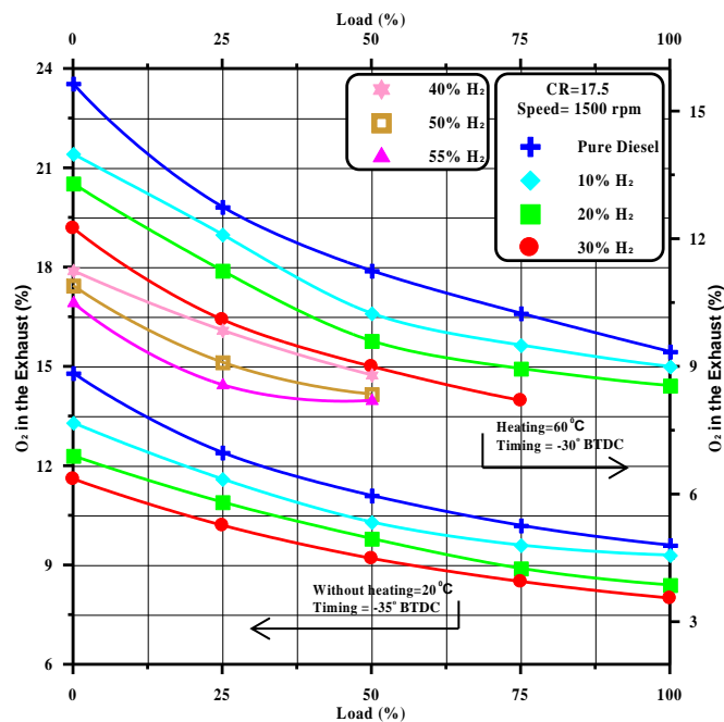
Fig 17 Variation of O 2 with Load for Different Hydrogen Blending Ratios With and Without Heating
