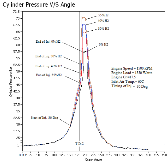
Fig 10 Variation of In-cylinder pressure with Crank angle for Different Hydrogen Blending Ratios.
