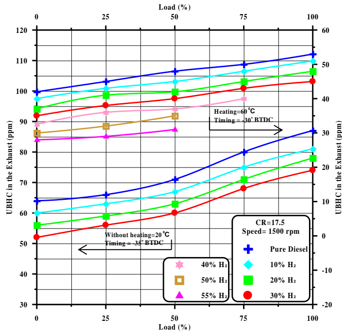
Fig 14 Variation of UBHC with Load for Different Hydrogen Blending Ratios With and Without Heating
