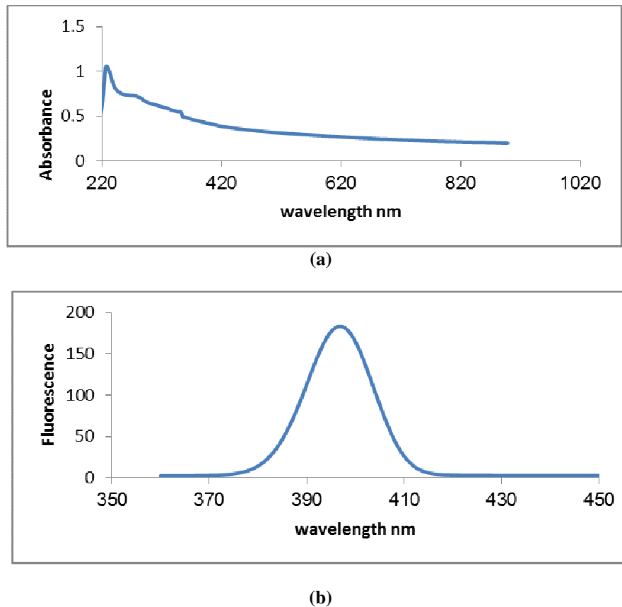
Fig. 5: Absorbance (a) and Fluorescence (b) spectra of MgO NPs prepared chemical method
