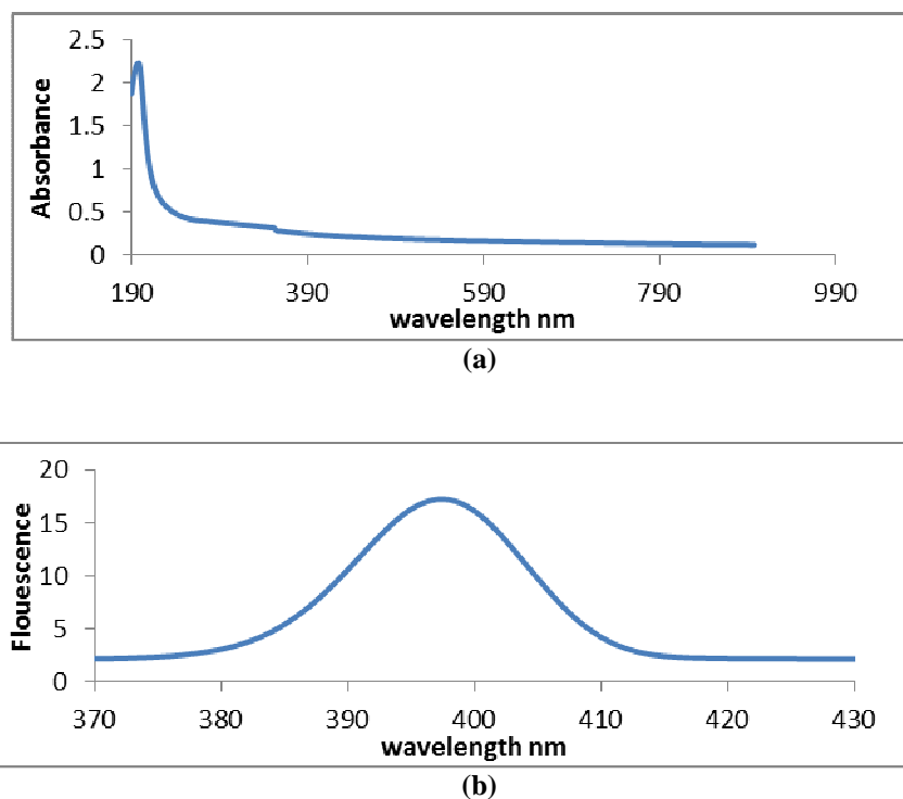
Fig. 4: Absorbance (a) and Fluorescence (b) spectra of MgO NPs prepared by PLAL method
