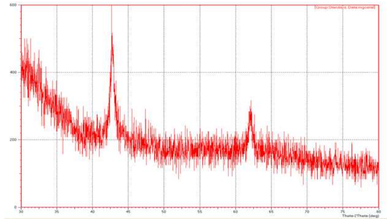
Fig. 1.a XRD of MgO NPs prepared by PLAL method
