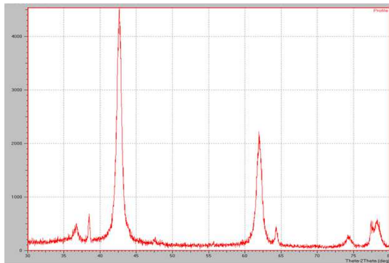
Fig. 1.b: XRD of MgO NPs prepared by chemical method
