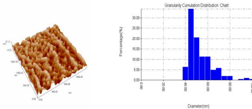
Fig. 3.a: AFM of MgO NPs prepared by PLAL method
