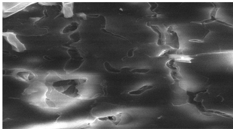
Fig. 2.a: SEM of MgO NPs prepared by PLAL method
