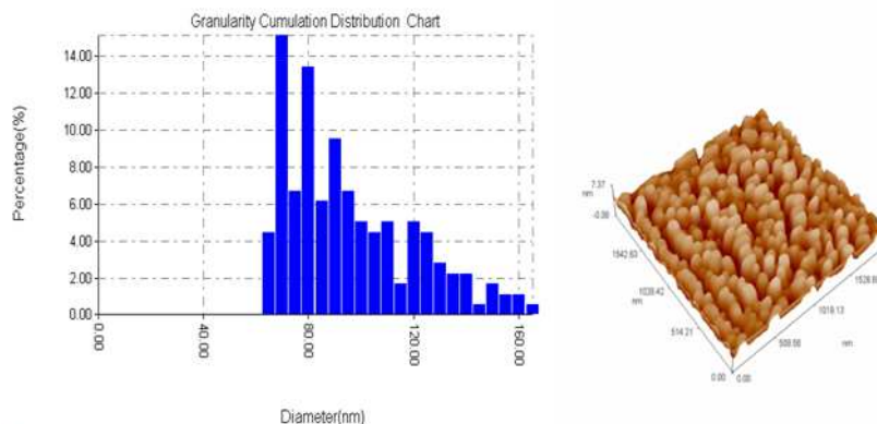
Fig. 3.b: AFM of MgO NPs prepared by chemical method
