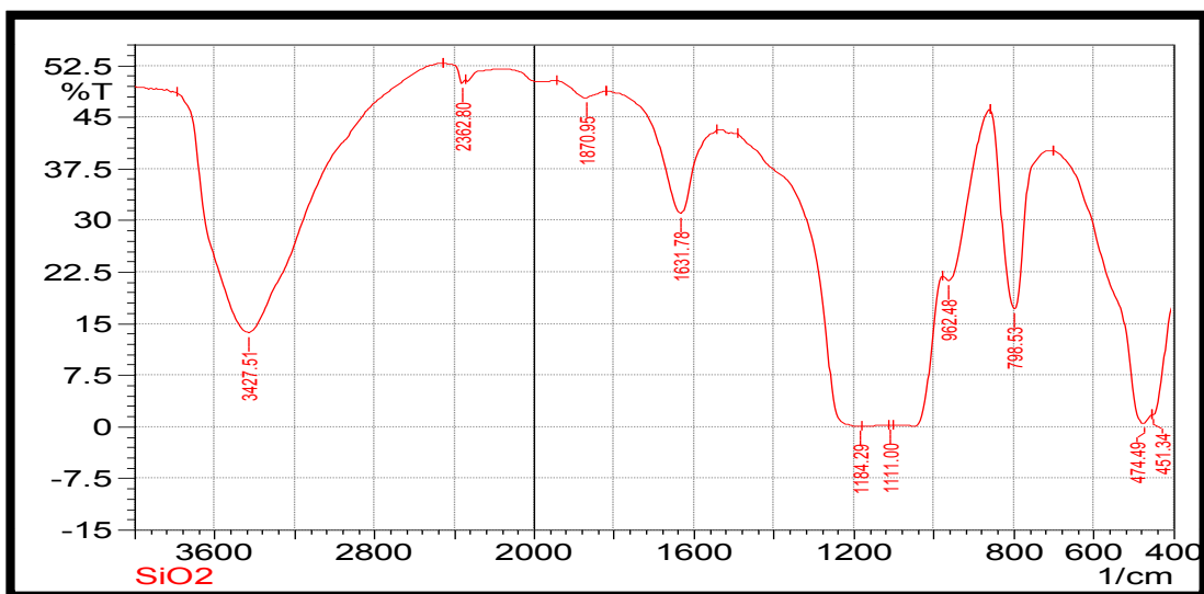
Fig.6a. FTIR spectrum of precipitated SiO 2
