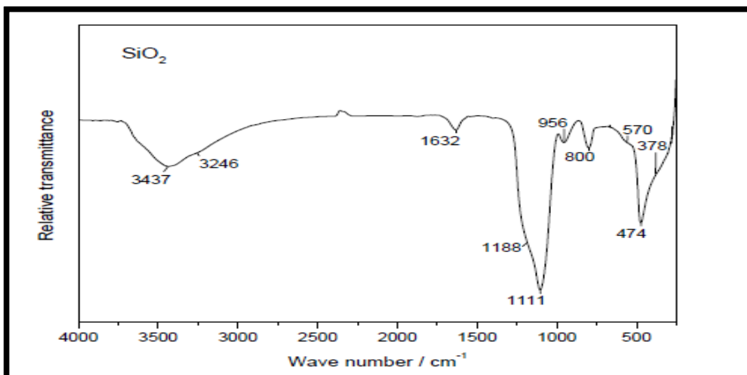
Fig. 6b. FTIR spectrum of precipitated SiO 2 [13]
