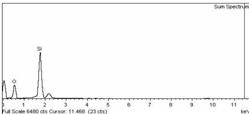
Fig. 4. EDS spectrum of precipitated SiO 2
