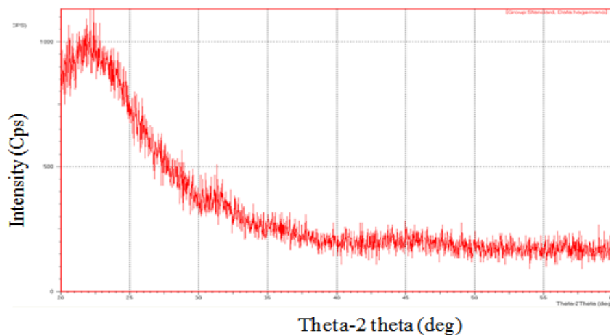
Fig.(5b). X-Ray Diffraction Analysis of precipitated SiO 2 (after extra washing)
