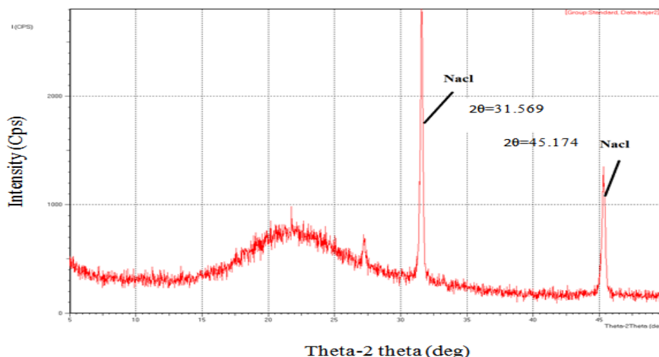
Fig.(5a). X-Ray Diffraction Analysis of precipitated SiO 2 (before washing)
