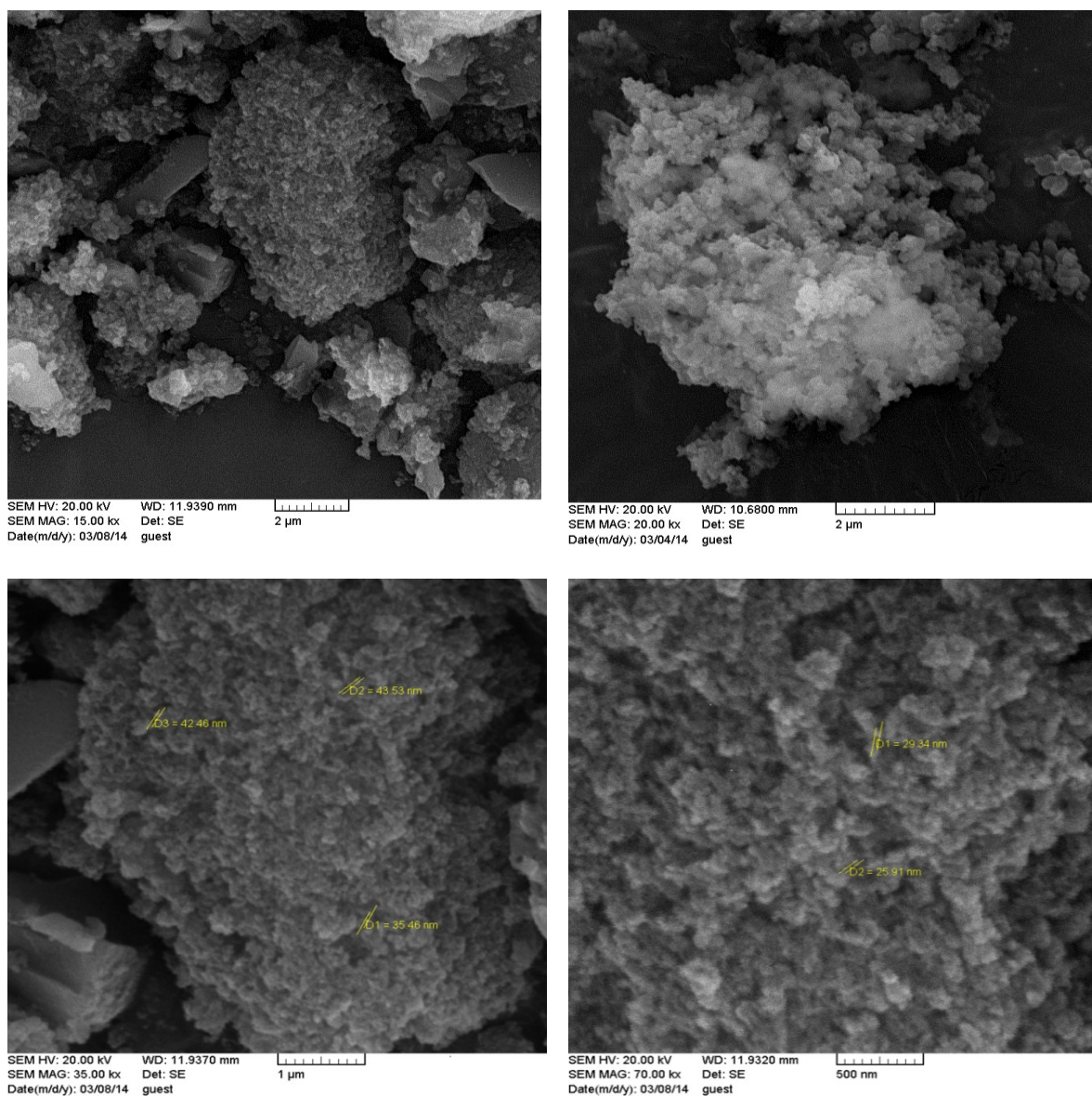
Fig. 2. SEM micrographs images of precipitated SiO 2
