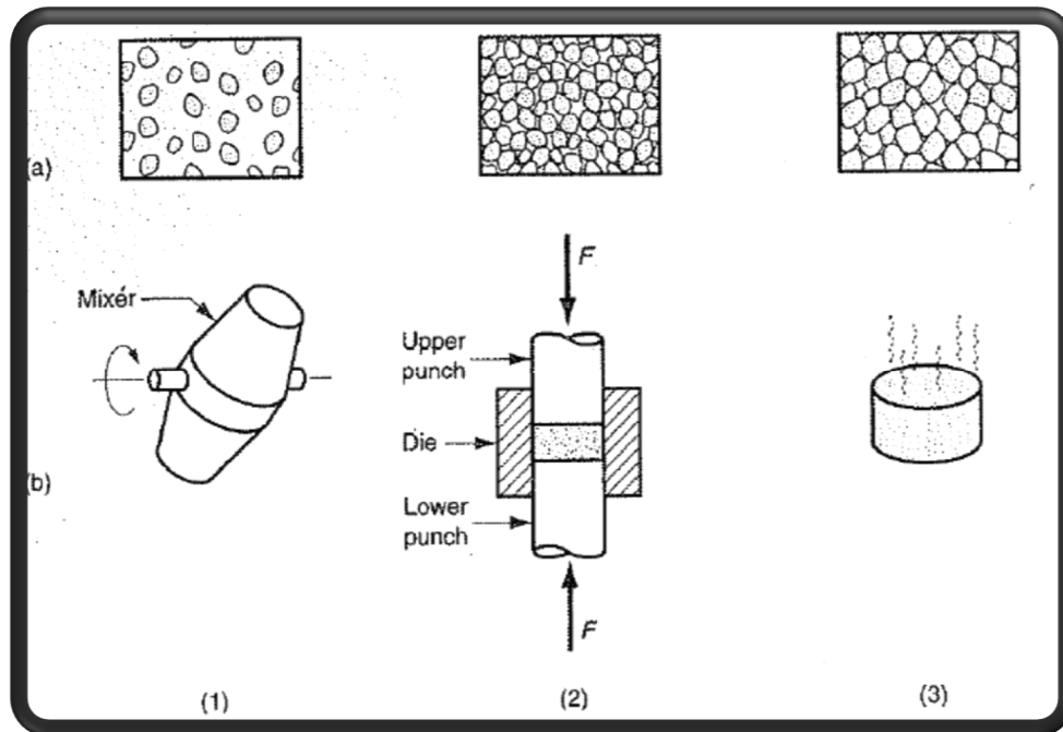
Fig (2): The conventional powder metallurgy production sequence: (1) blending, (2) compacting, (3) sintering [Shashank 2014]
