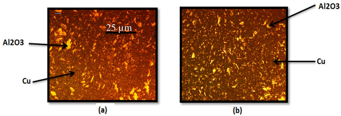
Fig (4): Microstructure of the sample prepared using a compacting pressure of 550 MPa (400X * magnification), (a) H 1 , (b) H 5
