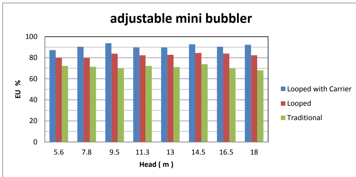
Figure 4 : Pressure – Field Uniformity Relationship for Adjustable Mini Bubbler flow Dripper
