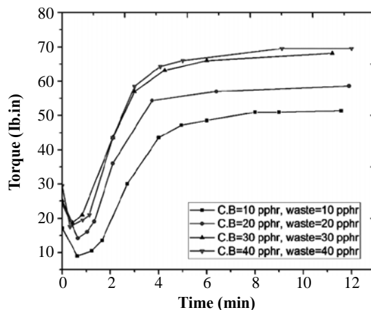
Fig. 3: Variations in rheograph of SBR compounds with the loading level of mix C.B. and waste at T = 175^{\circ}\text{C}
