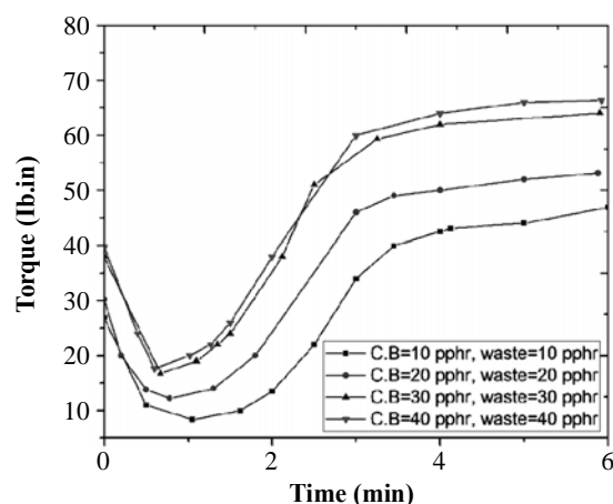
Fig. 4: Variations in rheograph of SBR compounds with the loading level of mix C.B. and waste at T = 185^{\circ}\text{C}
