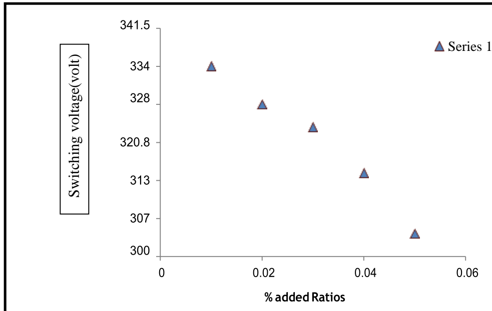
Fig (8): shows the operating voltage as a function of rates SnO 2 added to the polymer
