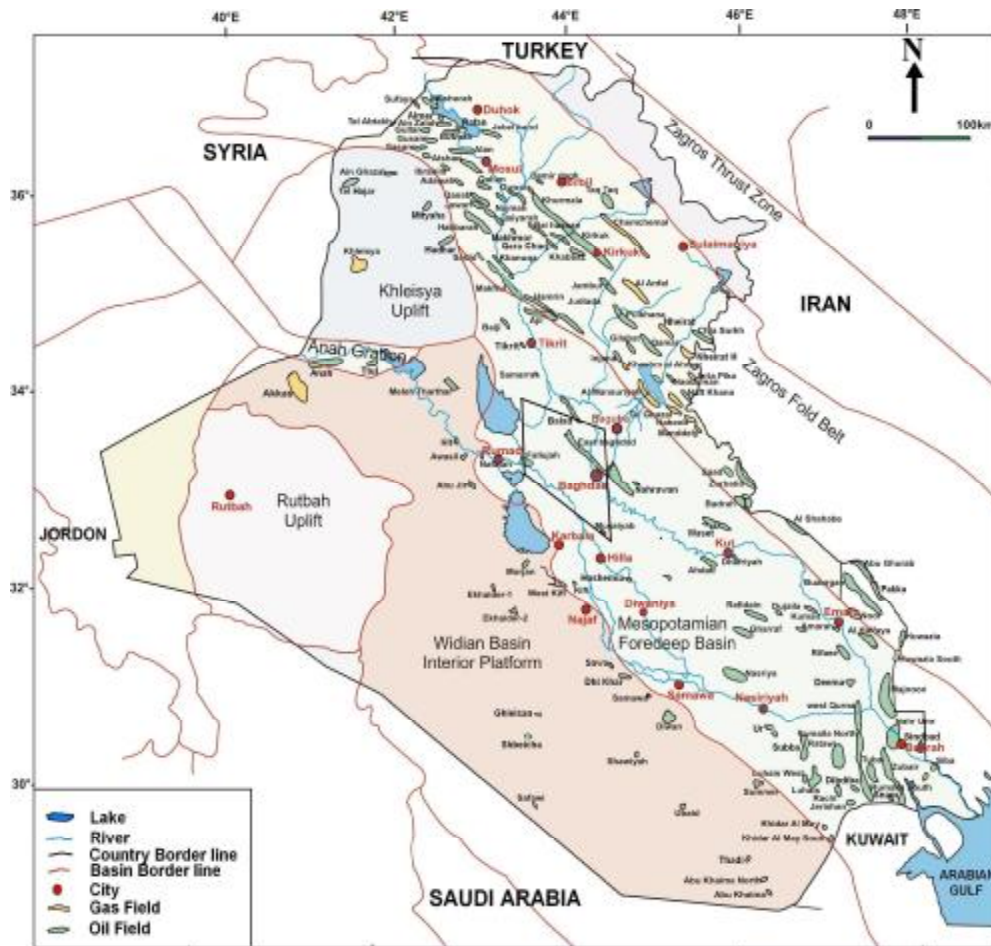
Figure (2). Location map of Iraq showing a northeast Arabian Peninsula of the region Iraq with locations of basins and oil fields [Iraqi Geological Survey and Mining, 2010]
