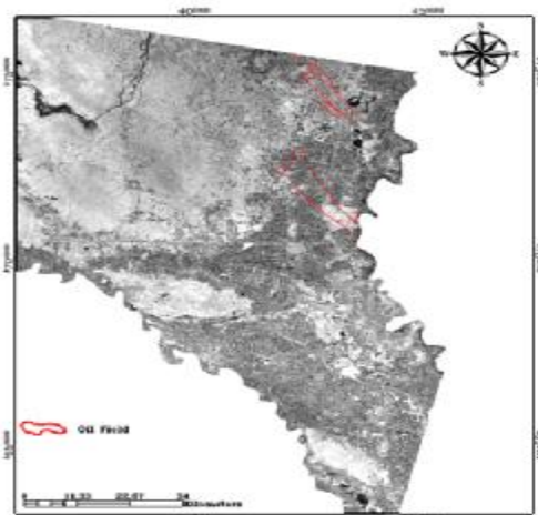
Figure (4-b) Gray Scale Thermal High Band (ETM+).
