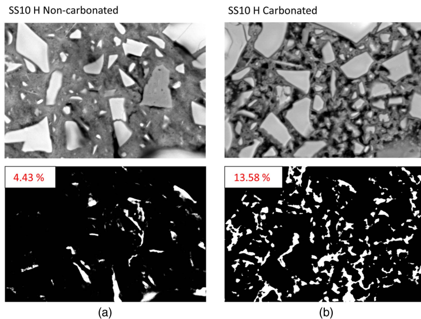
Fig. 15. Porosity percentage segmentation using Image J-software for SEM images of Mix SS10 H after 24 months of exposure to laboratory environment ( 20^{\circ}\text{C} \pm 2^{\circ}\text{C} and 40\% \pm 7\% RH) showing difference in porosity between (a) noncarbonated; and (b) carbonated regions. (Reprinted with permission from Humad 2019.)
