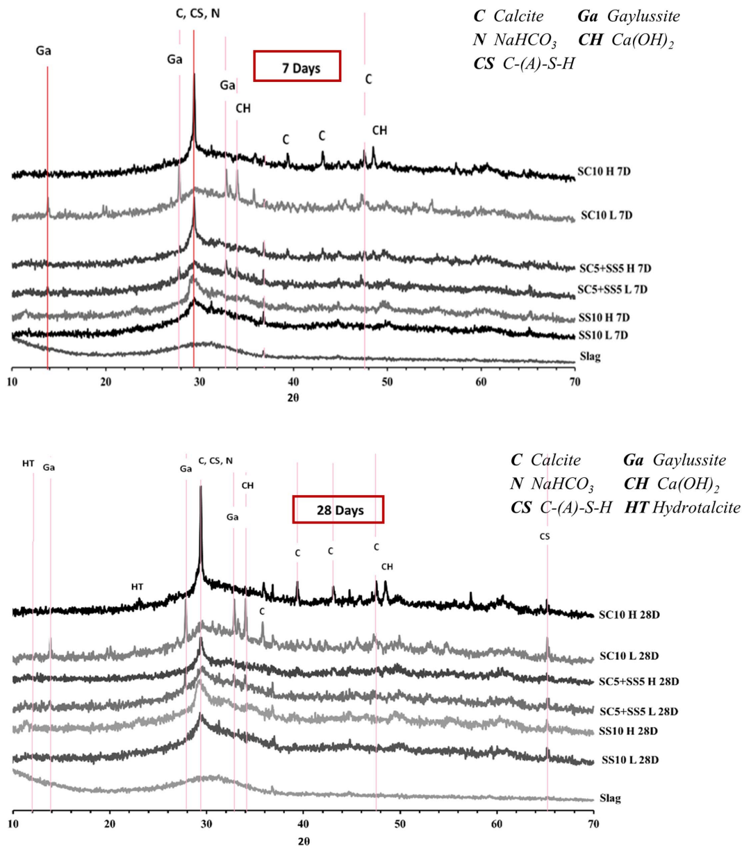
Fig. 5. XRD results for 7- and 28-day cured AAS pastes. Suffixes L7D and L28D denote 7 and 28 days of lab curing, respectively, whereas H7D and H28D denote 7 and 28 days of heat curing, respectively.
