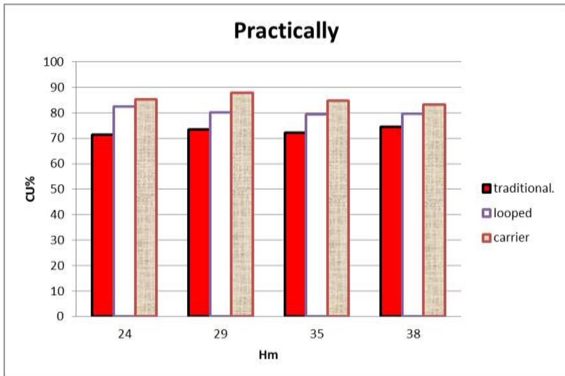
Fig. 3 The average means performance of the uniformity coefficients in the cases practically
