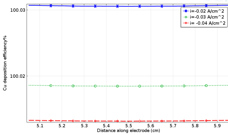
Fig. 6(b). Copper deposition efficiency versus distance along section B at m=0.5 kg/s.
