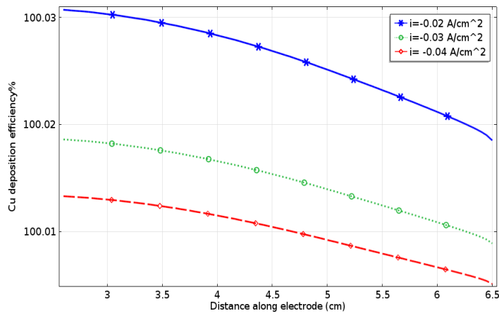
Fig. 6(e). Copper deposition efficiency versus distance along section R at m=0.5 kg/s.
