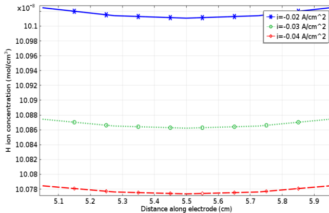
Fig. 5(a). H ion concentration distribution along section B at m=0.1 kg/s.
