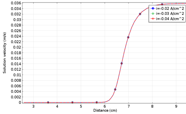
Fig. 4(b). Distribution of velocity along the cut line (shown in Fig. 4(a)) starting from B inside the trench towards the solution outside at m=0.5 kg/s.
