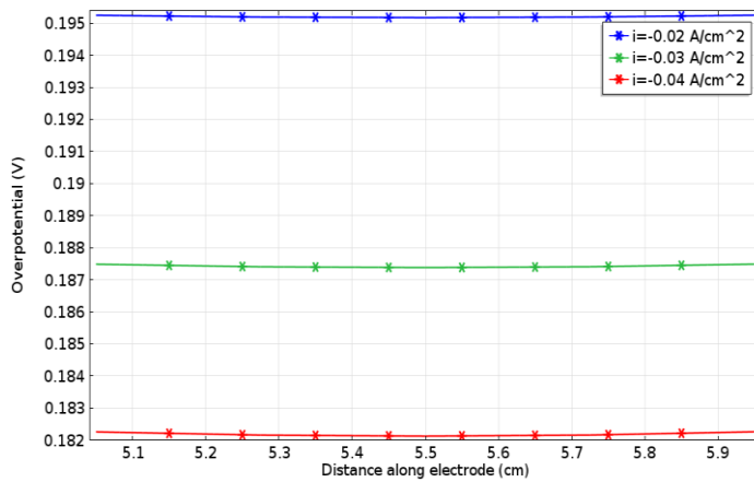
Fig. 7. Hydrogen evolution overpotential along the working electrode, section B at m = 0.1 kg/s.
