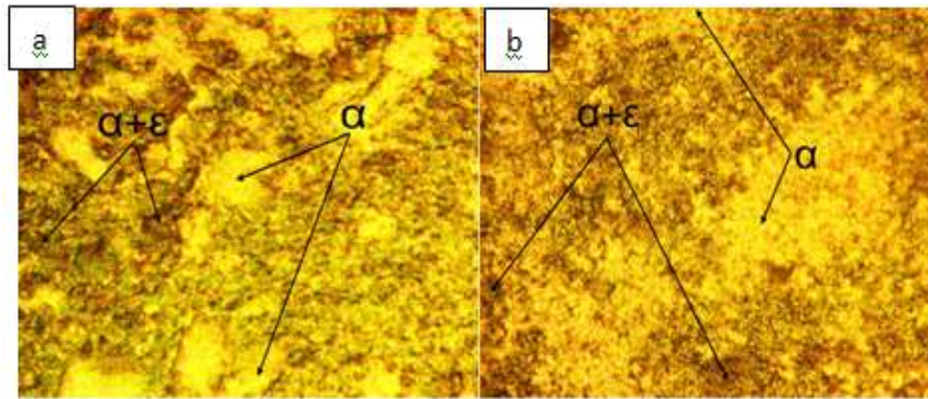
Fig. 5: Optical Microscope Image (600 X): (a) Sample Prepared at (450 °C , 60 min. , 40 MPa and 20 wt. % NaCl), (b) Sample Prepared at (650 °C , 180 min. , 80 MPa and 40 wt. % NaCl)
