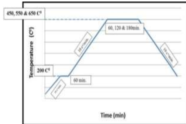
Fig. 1: The Sintering Program of the Green Samples
