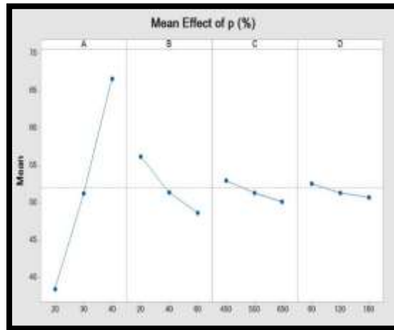
Fig. 7: Main Effect Plot for Means of The Porosity
