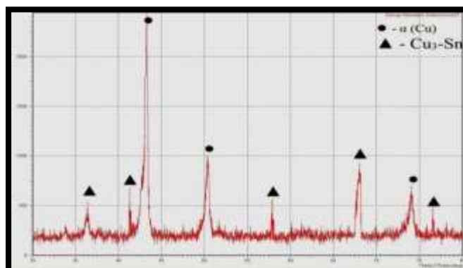
Fig. 4: XRD Pattern of Sample Prepared With 40 wt. % NaCl , 80 MPa Compact Pressure, 650 °C Sintering Temperature and 180 Min. Sintering Time
