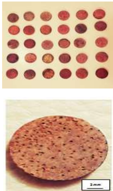
Fig. 2: The samples after removing NaCl
