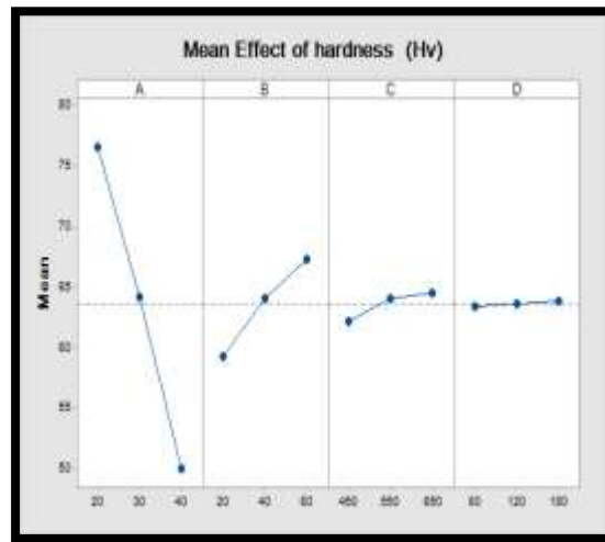
Fig. 9: Main Effect Plot for Means of Hv
