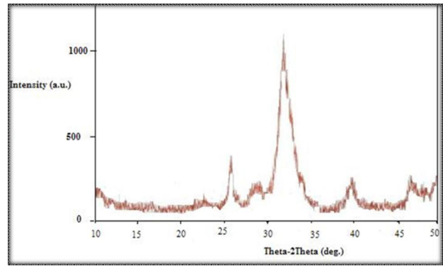
Fig. 2 XRD patterns of fish bones-HA powder.
