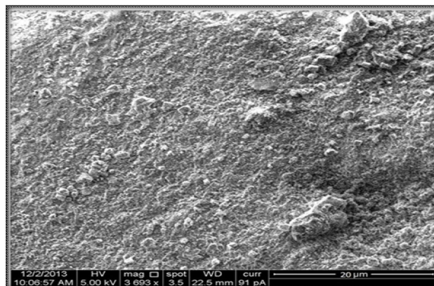
Fig. 10 SEM image of 15% micro HA-resin composite
