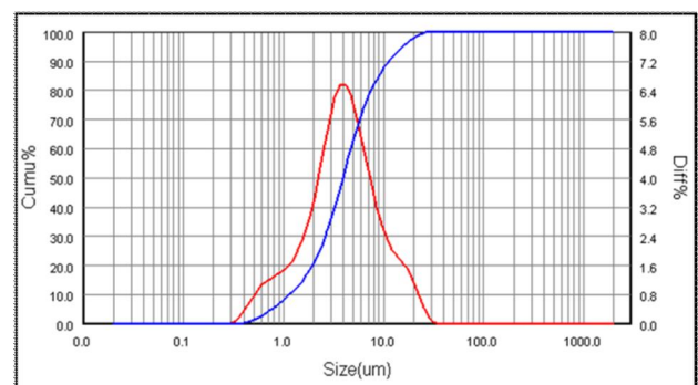
Fig. 4 Particle size analysis of fish bones HA-powder
