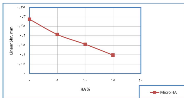
Fig. 8 Linear shrinkage of micro HA-resin composite
