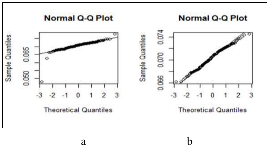
Figure (6): Q-Q Norm for Data Samples (R.E). (a- Before and b- After) Background
