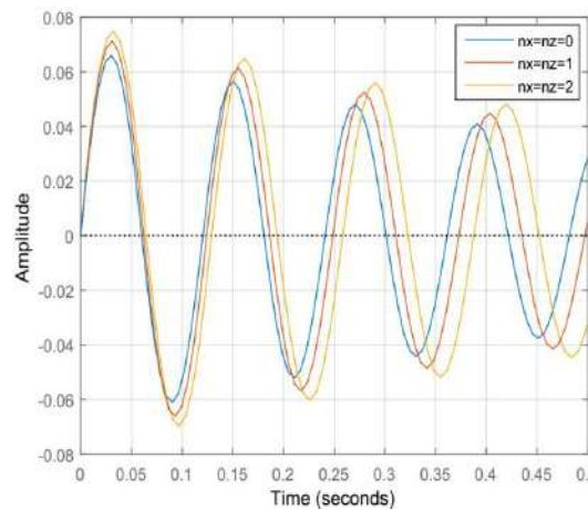
Figure 10. Zoom Transient response of cantilever FGM variable value of law power index
