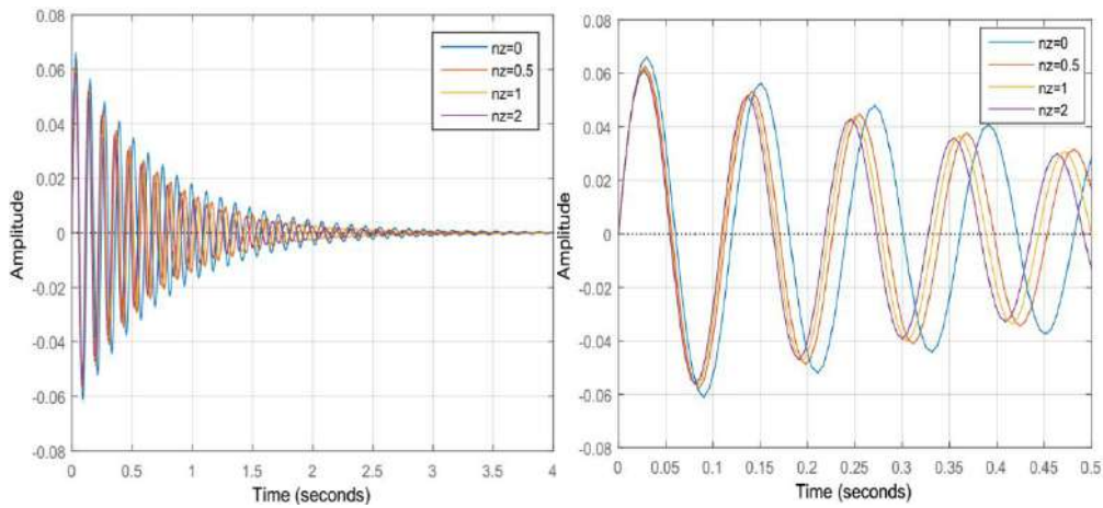
Figure 14. a) Transient response of cantilever FGM beam with n_x=0 , b) Zoom of the transient response.
