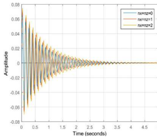
Figure 9. Transient response of cantilever FGM beam with variable value of law power index
