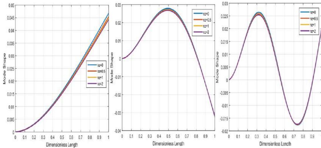
Figure 7. The first three modes of cantilever FGMT beam with law power index ( n_x=0 ), b=.05m , h=0.005m , h/l=0.1
