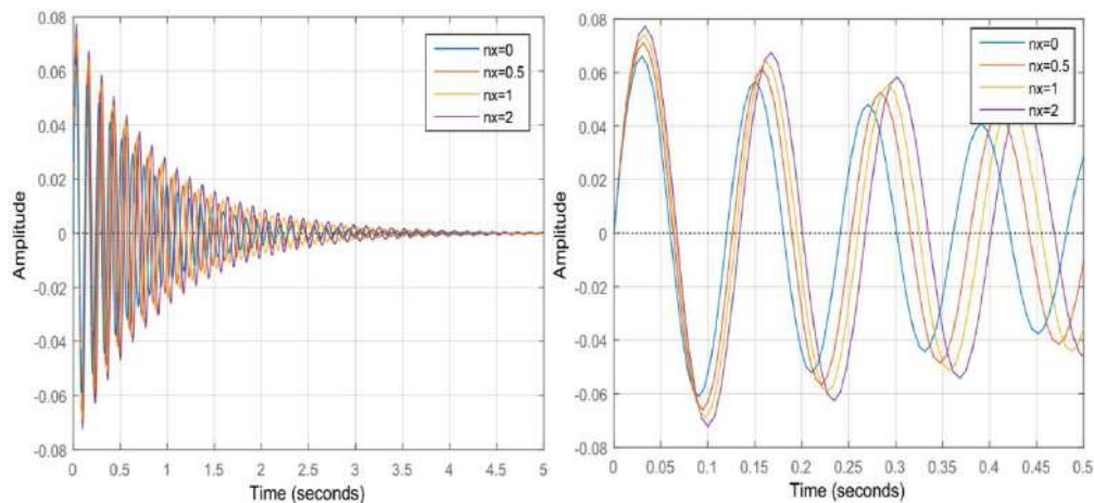
Figure 13. a) Transient response of cantilever FGM beam with nz=0 , b) Zoom of the transient response.
