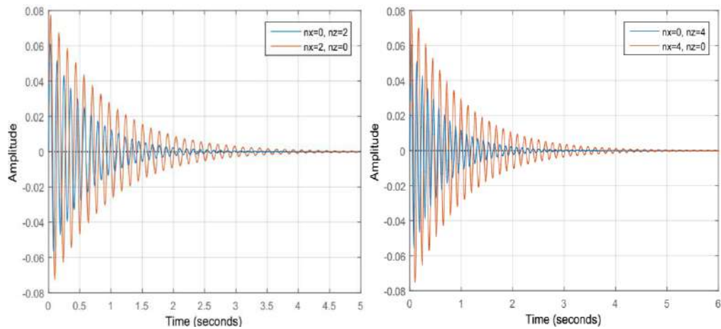
Figure 12. Transient response of cantilever FGM beam with variable value of law power index
