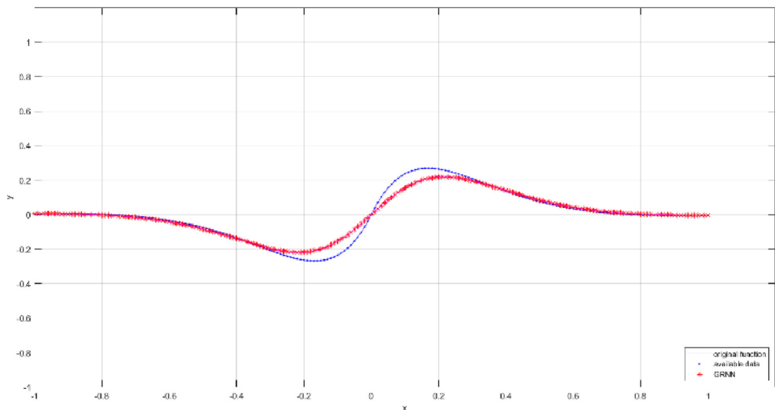
Fig. 2. Approximation of y = \sin(4x)\exp(-|5x|) by GRNN.
