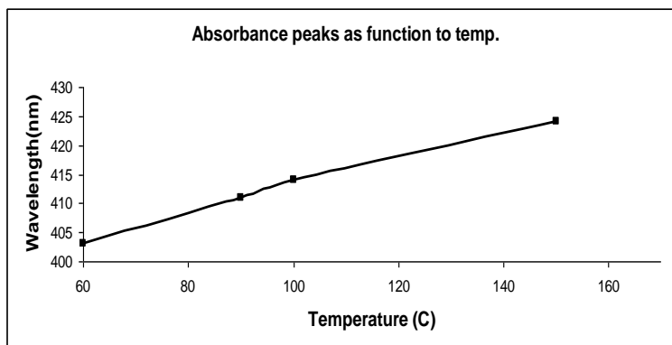
Figure 13. absorbance peak of Xerogel for transition ( v_3 ) as function of temperature
