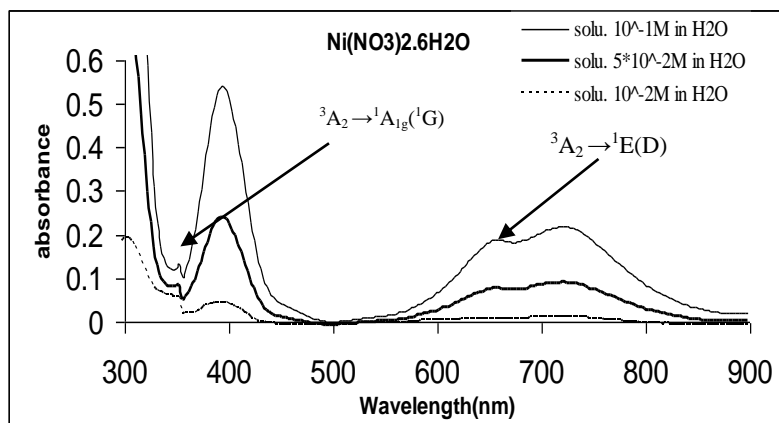
Figure (5) The absorption spectra of Ni(NO_3)_2 \cdot 6H_2O in water
