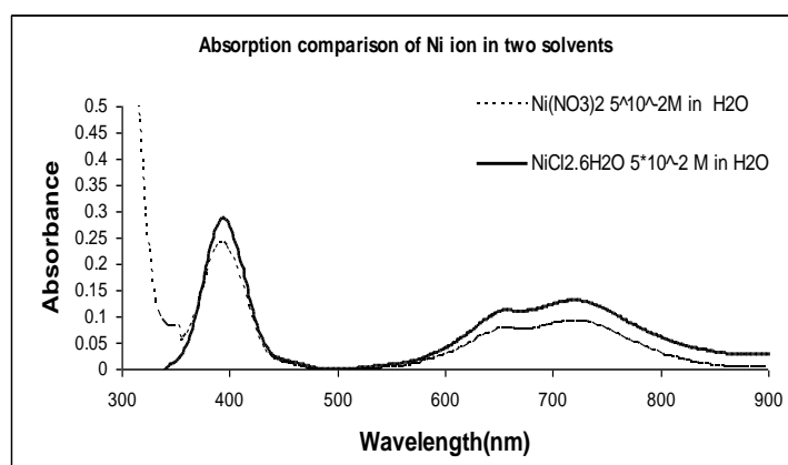
Figure (6) The absorption spectra of Ni(NO_3)_2 \cdot 6H_2O and NiCl_2 \cdot 6H_2O in water
