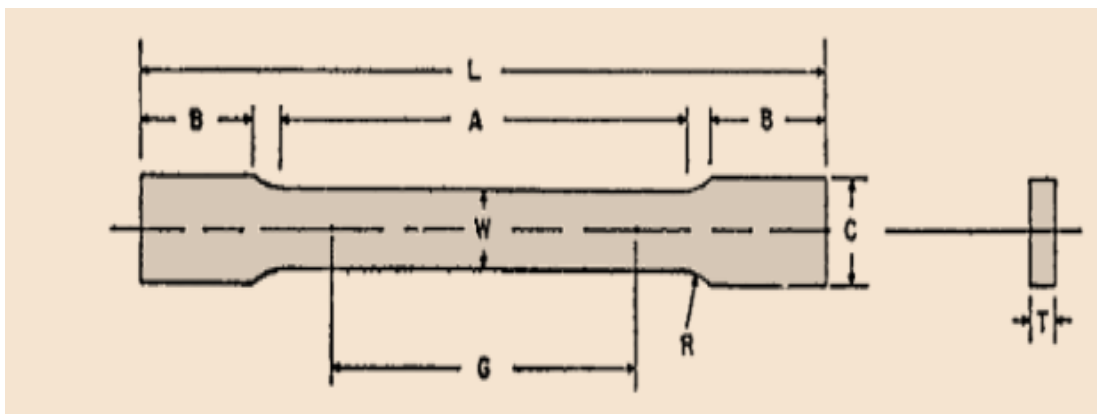
Figure 2 ASTM Sub-Size Sample for Tensile Test. Gage length (G) : ( 0.25±0.1) mm; Width (W) : ( 60.1± 0.05) mm; Thickness (T): 6mm; Radius of fillet, min (R): 6mm; Length overall length, min. (L): 110mm, Length , min. (A): 35 mm; Length of grip section, min. (B): 30mm; Width of grip Section, approximate(C): 20mm.[15]
