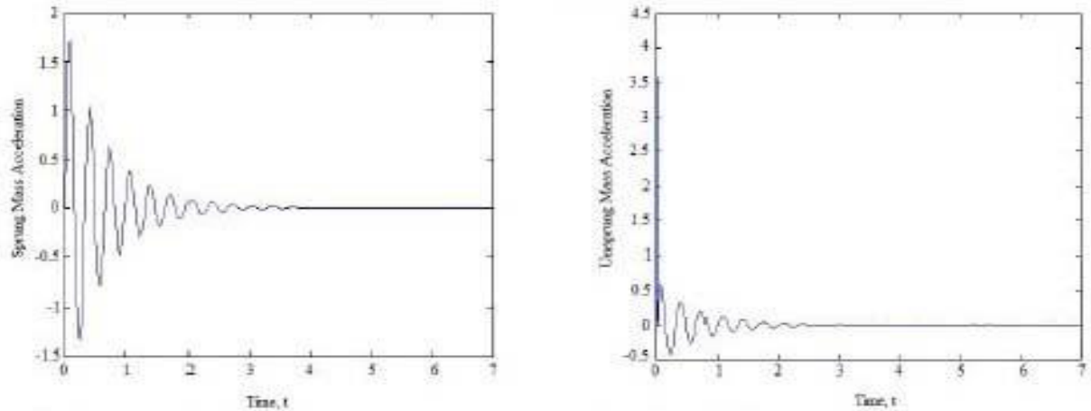
Figure. (14-b) Response of unsprung mass of suspension system [19]
