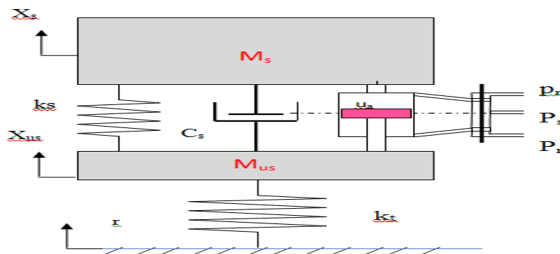
Figure. (7) Schematic of Active suspension system [5]
