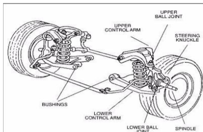
Figure. (3) Double wishbone suspension system [3]
